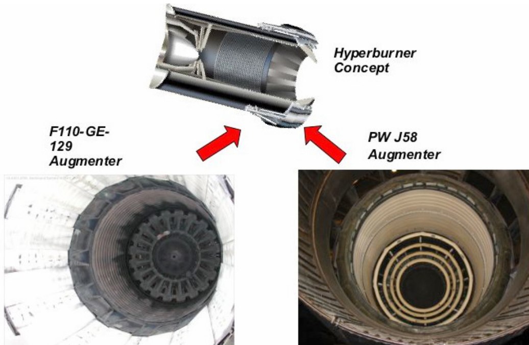
Figure 5.—Current RTA Hyperburner compared with F110 and J58 augmentor configurations.
