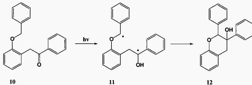
Scheme 3. Simplified representation of the photocyclization of \alpha -( o -(benzyloxyphenyl)acetophenone via the 1,6-biradical intermediate [27].
