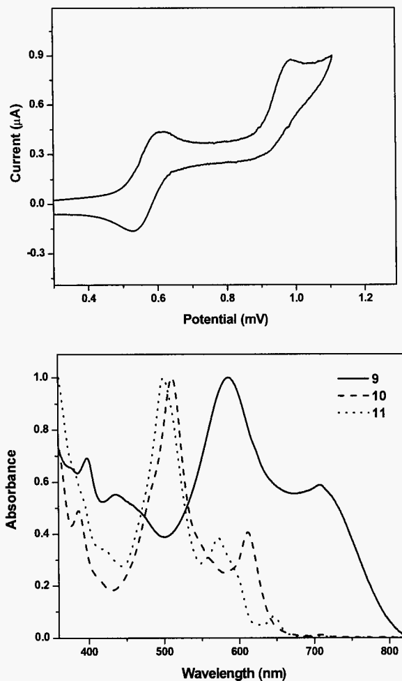
Fig. 4. (top) Cyclic voltammogram of CN-diox ( 9 ). The experiment was performed in benzonitrile (0.1 M TBAPF 6 ) at a scan rate of 50 mV/s. (bottom) Electronic spectra of the electrochemically generated radical cation of CN-diox ( 9 , solid line), Alkyl-diox ( 10 , dashed line), and diox ( 11 , dotted line) in benzonitrile.
