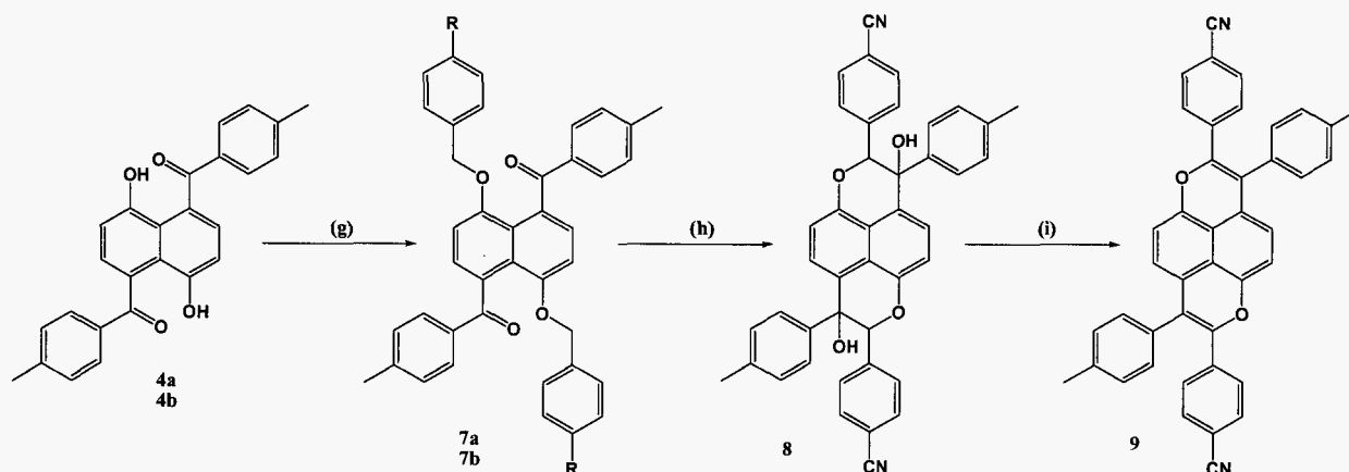
Scheme 2. Representation of the synthesis of 5,10-di(4-cyanophenyl)-4,9-di(4-methylphenyl)-1,6-dioxapyrene ( 9 or CN-diox ) from 1,5-dihydroxy-4,8-di(4-methylbenzoyl)naphthalene ( 4 ).
