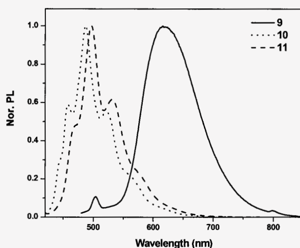
Fig. 6. Normalized photoluminescence spectra of CN-diox ( 9 , solid line), Alkyl-diox ( 10 , dashed line), and Diox ( 11 , dotted line) in THF at 23 °C. The excitation wavelengths were 440 nm, 370 nm, and 360 nm, respectively.
