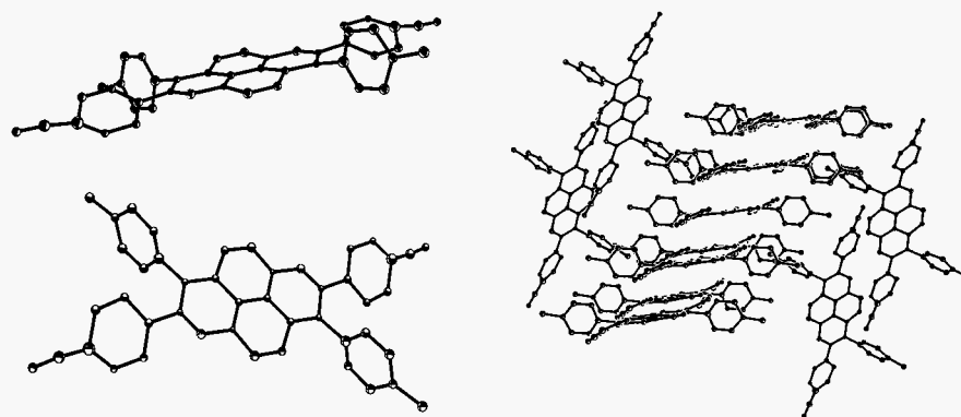
Fig. 3. X-Ray structures for CN-diox ( 9 ).
