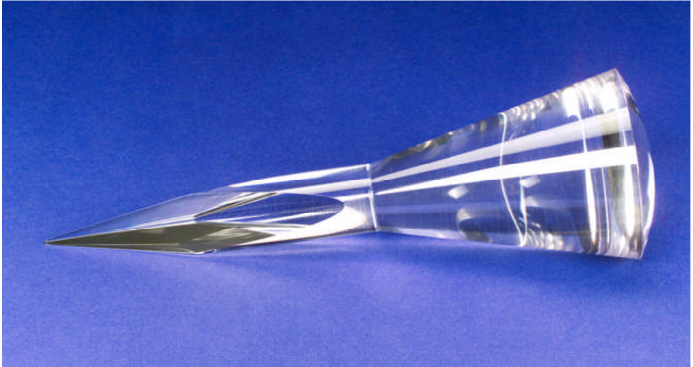
Prototype refractive secondary concentrator made of single-crystal sapphire.
