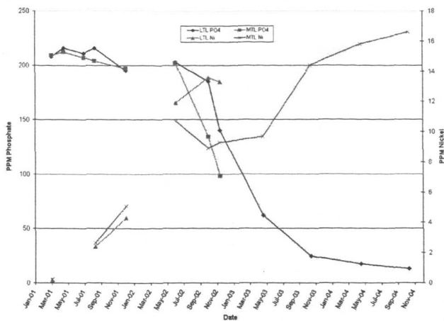
Figure 3. Phosphate and dissolved nickel trends showing nickel concentration leveling off as phosphate concentration drops (forming nickel phosphate)
