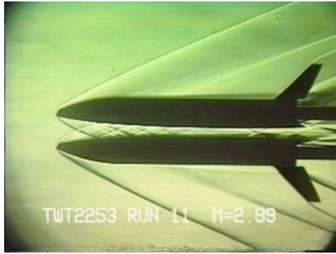
(a) \bar{x}/l_{ref} = 0.0, \bar{z}/l_{ref} = 0.0, \bar{\beta} = 0
