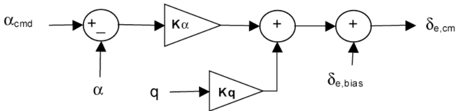
Figure 21. Feedback control system implemented in ConSep.
