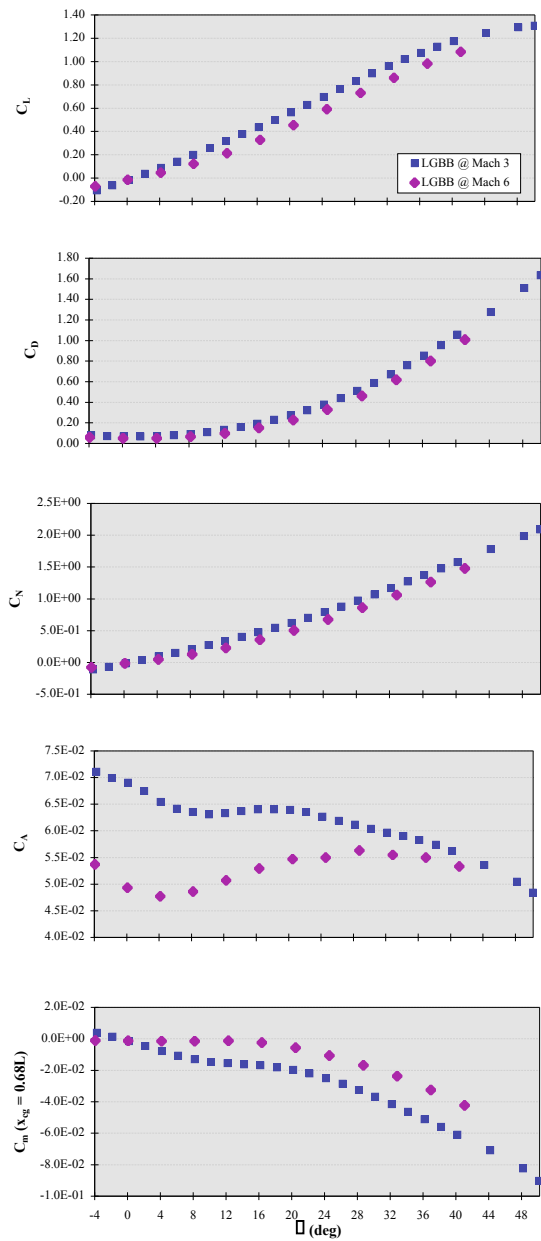
Figure 10: Variation of Isolated LGGB lift, drag, normal and axial force, and pitching moment coefficients with AoA at Mach 3 and 6.
