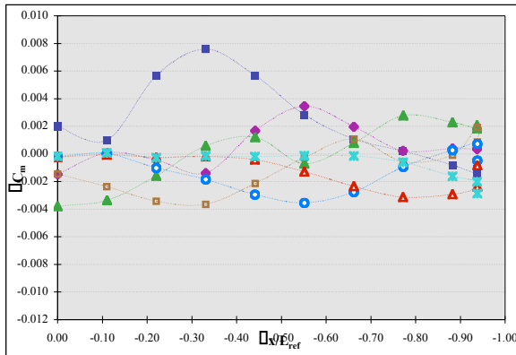
Vehicle 1 (Booster) @ \alpha = 0 degrees
