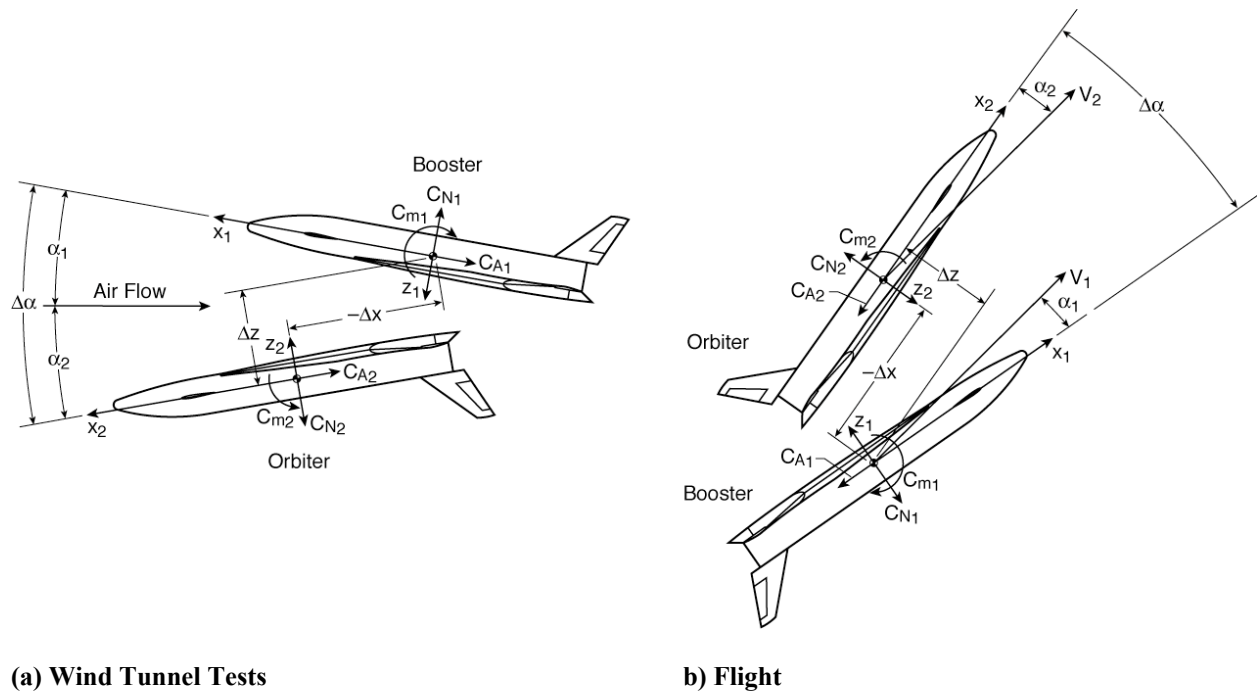
Figure 5. Relative locations of booster and orbiter in proximity.
