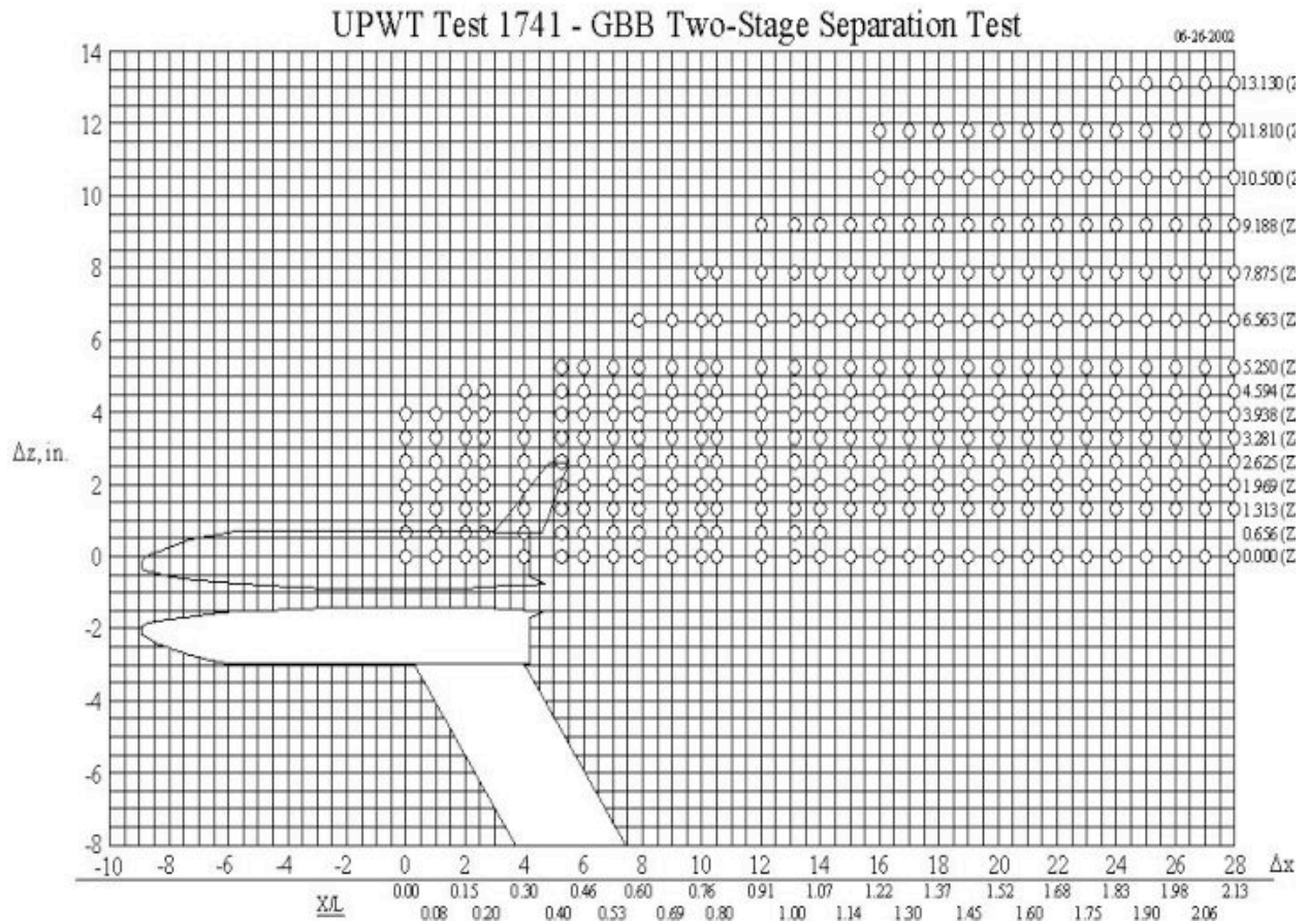
Figure 6. Schematic illustration of LGBB-Beimese UPWT test matrix at Mach 3.
