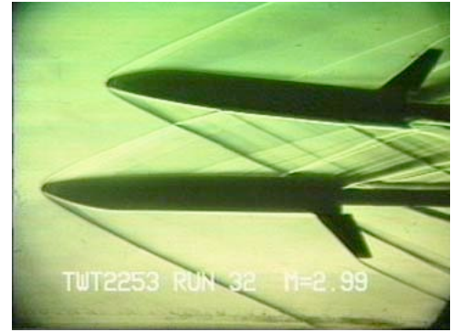
(b) \bar{x}/l_{ref} = 0.2, \bar{z}/l_{ref} = 0.16, \bar{\beta} = 5
