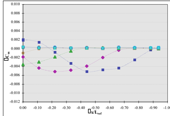
Vehicle 2 (Orbiter) @ \alpha = 0 degrees
