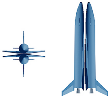
Figure 3. Bimese version of the LGBB TSTO Vehicle.
