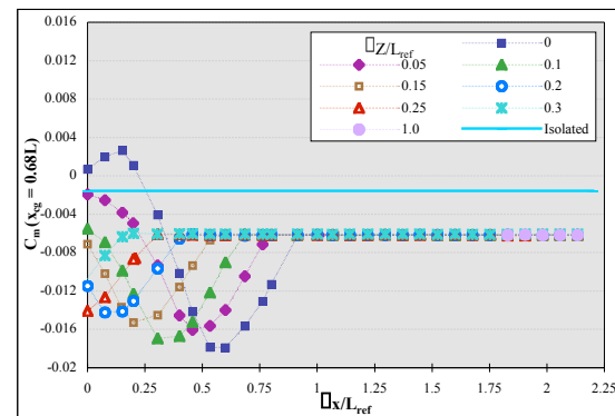
Figure 16: Variation of bimese-orbiter pitching moment coefficients with \bar{x}/L_{ref} and \bar{z}/L_{ref} at Mach 3 for \alpha = 0 , \beta = 0 degrees.
