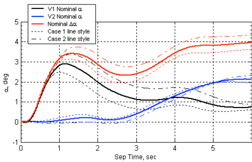
Figure 27. Effect of parametric variation in altitude.
