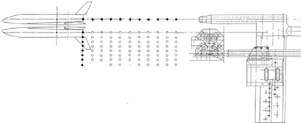
Figure 7. Schematic illustration of the LGBB-Beimese Mach 6 Tunnel test matrix.
