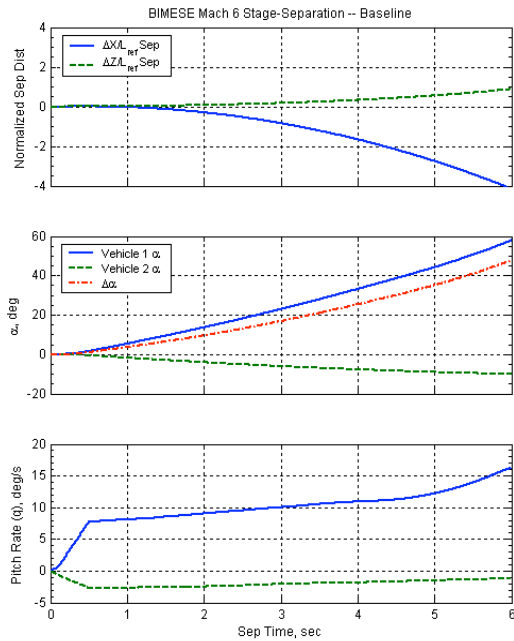
Figure 20. Mach 6 baseline separation.
