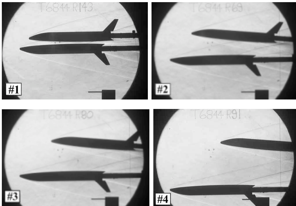
Figure 9. Schlieren Photographs of the LGBB-Bimese configuration in 20-Inch Mach 6 Tunnel.
