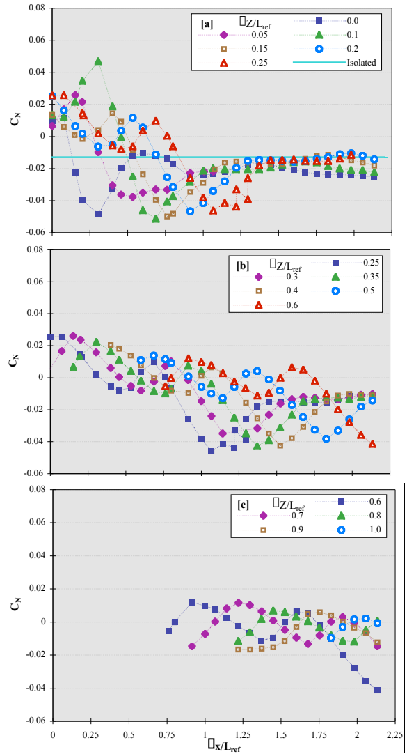
Figure 11: Variation of bimese-booster normal force coefficient with \square x/L_{ref} and \square z/L_{ref} at Mach 3 for \square = 0, \square = 0 degrees.
