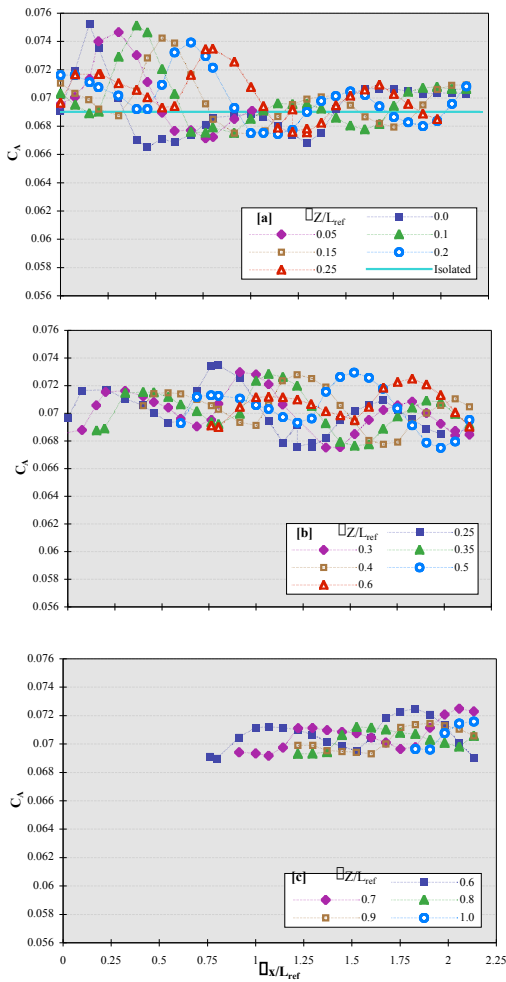
Figure 13: Variation of bimese-booster axial force coefficient with \bar{x}/L_{ref} and \bar{z}/L_{ref} at Mach 3 for \alpha = 0 , \beta = 0 degrees.
