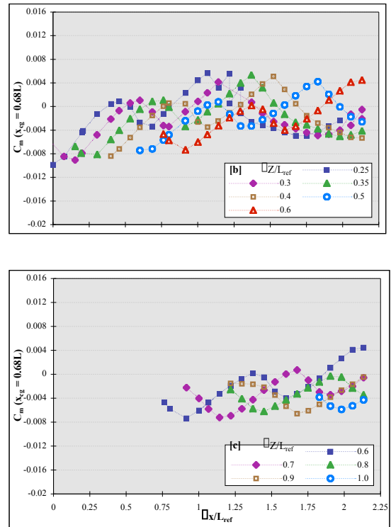
Figure 14: Variation of bimese-booster pitching moment coefficient with \bar{x}/L_{ref} and \bar{z}/L_{ref} at Mach 3 for \alpha = 0 , \beta = 0 degrees.
