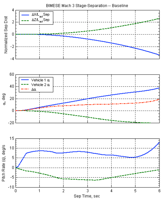
Figure 19. Mach 3 baseline separation.
