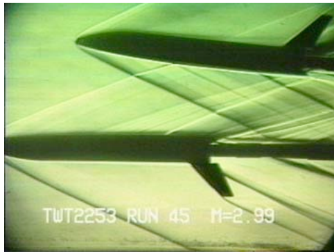
(c) \bar{x}/l_{ref} = 0.4, \bar{z}/l_{ref} = 0.25, \bar{\beta} = 5
