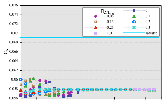
Figure 15: Variation of bimese-orbiter axial force coefficients with \bar{x}/L_{ref} and \bar{z}/L_{ref} at Mach 3 for \alpha = 0 , \beta = 0 degrees.
