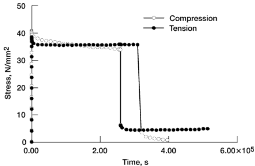
Comparison of the absolute compressive and tensile stress relaxation response at 135 °C at a constant applied strain of \pm 0.5 percent.
