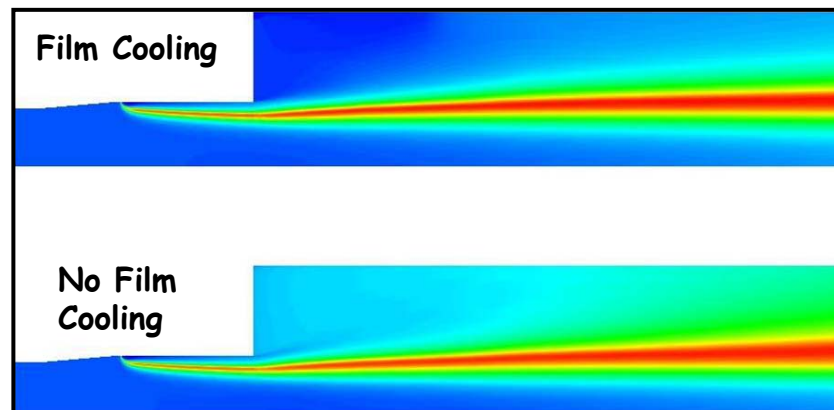
Temperature Contours
