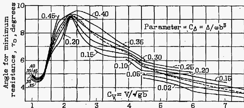
Figure 7.-Variation of angle for minimum resistance, \tau_0 , with speed coef., C_V .
