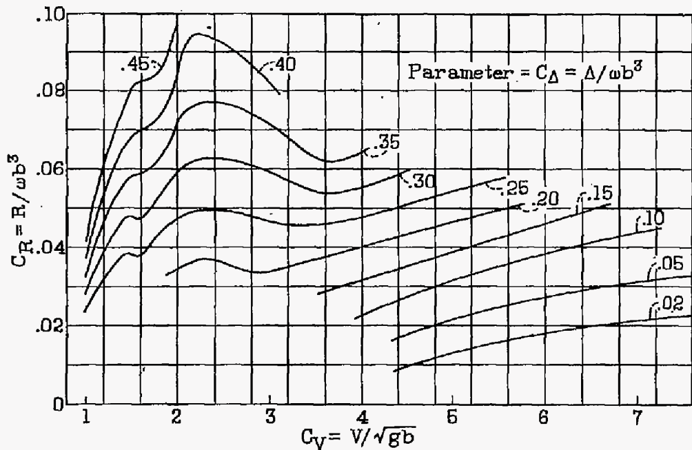
Figure 8.-Resistance coefficient at best trim angles.
