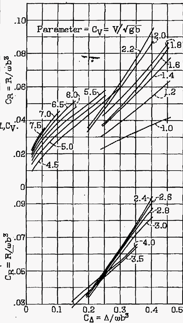
Figure 9.- C_R against C_\Delta at best trim angles.
