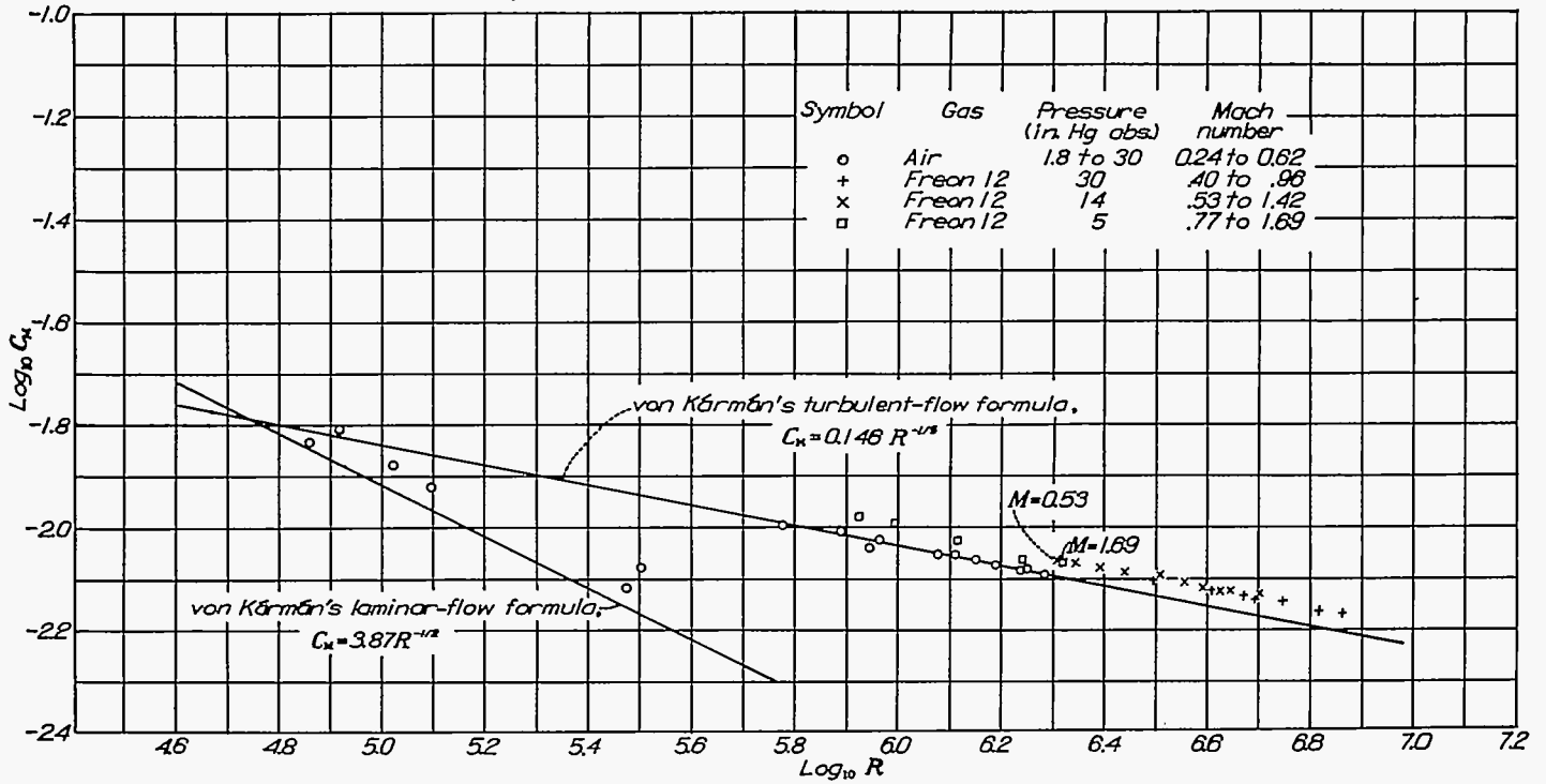
FIGURE 5.—Moment coefficient for disks as function of Reynolds number for several values of Mach number with air and Freon 12 as mediums. Maximum Mach number, 1.69.
