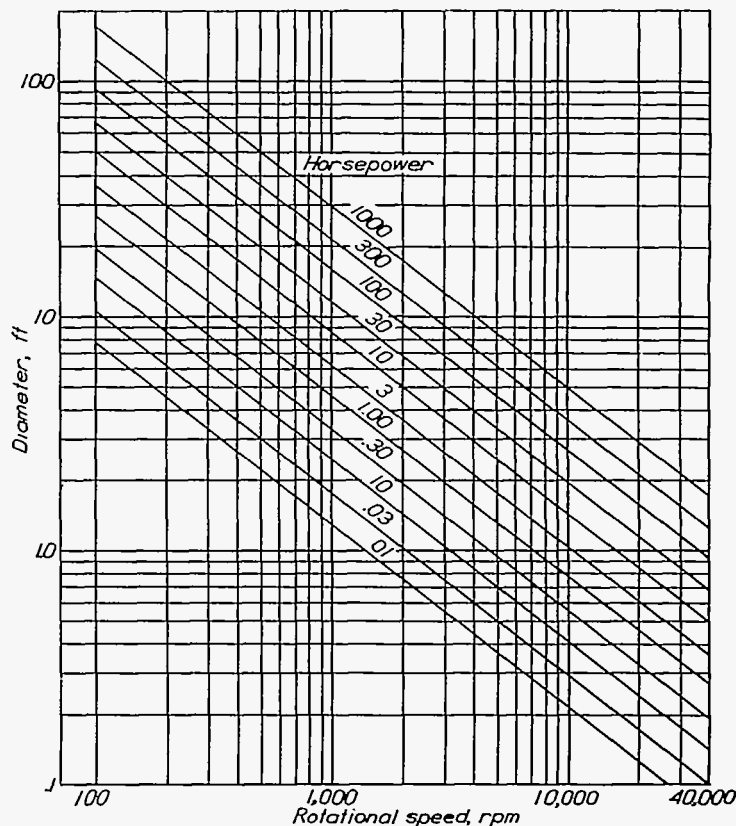
FIGURE 18.—Power requirement for smooth cylinders (1-ft length).
