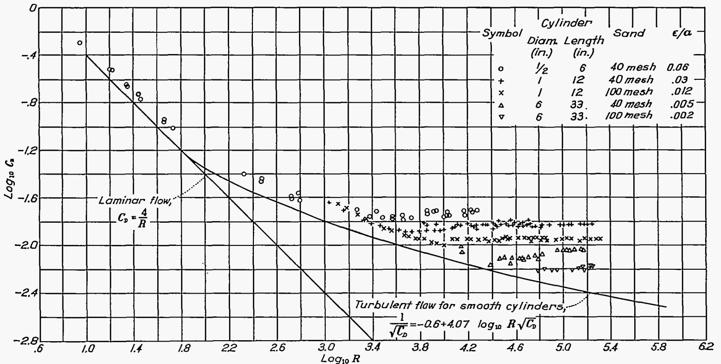
FIGURE 8.—Effect of surface roughness, or grain size, on the drag coefficient. Saturation density of particles.
