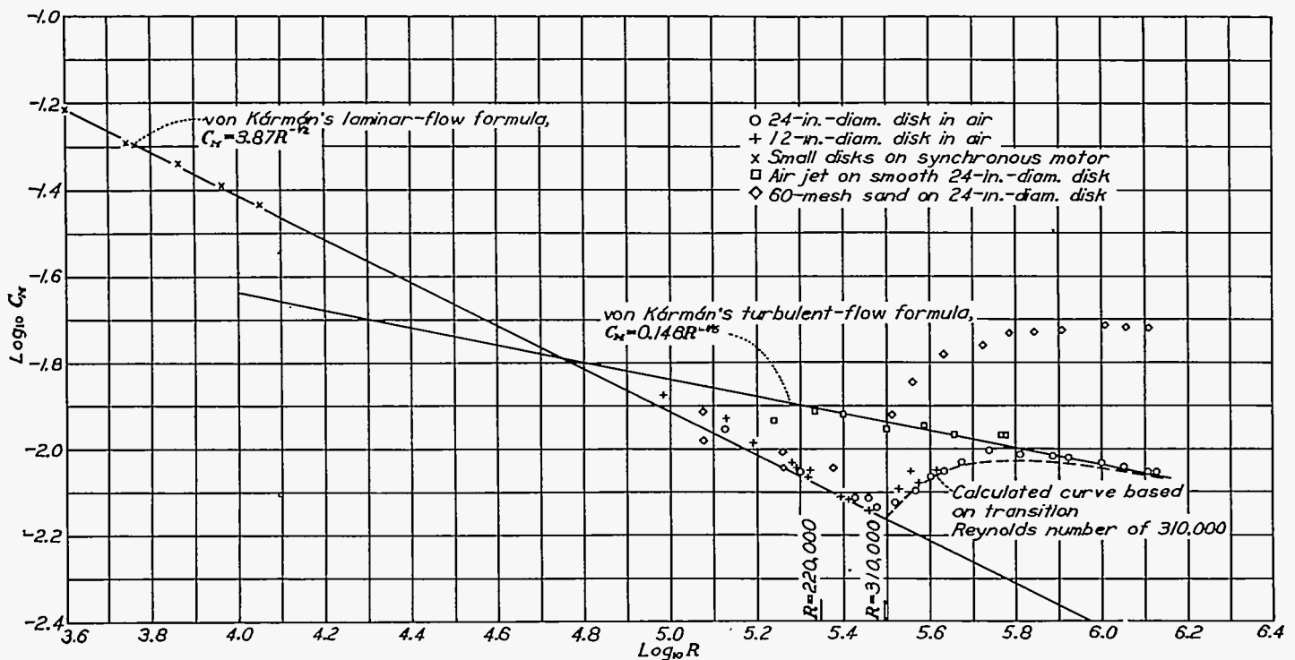
FIGURE 2.—Moment coefficient C_M = \frac{M}{\frac{1}{2}\rho\omega^2 a^3} for disks as function of Reynolds number.
