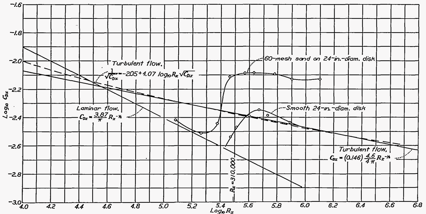
FIGURE 3.—Local drag coefficient for disks obtained by differentiating the moment-coefficient curve.
