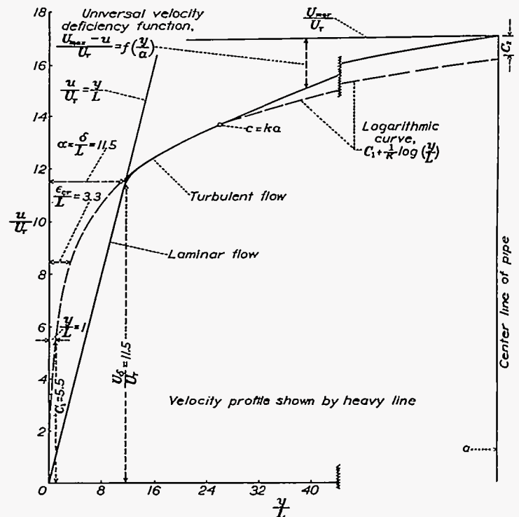
FIGURE 1.—Parameters and functions of the velocity profile by the von Kármán-Prandtl theory.
