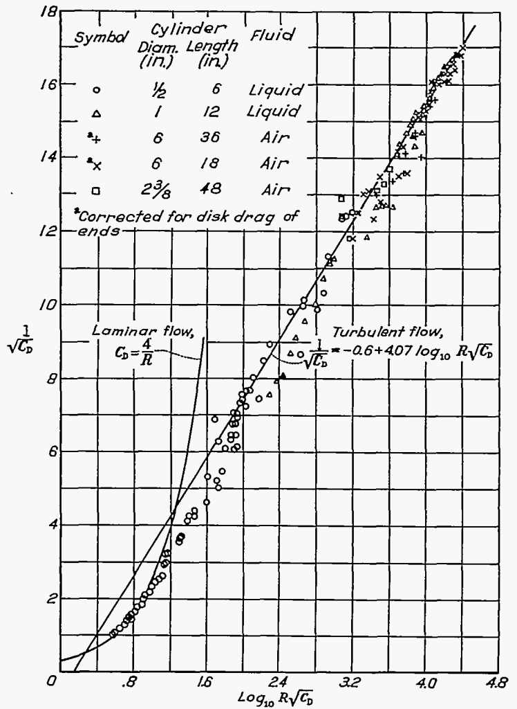
FIGURE 7.—Drag parameter \frac{1}{\sqrt{C_D}} for smooth cylinders as function of \log_{10} R\sqrt{C_D} .
