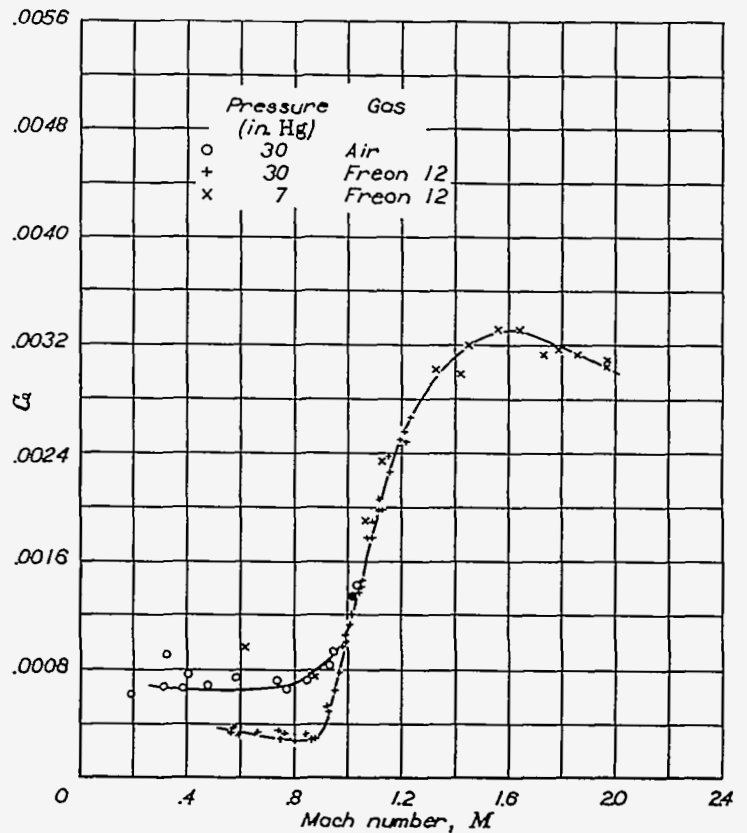
FIGURE 12.—Torque coefficient C_Q = \frac{Q}{\rho n^2 D^5} as function of Mach number for propeller E.
