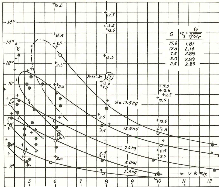
Figure 15.- Stability limits of the flat planing surface.
