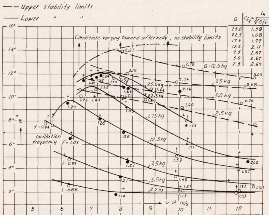
Figure 25.- Measured values for DVL 19, \frac{l}{b_{st}} = 9.19 , \zeta = 130^\circ .
