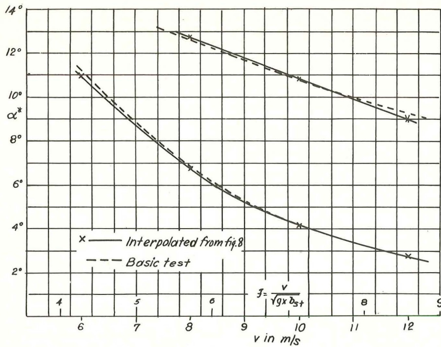
Figure 10.- Limits for direct and indirect towing method.
