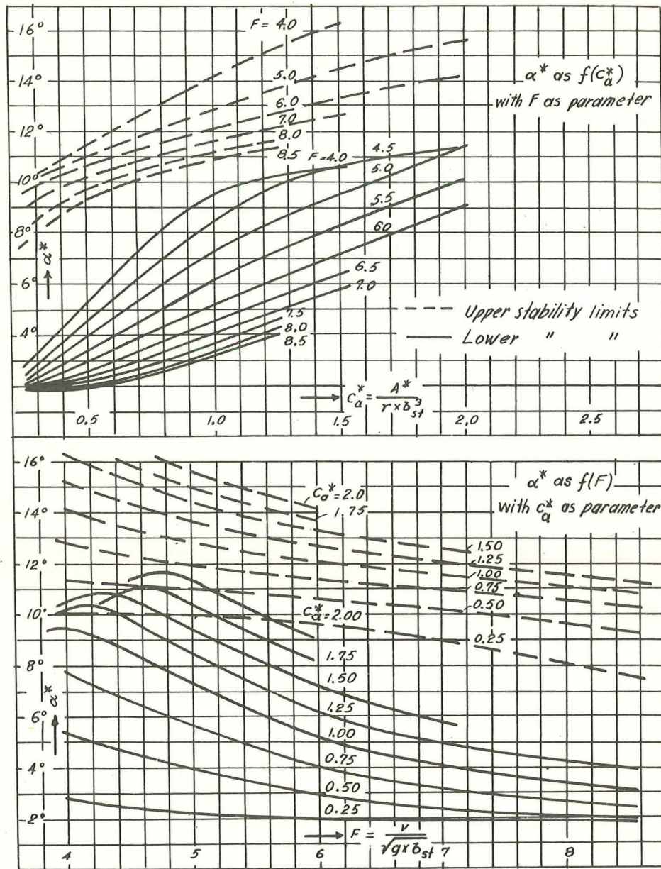
Figure 27.- Dimensionless work sheet for DVL 18, \frac{l}{b_{st}} = 7.50 , \zeta = 130^\circ .
