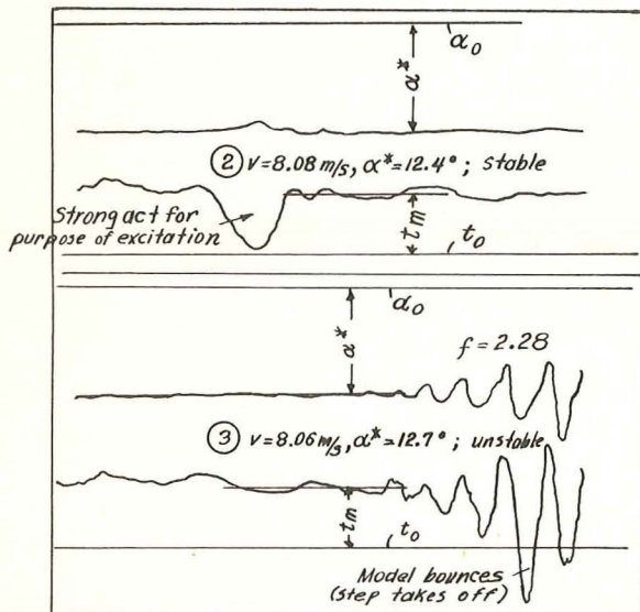
(b) 8m/s: Photograph figure 4(b) shows a stable run for \alpha^* = 12.4^\circ . The afterbody is still supporting. Recording No. 2 shows the strong damping at touch of the model. Recording No. 3 shows the oscillation occurring if the attitude is increased by only 0.3^\circ . The porpoising amplitude has, after only 4 oscillations, increased so much that the step takes off from the water. The afterbody remains in contact with the water; thus a rotation about an instantaneous point of rotation shifted far to the rear takes place.
