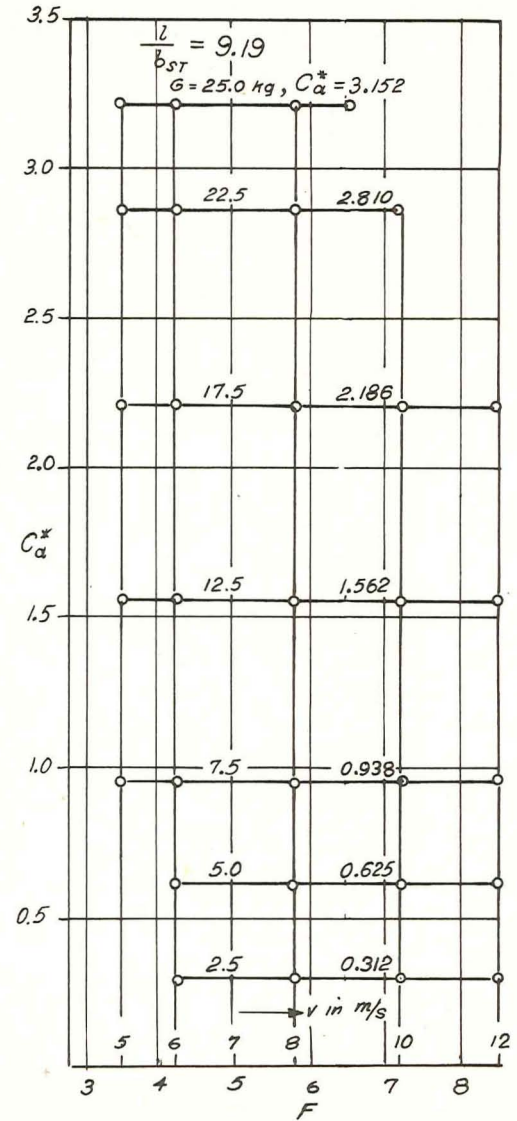
Figure 22.- Scheme of investigation for the series of DVL float families.
