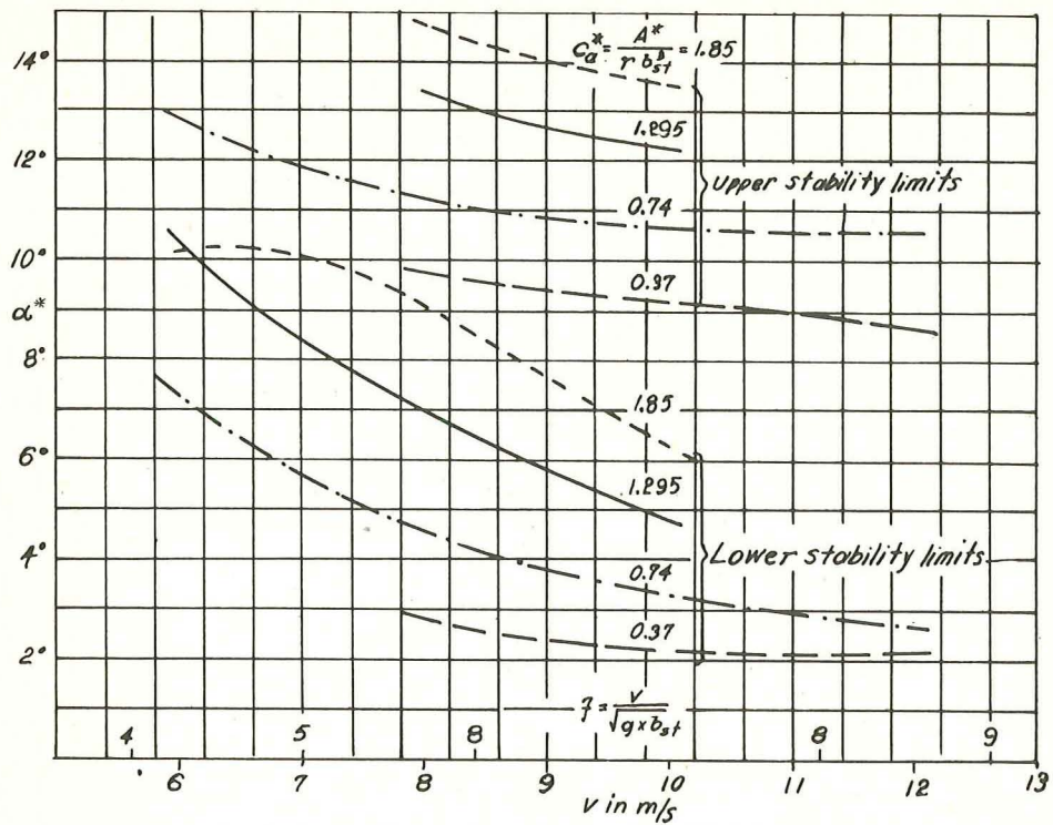
Figure 8.- Influence of the loading.
