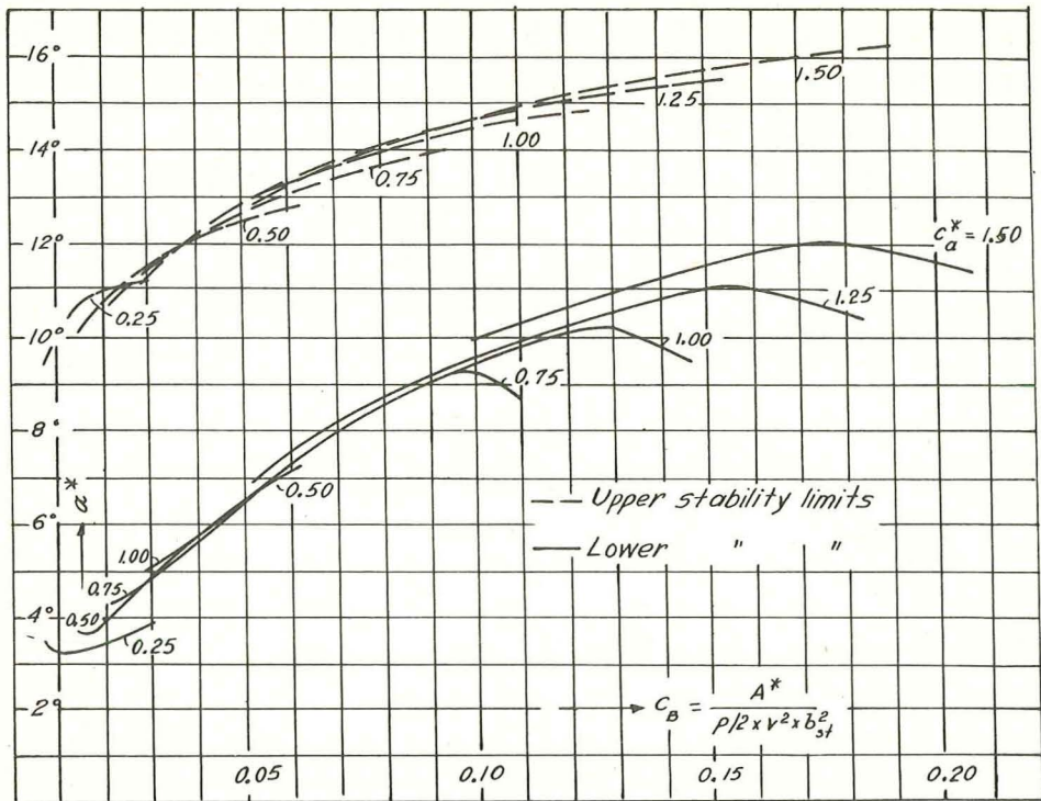
Figure 29.- \alpha^* as f(c_B) with c_a^* as parameter for DVL 17.
