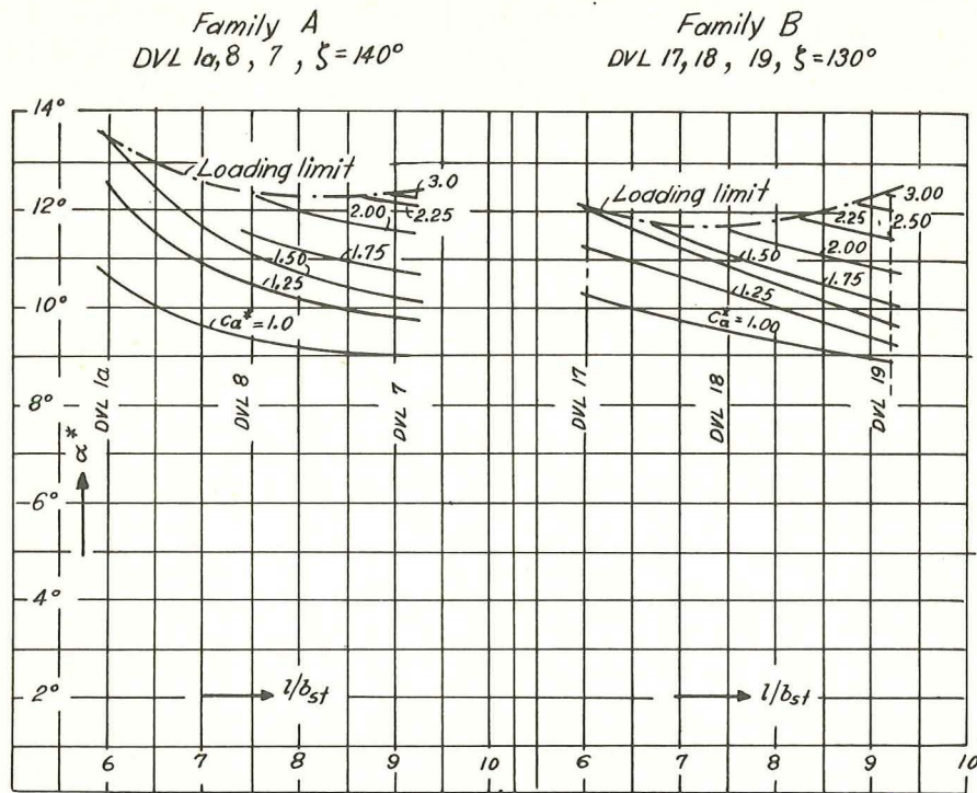
Figure 33.- Series DVL float families A and B of 140^\circ and 130^\circ keel angle; comparison of the stability maxima of the lower limit.
