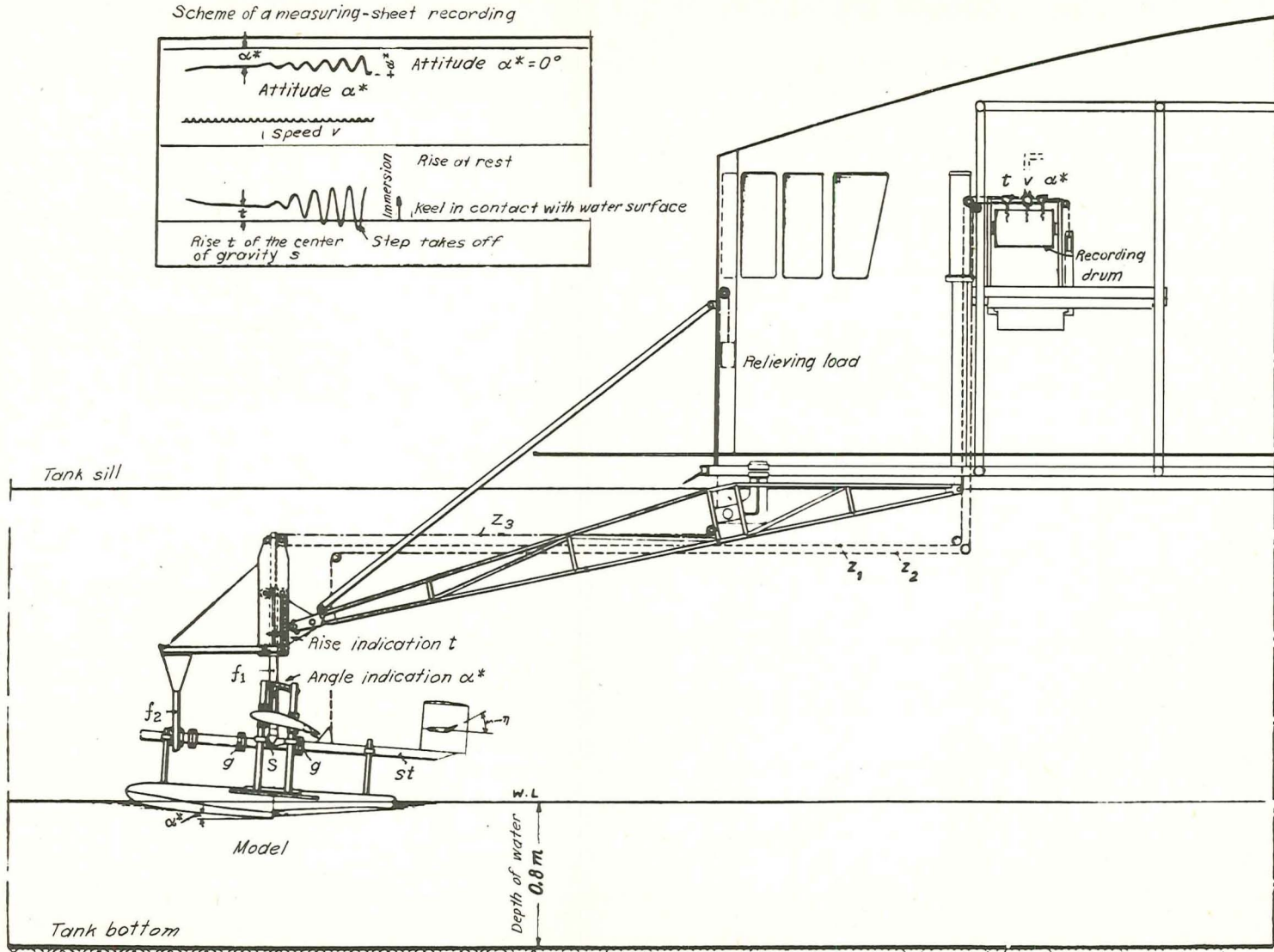
Figure 2.- Measuring apparatus for porpoising tests.
