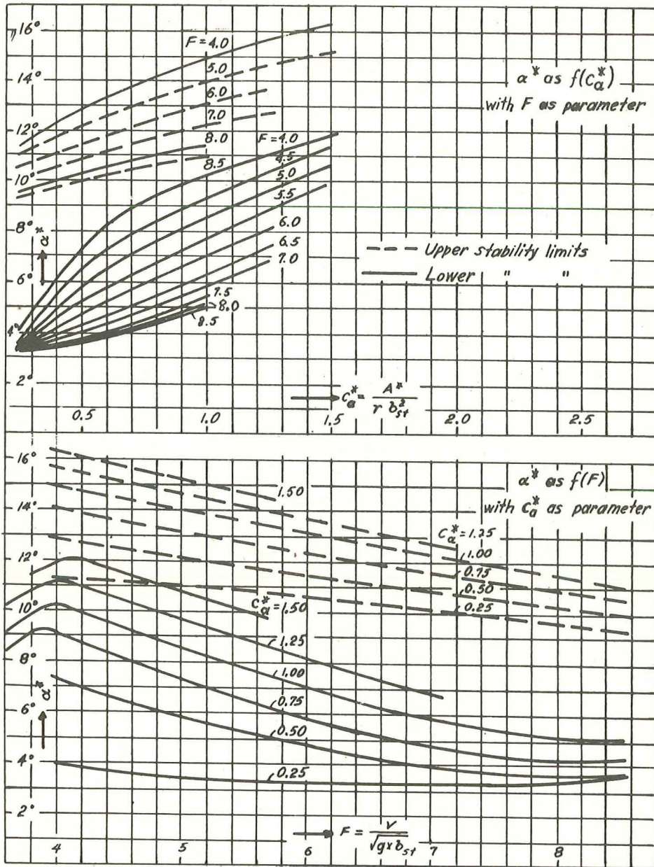
Figure 26.- Dimensionless work sheet for DVL 17, \frac{l}{b_{st}} = 6.04 , \zeta = 130^\circ .
