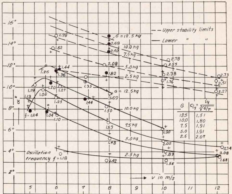
Figure 23.- Measured values for DVL 17, \frac{z}{b_{st}} = 6.04 , \zeta = 130^\circ .
