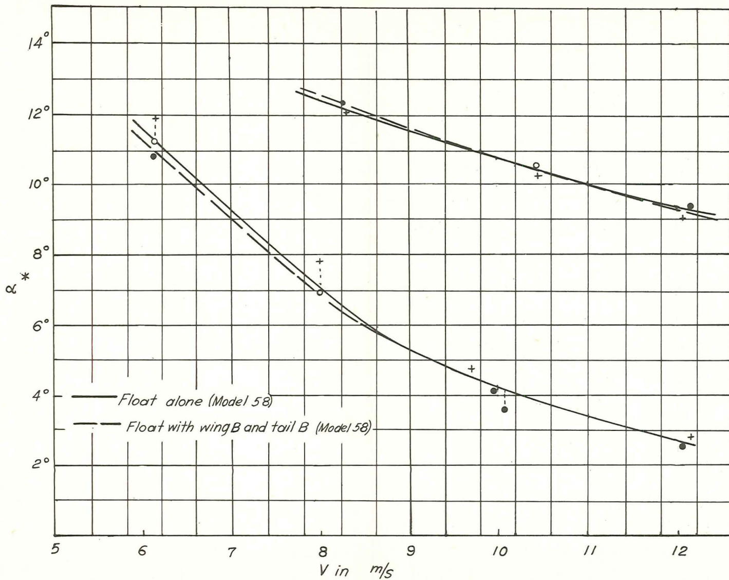
Figure 6.- Float design DVL 18 without wing and tail plane in comparison to the basic test.
