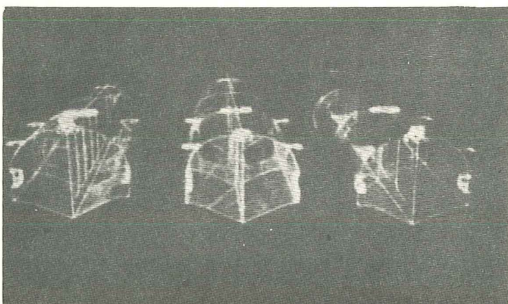
Figure 13.- Forebodies of the series of DVL float family of 130^{\circ} keel angle.
