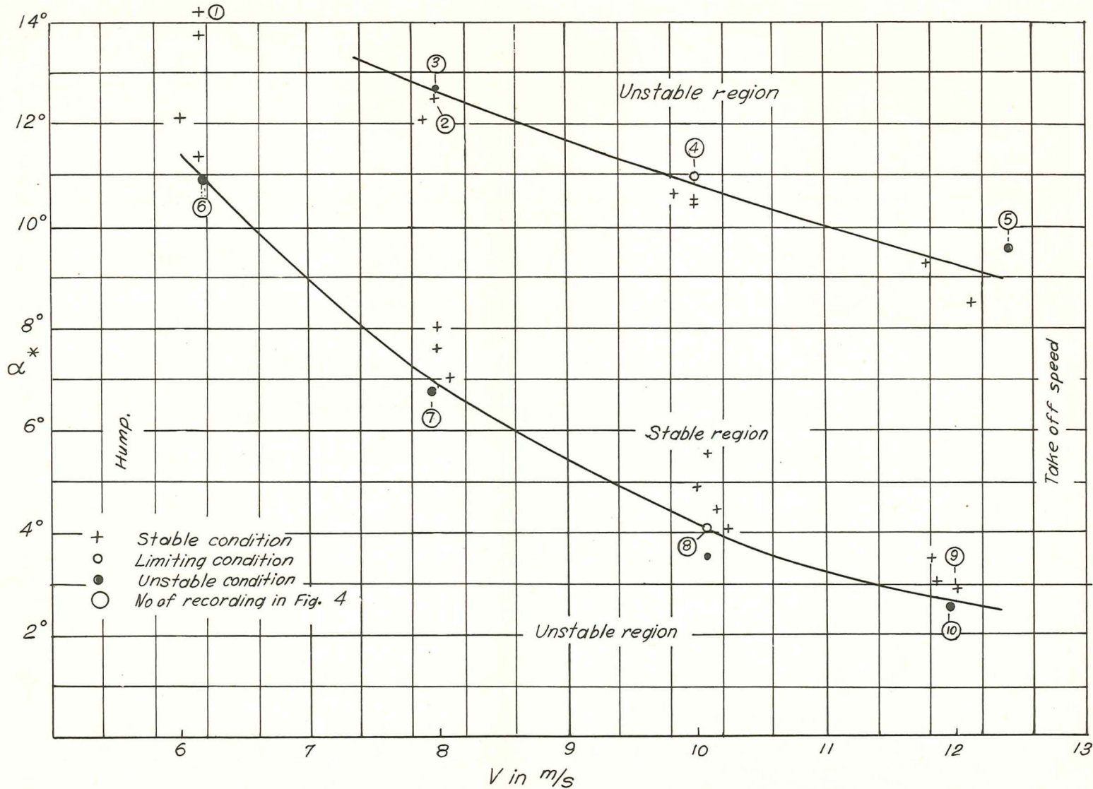
Figure 3.- Basic test. Float design DVL 18 with wing and tail plane.
