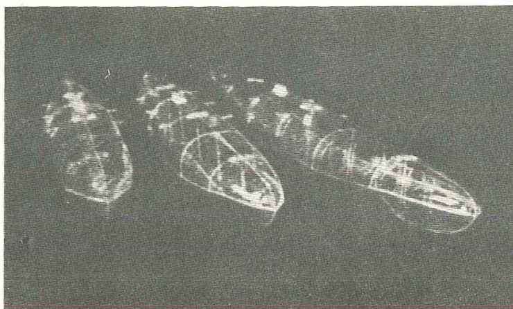
Figure 14.- Series of DVL float family of 130^{\circ} keel angle.
