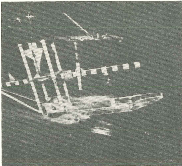
Figure 17.- Flat planing surface; A^* = 12.5\text{kg} , \alpha^* = 10.2^\circ , v = 7.8\text{m/s} stable only for perfectly calm water; porpoising oscillations proper for slightly rippled water.
