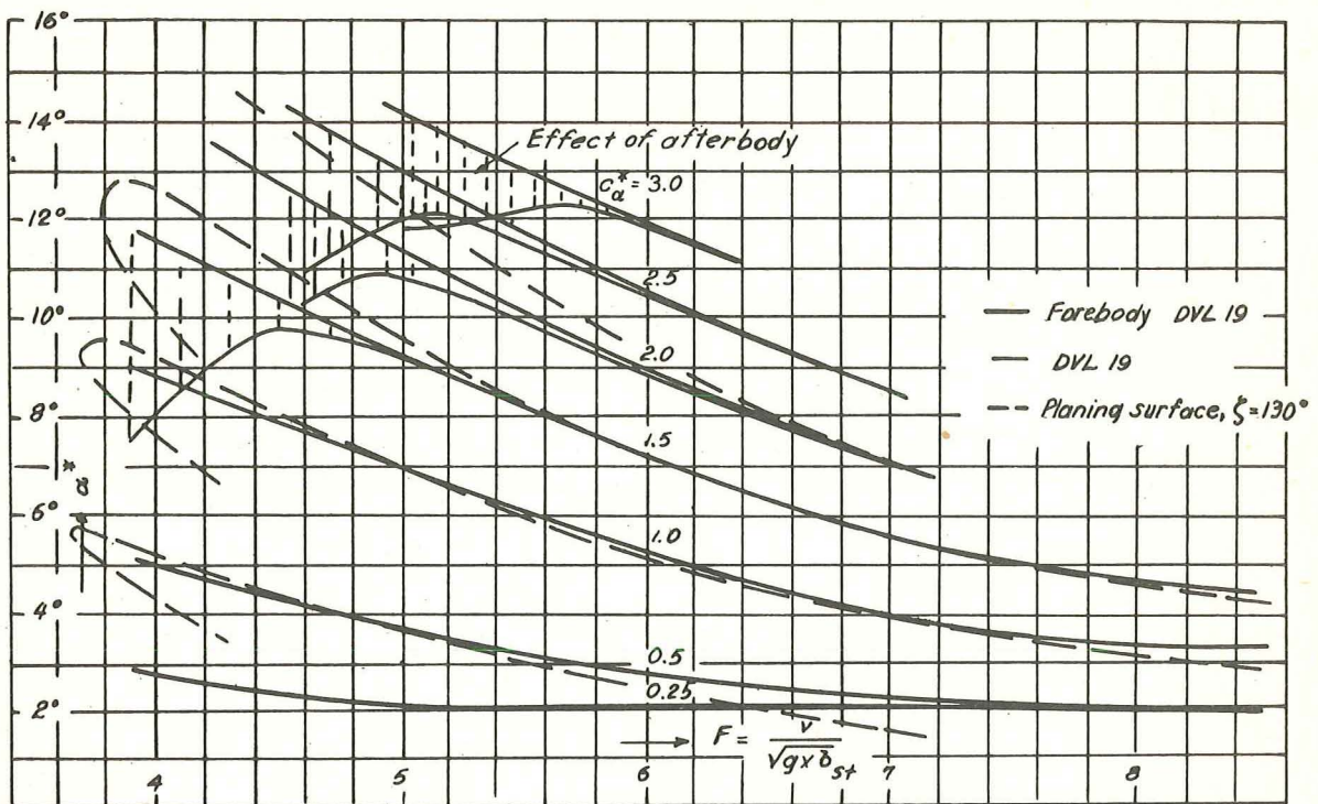
Figure 20.- Long forebody DVL 19; comparison with float DVL 19 and planing surface with 130^\circ keel angle.
