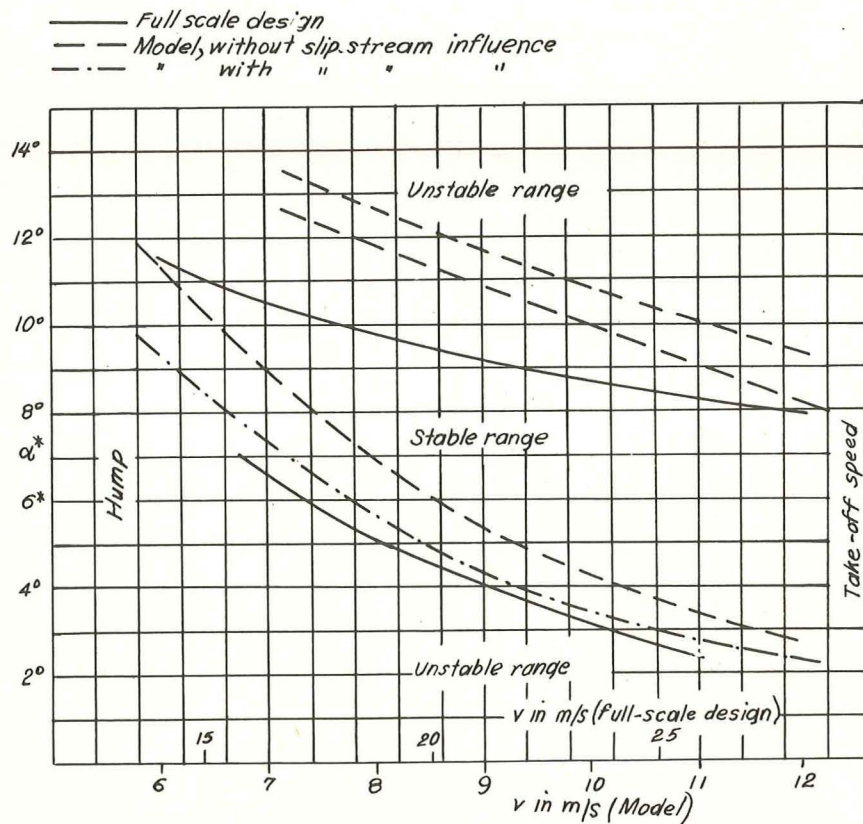
Figure 11.- Comparison between model and full-scale design.
