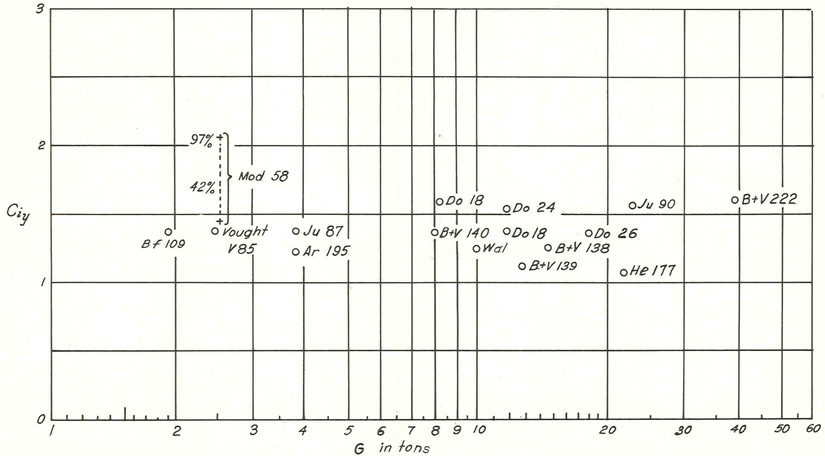
Figure 5.- Coefficient of the moment of inertia as a function of the flying weight.
