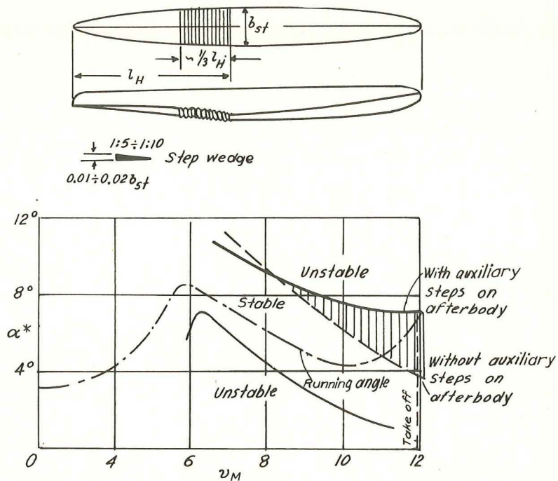
Figure 34.- Favorable shifting of the upper stability limit by use of auxiliary steps on the afterbody.
