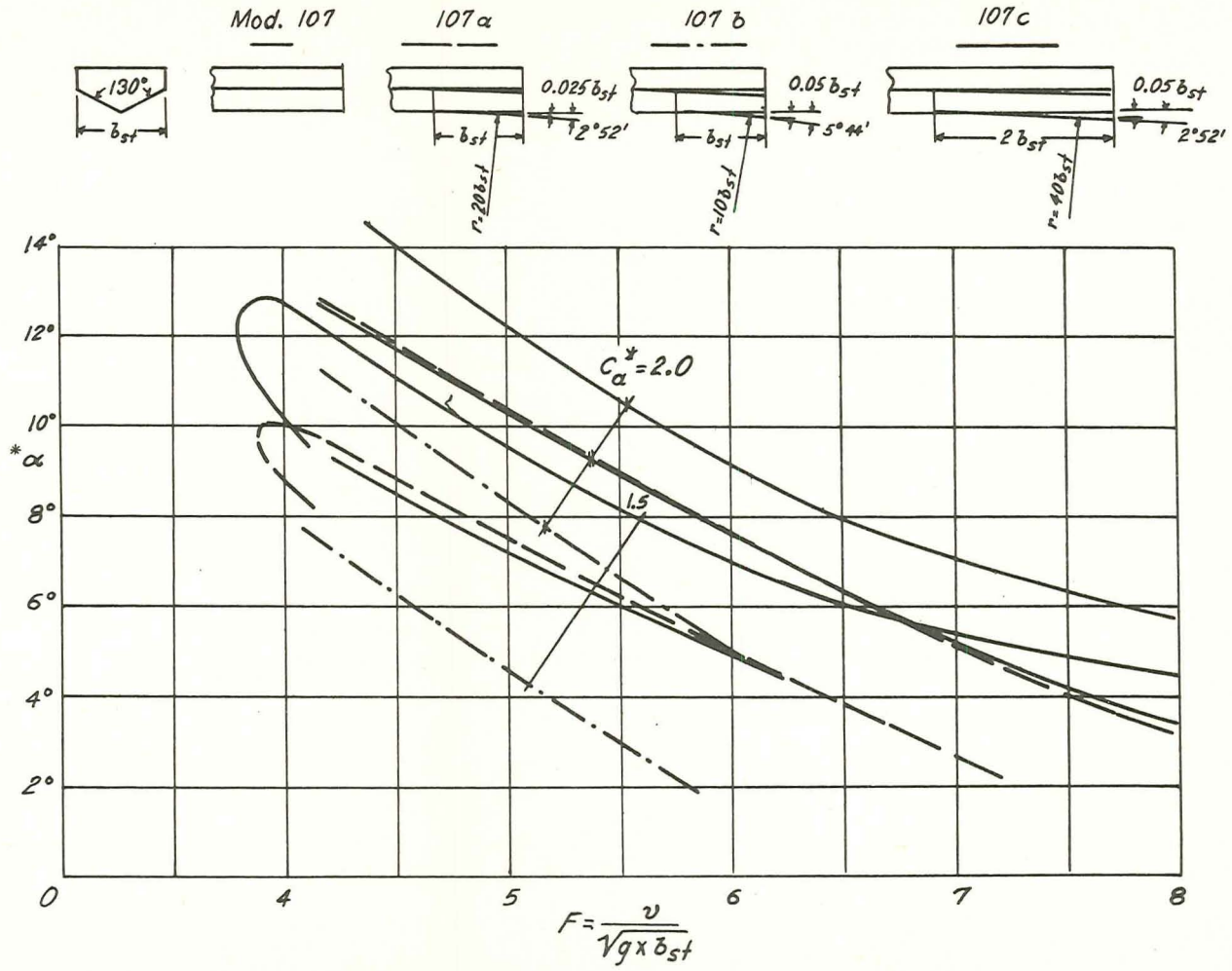
Figure 36.- Influence of a slight concavity of the bottom before the step on the position of the lower limit for the planing surface with a keel angle of 130^\circ .
