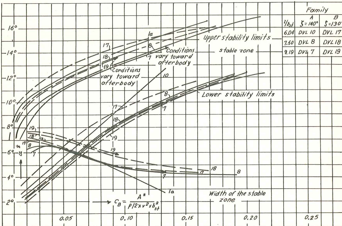
Figure 32.- Series DVL float families A and B of 140° and 130° keel angle; comparison of the mean stability limits.
