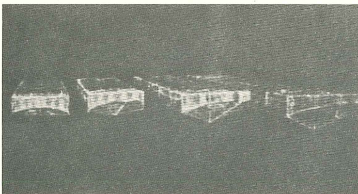
Figure 12.- Planing surfaces with 130^{\circ} , 140^{\circ} , 160^{\circ} , and 180^{\circ} keel angle.
