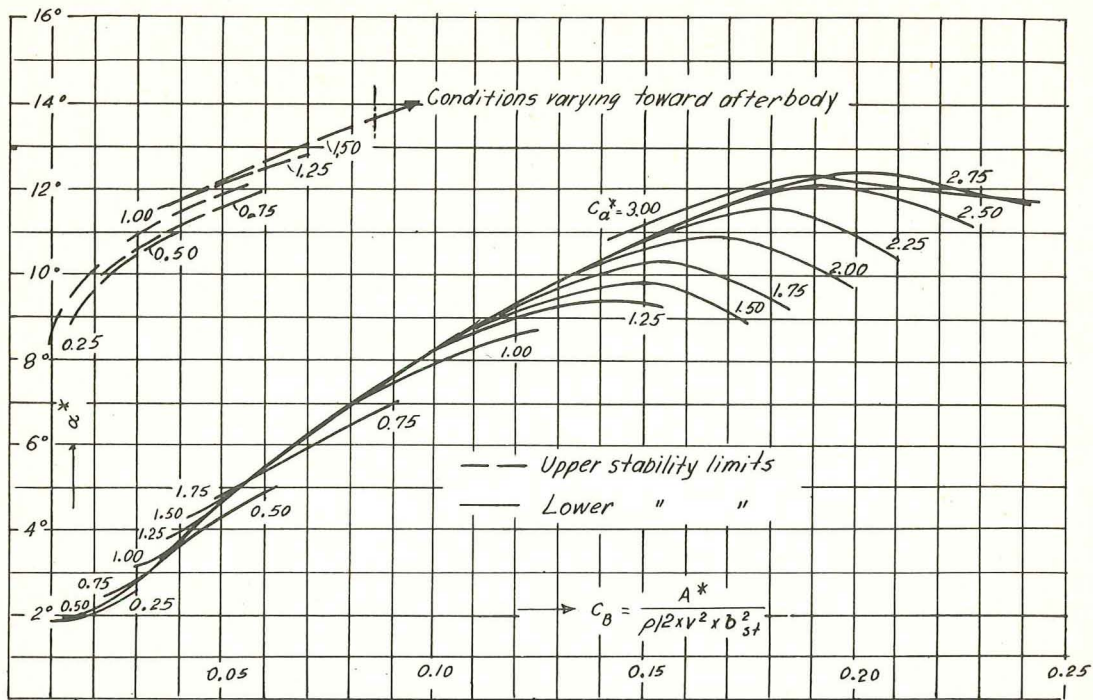
Figure 31.- \alpha^* as f(c_B) with c_a^* as parameter for DVL 19.
