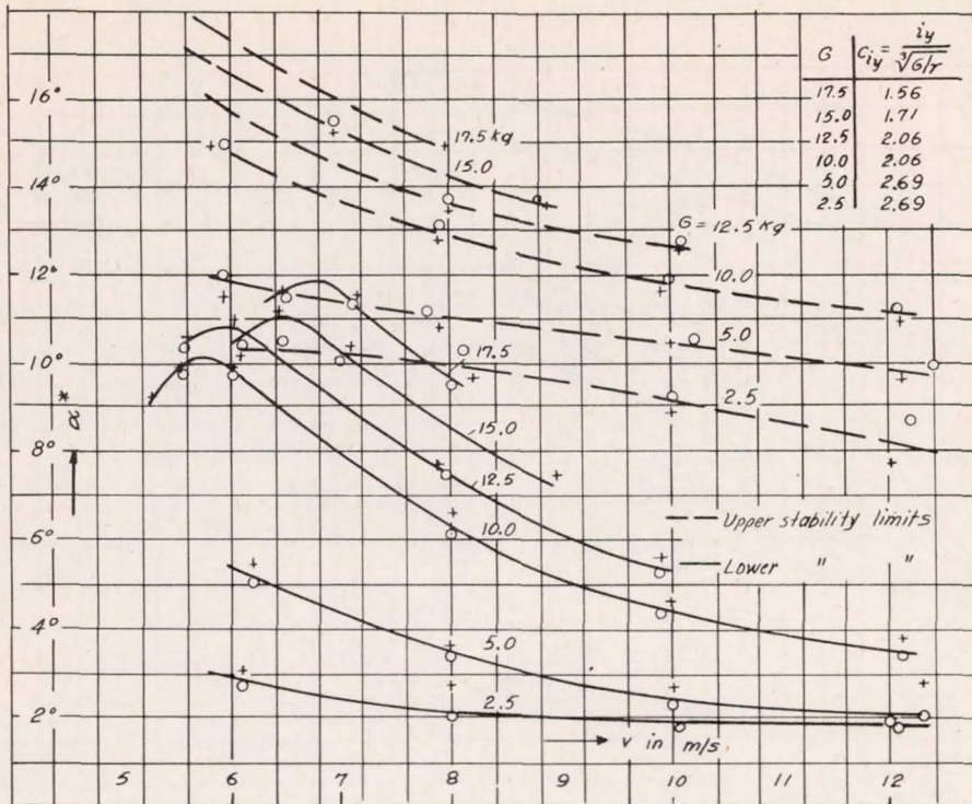
Figure 24.- Measured values for DVL 18, \frac{l}{b_{st}} = 7.50 , \zeta = 130^\circ .
