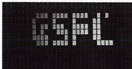
Figure 11. 64 X 128 MSA array electrically addressed to display 'GSFC'
