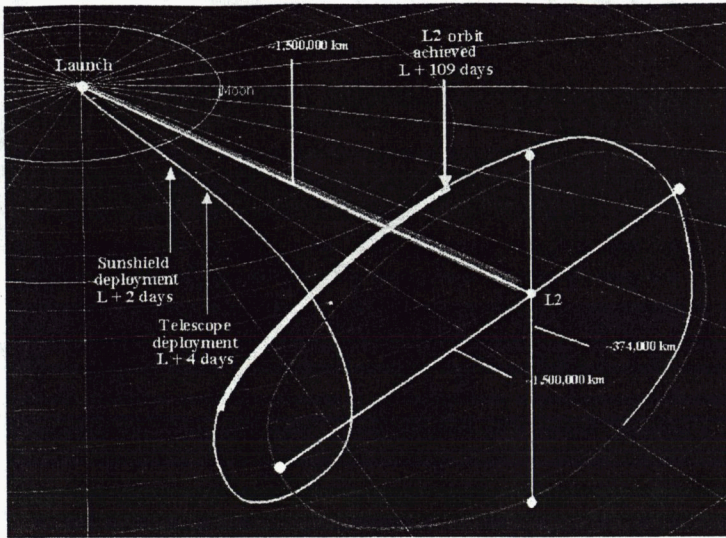
Figure 3. JWST Launch Trajectory
