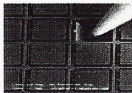
Figure 10. Electron micrograph of a prototype JWST micro-shutter array. Light shields that mask gaps around the periphery of each shutter are removed for clarity.
