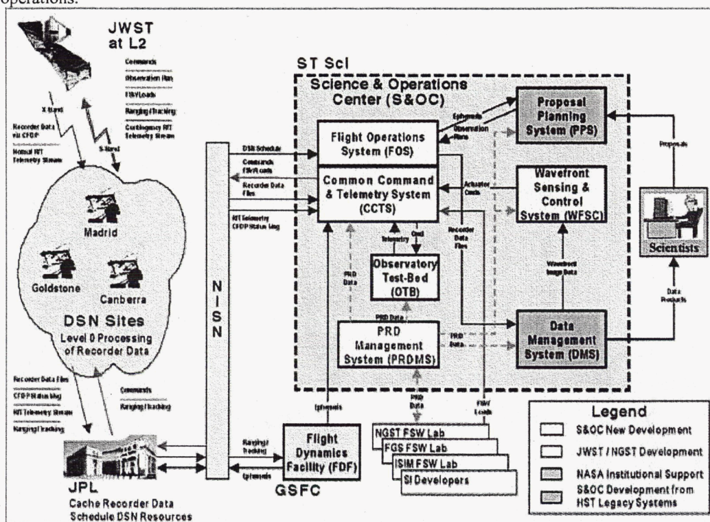
Figure 15. JWST Mission Operations Block Diagram
