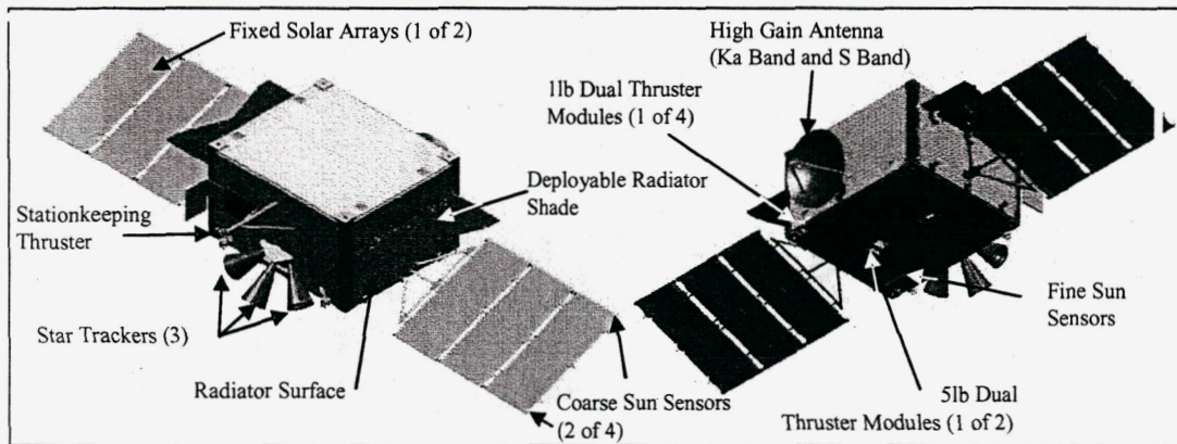
Figure 13. JWST Spacecraft Bus External Configuration
