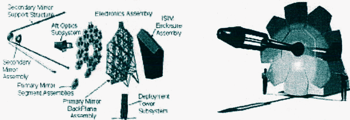
Figure 5. JWST Optical Telescope Element
