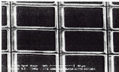
Figure 12. Close up of 100 X 200 micron pixel size with light shields attached
