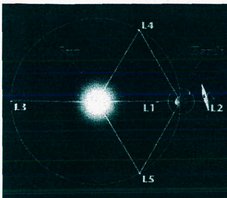
Figure 2. The Second LaGrange Point
