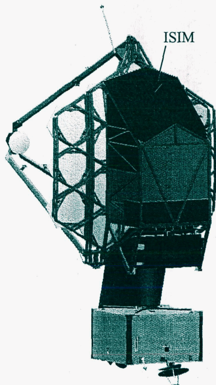
Figure 8. Integrated Science Instrument Module (ISIM) (sunshade omitted)
