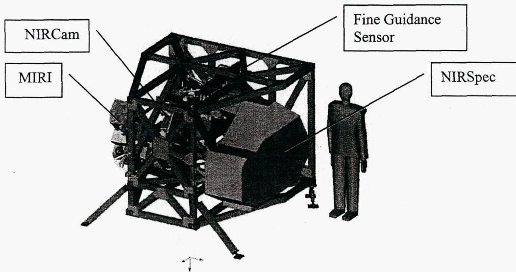
Figure 9. ISIM. (Enclosure removed for clarity)
