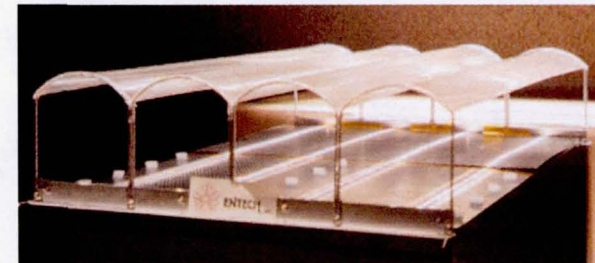
Developed in 1999-2000: Flexible-Blanket Version of Stretched Lens Array (SLA)
