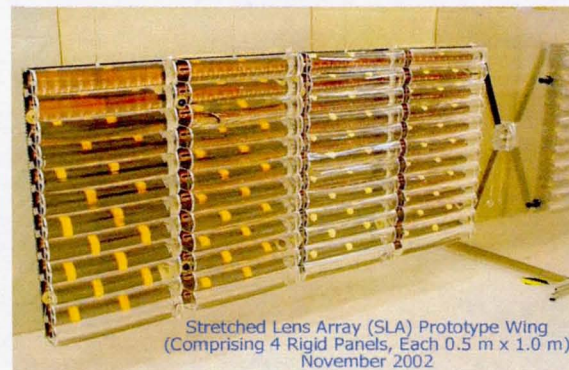
Developed in 2001-2002: Rigid Panel Version of SLA
