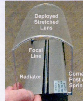
Stretched Lens Invented in 1998
