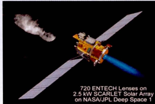
Developed in Mid-1990's, Launched in 1998: SCARLET Array on Deep Space 1
