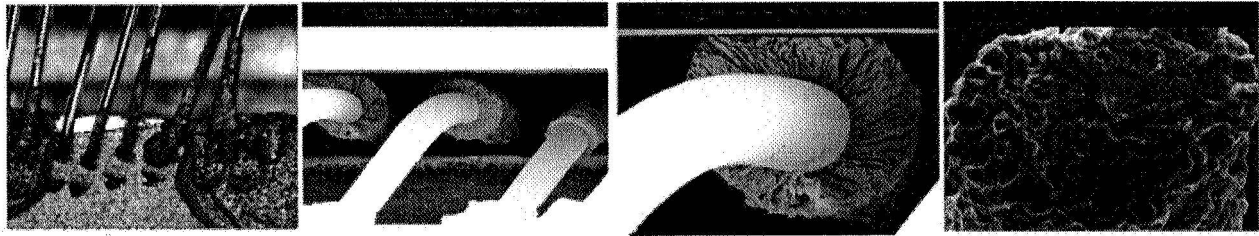
Figure 5: From left to right, a) Indium creep onto the gold wires, b) & c) SEM images of indium attack, d) cross section of gold/indium intermetallic on the gold wire.
