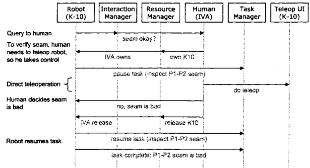
Figure 8: Execution sequence of human supporting a robot.
