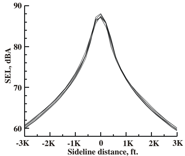
Figure 12. Variability of RNM predicted sound exposure levels for housekeeping runs; level flyovers at 110 knots; MD600N.
