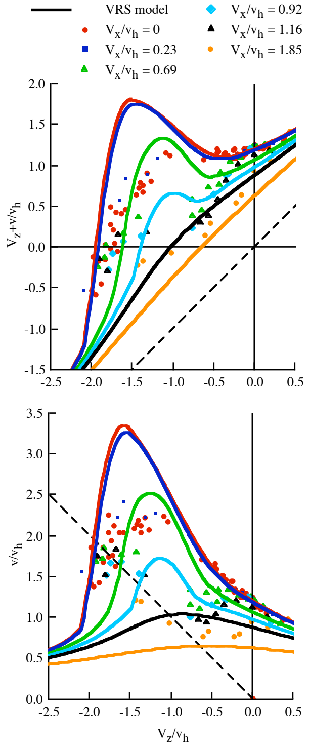
Figure 51. Taghizad (2002) flight test: nonaxial flow; \sigma = 0.083 , \theta_{tw} = -10 deg; \kappa = 1.20 .
