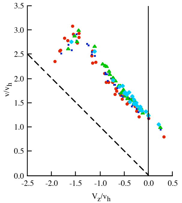
Figure 11. Yaggy and Mort (1962) wind tunnel test: axial flow; \sigma = 0.20 , \theta_{tw} = -22.4 deg, flapping propeller.
