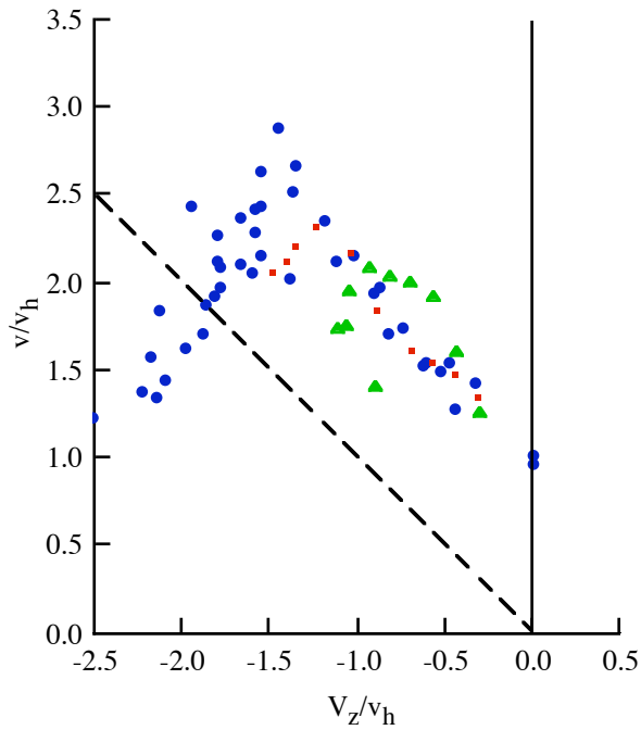
Figure 22(c). Washizu (1966) moving track test: rear rotor; \sigma = 0.0573 , \theta_{tw} = -8.33 deg.
