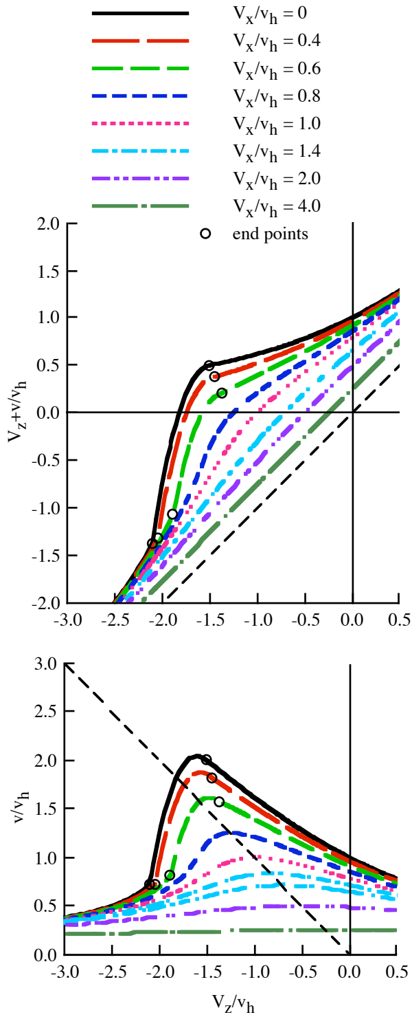
Figure 38. Rotor inflow from baseline model.
