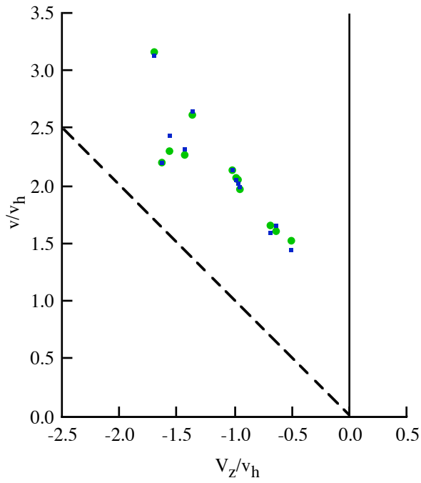
Figure 14. Betzina (2001) wind tunnel test: axial flow; \sigma = 0.1194 , \theta_{tw} = -41 deg, rotor only.
