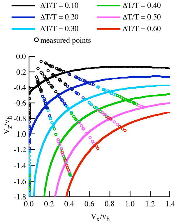
Figure 30. Yaggy and Mort (1962) wind tunnel test: thrust fluctuations; \sigma = 0.20 , \theta_{tw} = -22.4 deg, flapping propeller.
