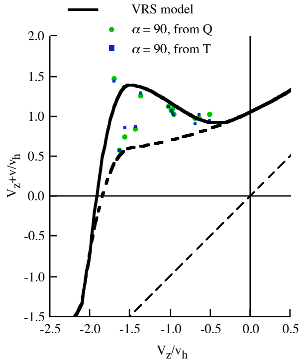
Figure 44. Betzina (2001) wind tunnel test: axial flow; \sigma = 0.1194 , \theta_{TW} = -41 deg, rotor only; \kappa = 1.05 .
