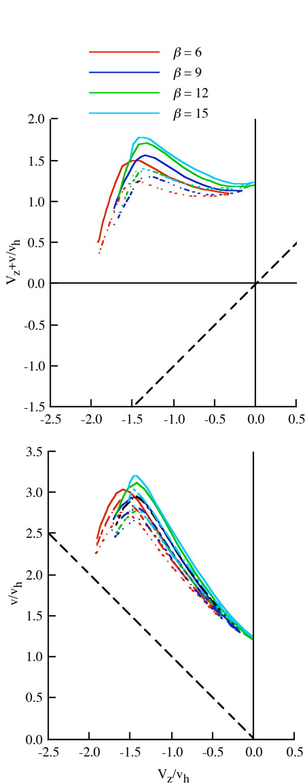
Figure 24. Yaggy and Mort (1962) wind tunnel test: minimum (dotted) and maximum (solid) inflow; \sigma = 0.20 , \theta_{tw} = -22.4 deg, flapping propeller; axial flow, \alpha = 90 deg.
