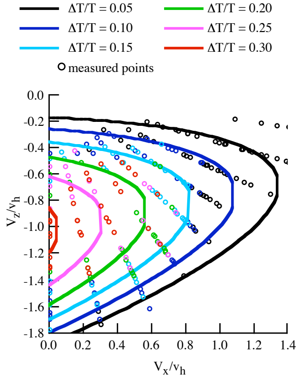
Figure 32(b). Betzina (2001) wind tunnel test: thrust fluctuations; rotor and image plane.
