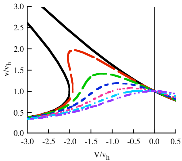
Figure 5(c). Momentum theory in forward flight (function of V and \alpha ).
