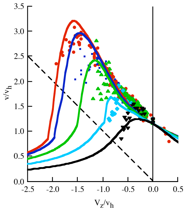
Figure 46. Yaggy and Mort (1962) wind tunnel test: nonaxial flow; \sigma = 0.20 , \theta_{tw} = -22.4 deg, flapping propeller; \kappa = 1.15 .
