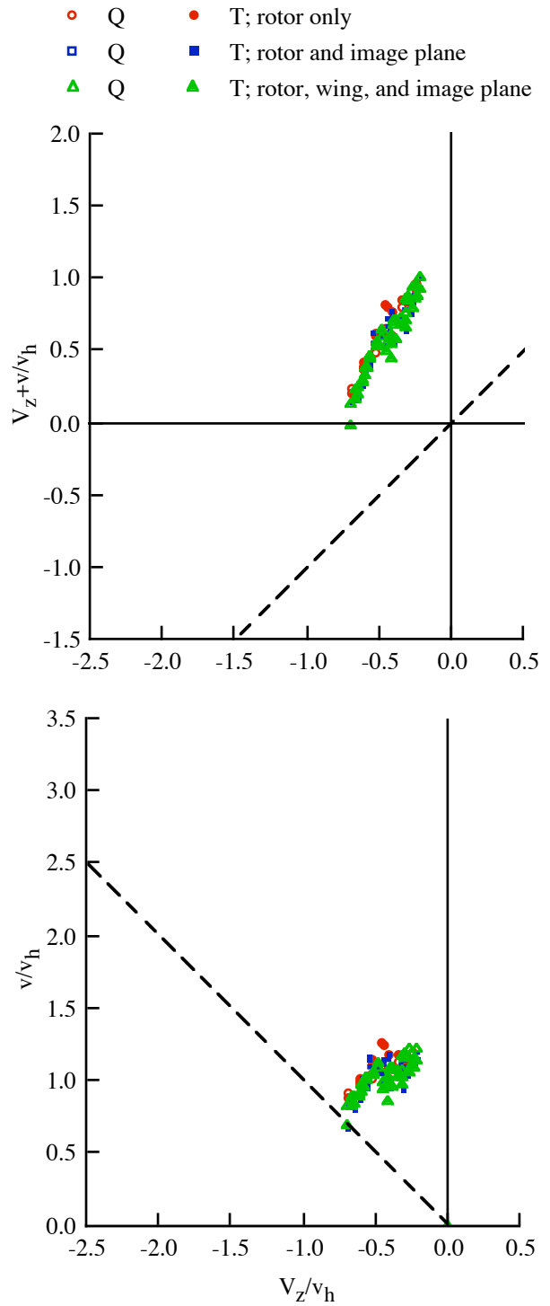
Figure 23(c). Betzina (2001) wind tunnel test: influence of image plane; \sigma = 0.1194 , \theta_{tw} = -41 deg; nonaxial flow, \alpha = 30 deg.
