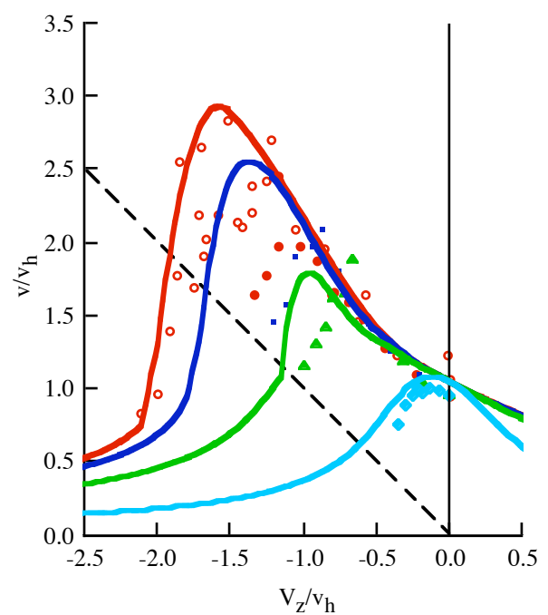
Figure 47. Washizu (1966) moving track test: nonaxial flow; \sigma = 0.0573 , \theta_{tw} = -8.33 deg; \kappa = 1.05 .
