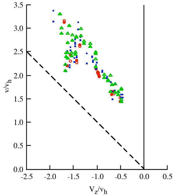
Figure 23(a). Betzina (2001) wind tunnel test: influence of image plane; \sigma = 0.1194 , \theta_{tw} = -41 deg; axial flow, \alpha = 90 deg.
