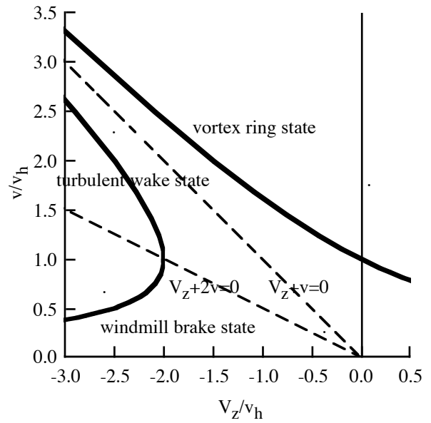
Figure 4. Momentum theory and inflow states in axial flow.
