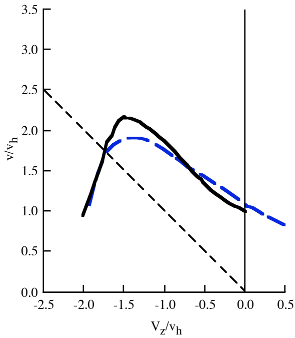
Figure 10. Gessow (1954): axial flow.
