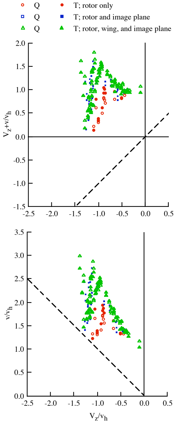
Figure 23(b). Betzina (2001) wind tunnel test: influence of image plane; \sigma = 0.1194 , \theta_{tw} = -41 deg; nonaxial flow, \alpha = 60 deg.
