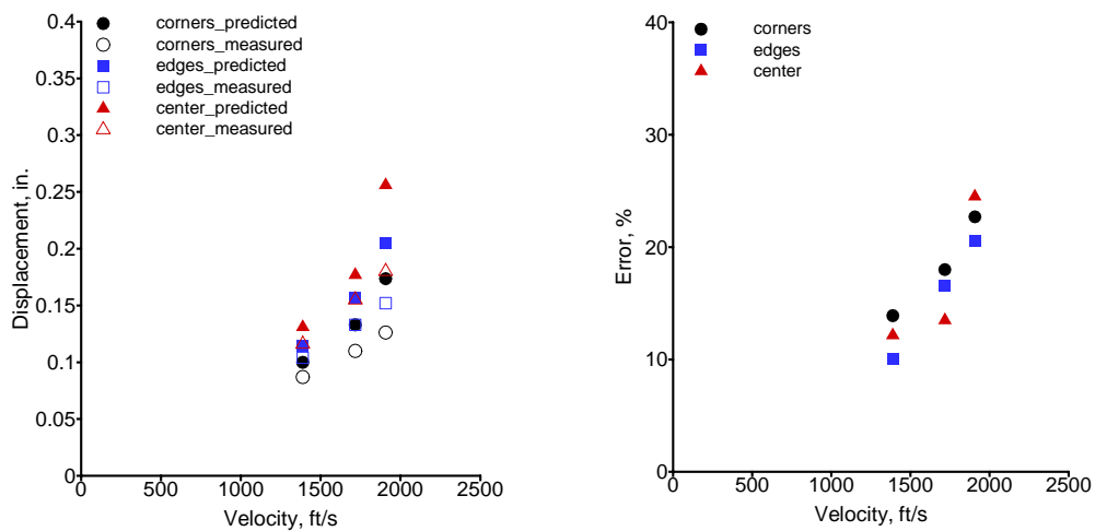
Figure 6. The maximum displacements and percent error of all the correlated data points.
