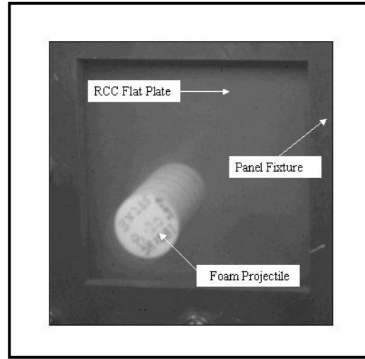
Figure 3. Test set-up showing the BX-265 foam projectile impacting the RCC panel.
