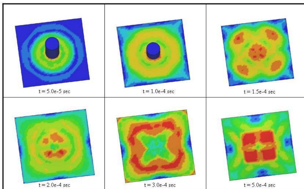
Figure 12. Colored contours of the first-principal stresses at different time intervals for the A146-3 panel. Then impact velocity of the foam is 22,140 in/sec.
