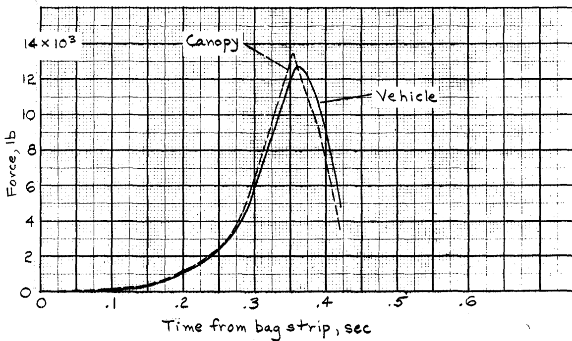
Figure 8.- Inflation loads for two configurations using typical C_D S history (Figure 6); damping coefficient = 25 lb-sec/line.
