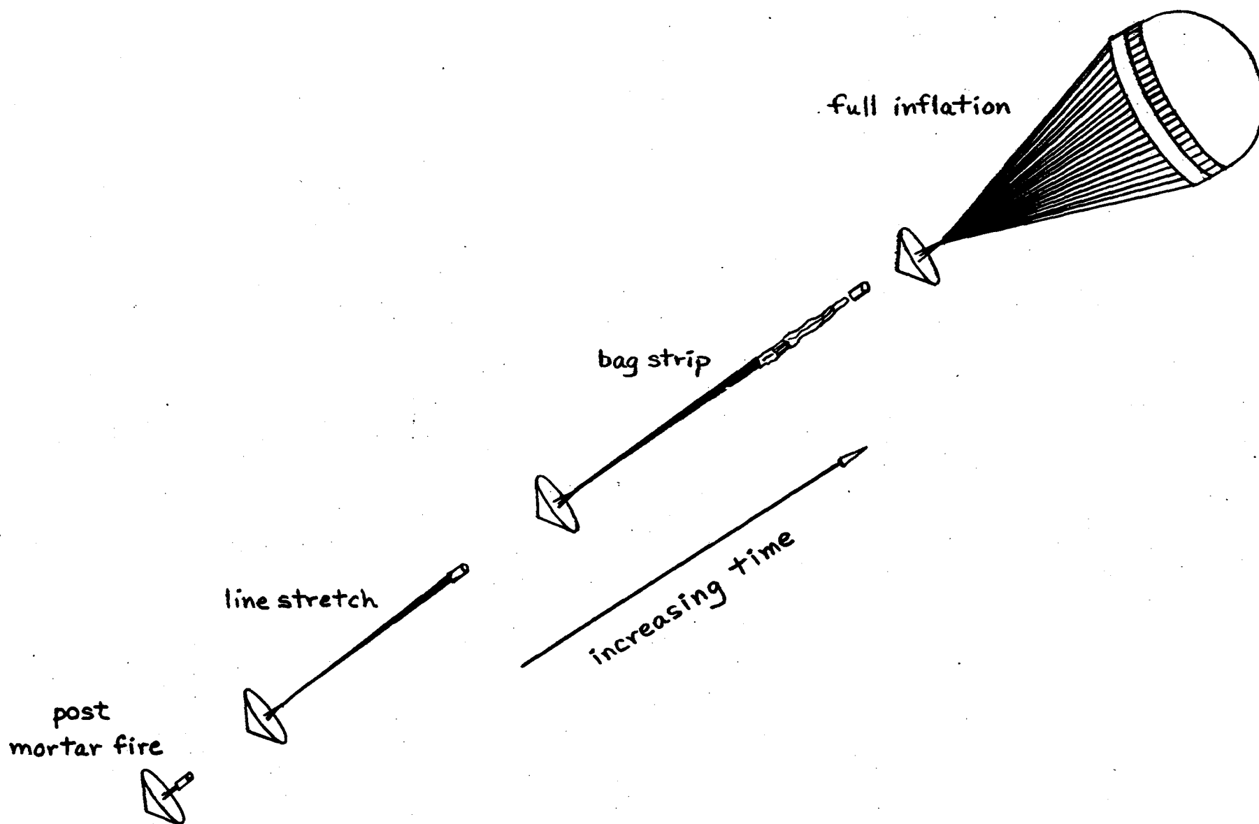
Figure 1.- Sketch of unfurling and inflation sequence.
