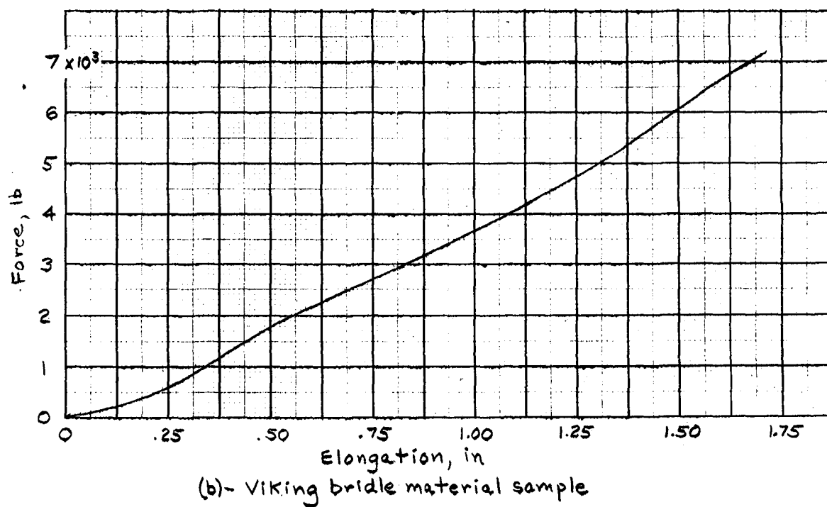
Figure 4.- Force-elongation curves for Viking suspension line and bridle samples, as obtained from Instron tests (gage length \approx 10 in).
