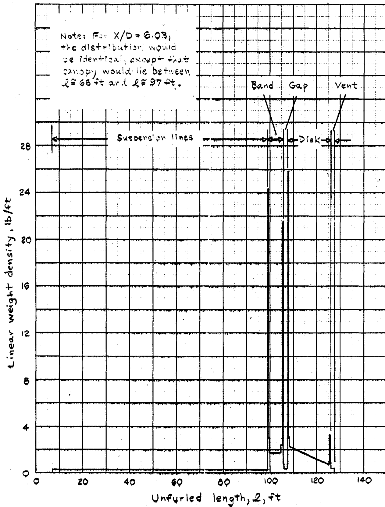
Figure 3.- Linear weight distribution of Viking 53-ft.- D 0 DGB, X/D at full inflation = 8.69.
