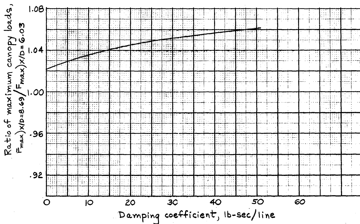
Figure 10.— Ratios of maximum loads for the two Viking configurations as a function of suspension line damping coefficient.
