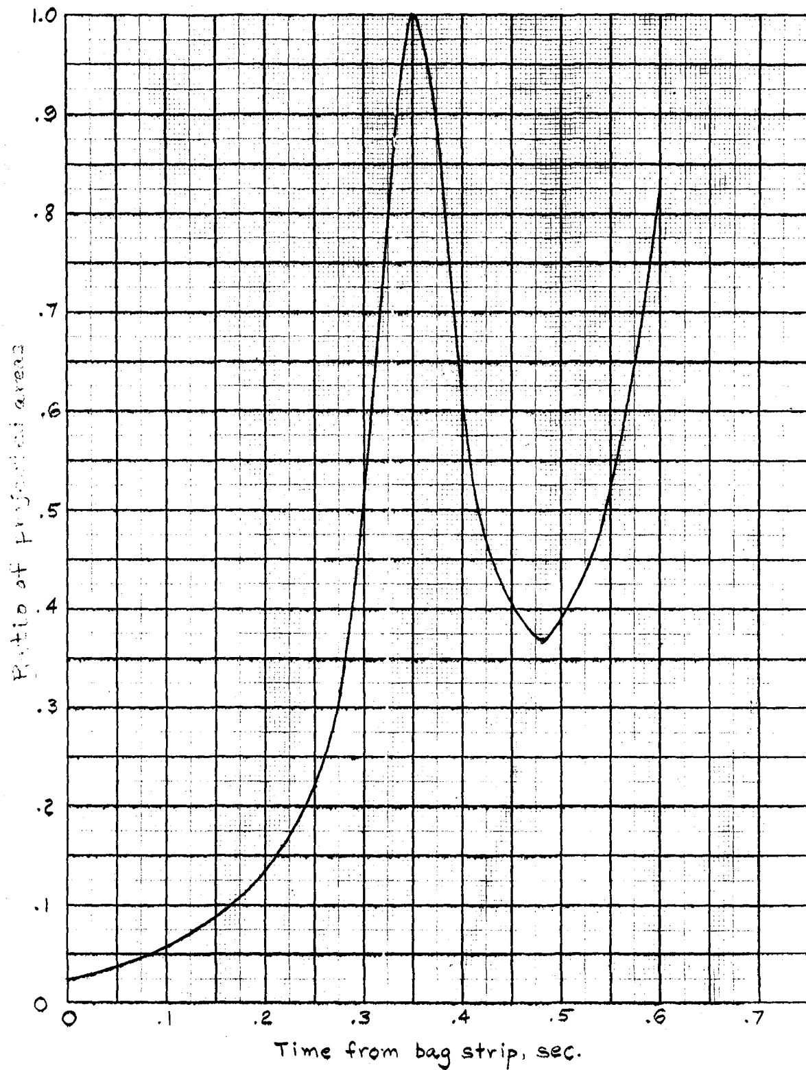
Figure 5.- Input ratio of instantaneous canopy projected area to canopy projected area at full inflation.
