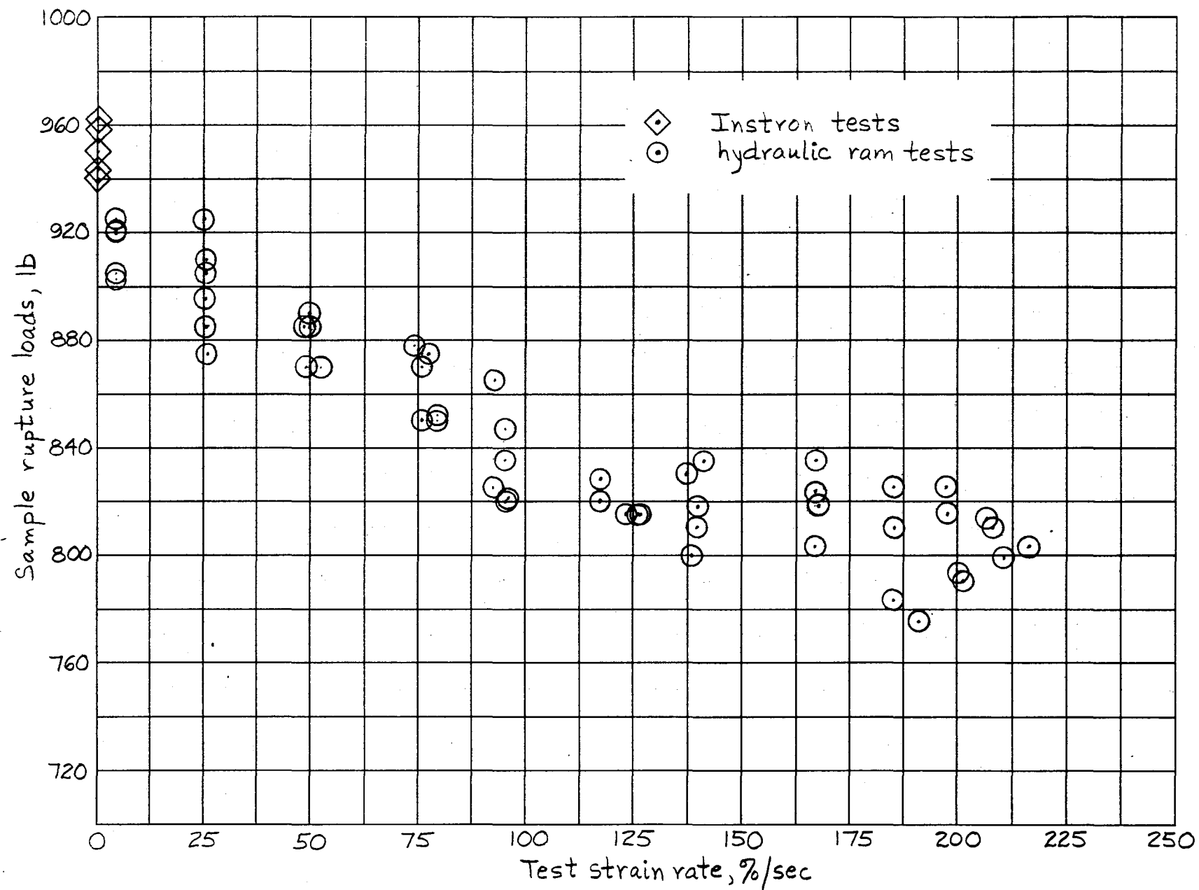
Figure 13.- Sample rupture loads as a function of strain rate at which samples were tested.
