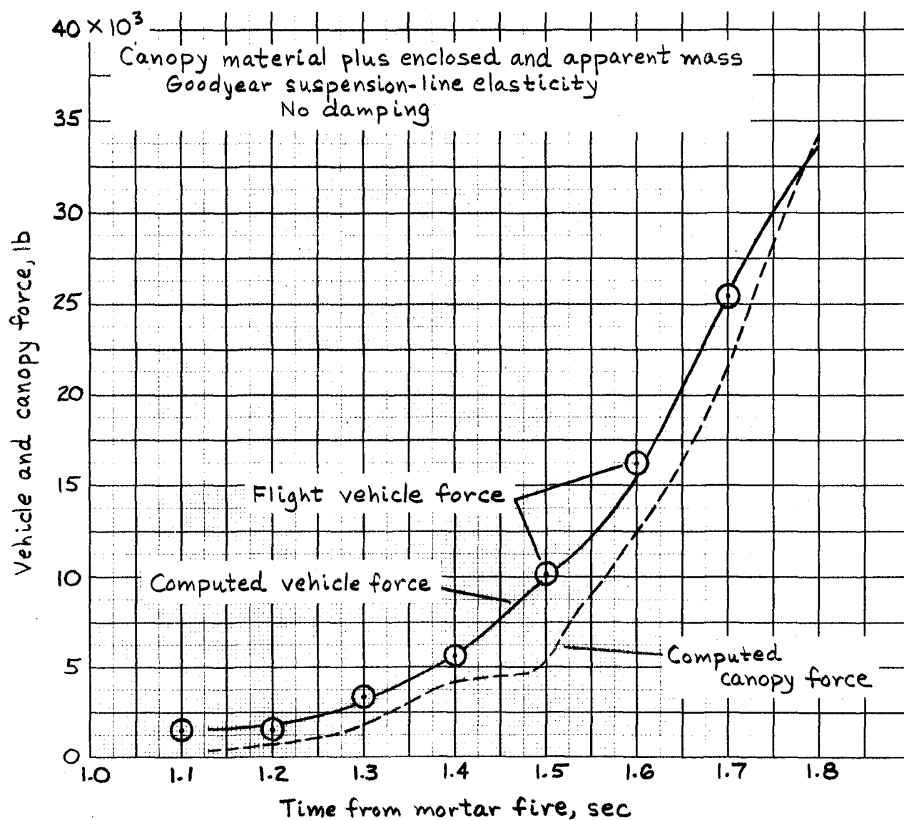
(b) Vehicle and canopy force histories
