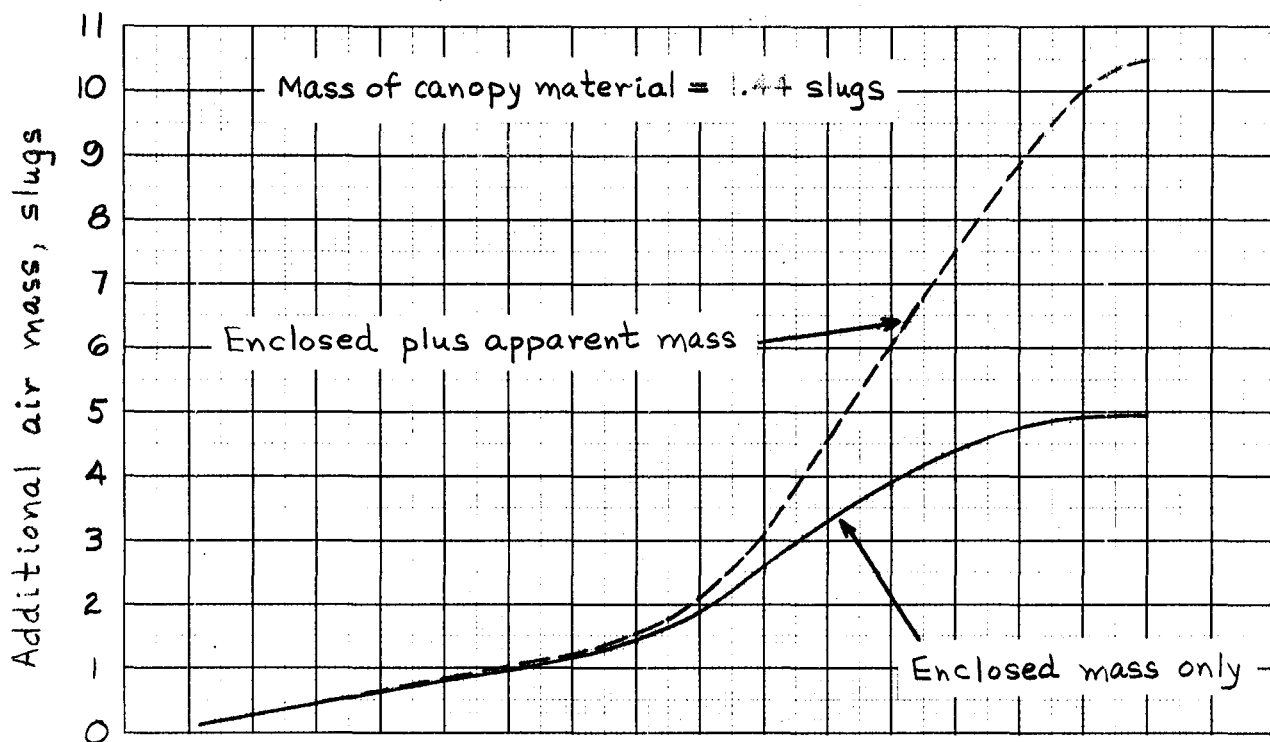
(a) Additional air mass history
