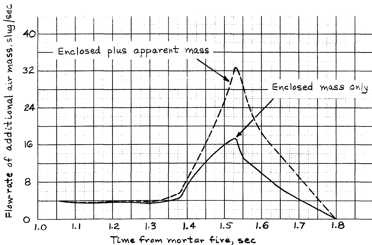
(b) Flow-rate of additional air mass
