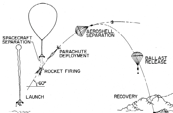
Figure 6. Balloon/rocket test method (from ref. 21).
