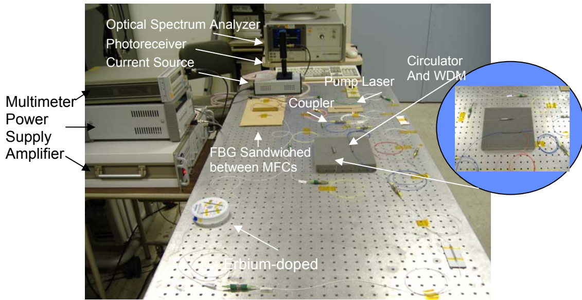
Figure 6: Experimental setup
