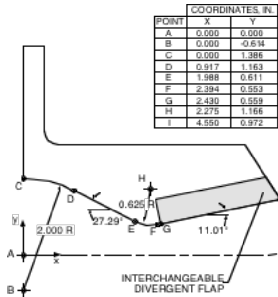
Figure 1 Sketch Showing Nozzle Geometric Details, ref. (3)
