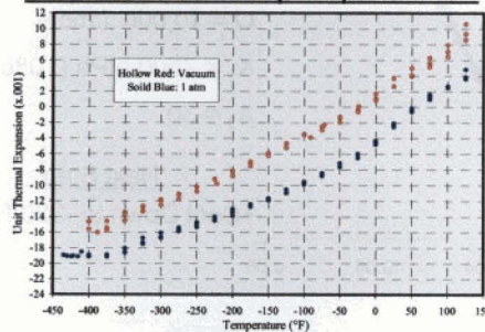
Figure 1. Comparison Thermal Expansion of BX 265 (3") in the 11 direction under Vacuum and at 1 atm, & 0.9 psi load
