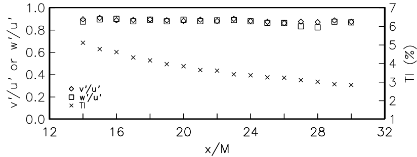
Figure 2.9. Turbulence intensity (TI) and isotropy ( v'/u' and w'/u' ) as a function of streamwise distance for Grid 0.
