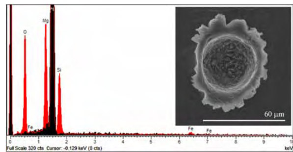
Fig. 1. Secondary electron image of the bowl-shaped crater preserved in foil C2086N and the 20 kV EDS spectra for the dominant Mg-silicate residue phase.
