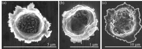
Fig. 2. Secondary electron images of the typical morphologies seen in impact craters preserved on the foil surfaces.
