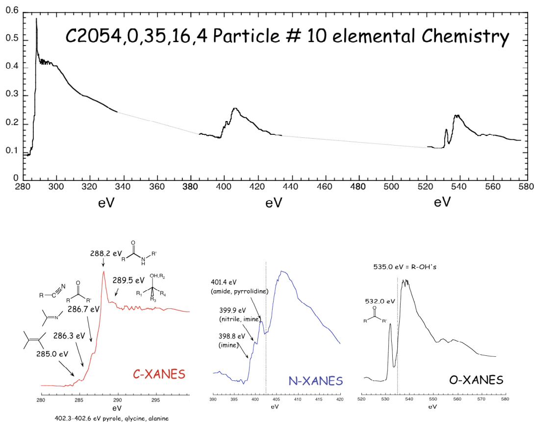
SUPPORTING FIGURE 6 – (Top) A XANES spectrum showing the C-, N-, and O- 1s ionization edges of Track 35, Grain 16, Mount 4 to scale. (Bottom) Expanded spectra of the individual C, N, and O edges showing the subfeatures associated with different chemical bonds.
