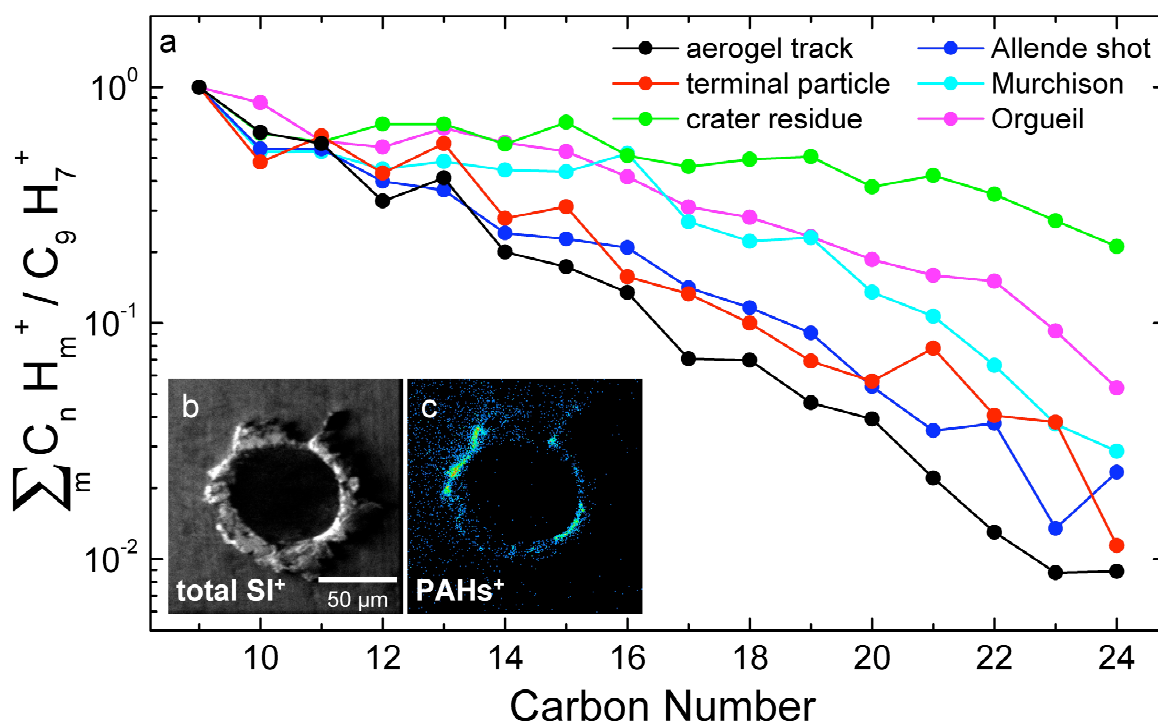
SUPPORTING FIGURE 2 – (a) Abundances of PAHs as a function of their number of carbon atoms relative to the abundance of \text{C}_9\text{H}_7^+ , the PAH fragment that typically shows the highest intensity in TOF-SIMS analysis. Analyzed samples include one dissected aerogel keystone with a particle track (Track 21), one terminal particle extracted from aerogel (Track 44, Grain 4), and one crater residue on aluminum foil (large crater from C2009N). For the latter, the corresponding PAH secondary ion distribution image (c) and a total secondary ion
