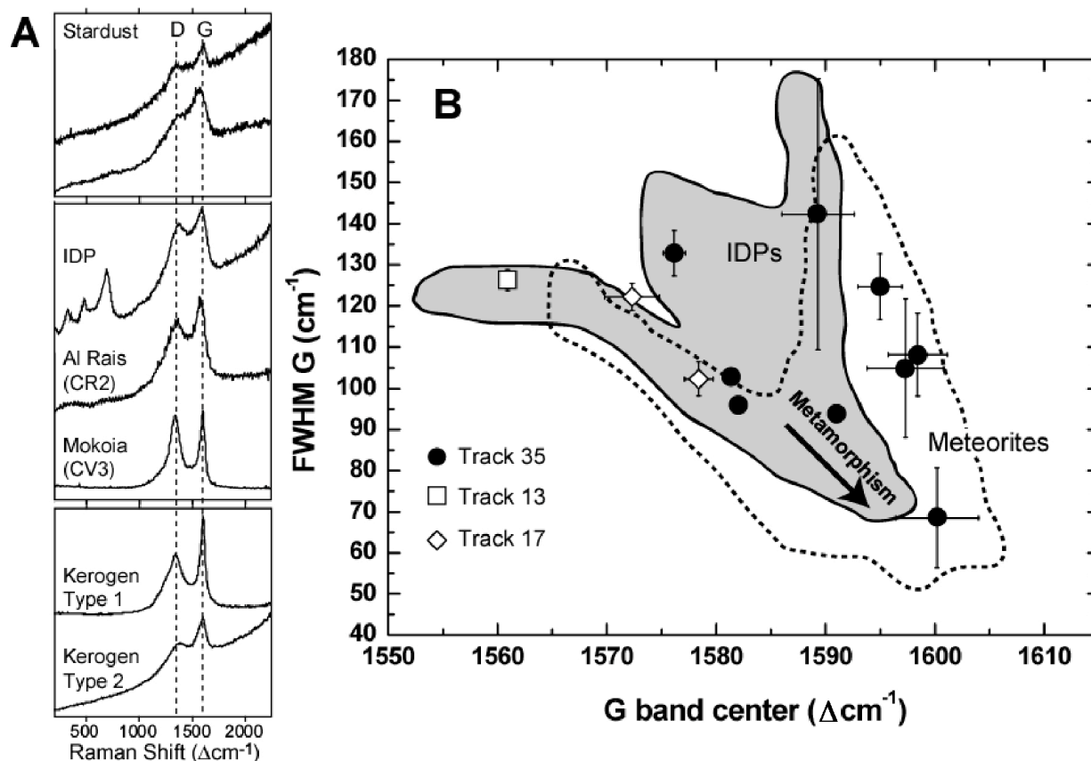
FIGURE 2 – A) Raman spectra of Stardust particles from Track 35, Grain 30 and Track 13, Grain 1 (top pair) compared to the spectra of organics from extraterrestrial and terrestrial carbonaceous materials with different fluorescence backgrounds. All exhibit D and G bands characteristic of disordered \text{sp}^2 -bonded carbon. The phyllosilicate bands below 1000\text{ cm}^{-1} in the IDP spectrum have not been seen in Stardust samples. B) The G band position and width (FWHM) of a material reflect its degree of thermal metamorphism and “structural ordering.” The boundaries show the range of values from over 40 chondritic meteorites and 40 IDPs analyzed in PET Raman laboratories (9,10,29,30). Analyzed Stardust particles span the entire range seen in IDPs and meteorites. Organics in highly thermally metamorphosed meteorites plot to the lower right. The presence of Stardust points in the upper left indicates that at least some of the cometary organics are very primitive and were captured with relatively little alteration. One Stardust sample shows an unusually low G band position (below 1570\text{ cm}^{-1} ), suggesting diamond-like carbon that has been amorphized, e.g., due to particle irradiation (31). One-sigma error bars represent measurement reproducibility and do not include estimates of possible inter-laboratory biases.
