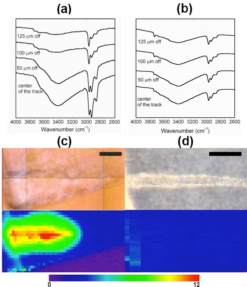
FIGURE 3 – IR transmittance spectra obtained along a line perpendicular to cometary impact tracks (a) Track 59 and (b) Track 61. In addition to aerogel features, the spectra of Track 59 (a) display peaks at 3322, 2968, 2923, 2855, and 1706 cm -1 (not shown) both inside the track and extending outward into the aerogel. (b) Track 61 exhibits only the aliphatic CH stretching feature dominated by the 2968 cm -1 peak and (Si-O) bands (not shown) characteristic of the flight aerogel. The optical images of the same tracks, with the corresponding maps displaying the intensity distribution of the 2923 cm -1 peak (-CH 2 -), are displayed in (c) and (d). The false color image scale shown at the bottom is used in both maps and the black scale bars corresponds to 100 μm. In both cases the entrance of the cometary particle is on the left hand side. The false color map in (c) shows an increase in intensity of the 2923 cm -1 -CH 2 - peak in and near the track. The distributions of other organics peaks are similar. In contrast, the second track shown in Fig. 4d shows almost uniform distribution of the peak area centered at 2923 cm -1 , i.e., the track shows only the features of aerogel.
