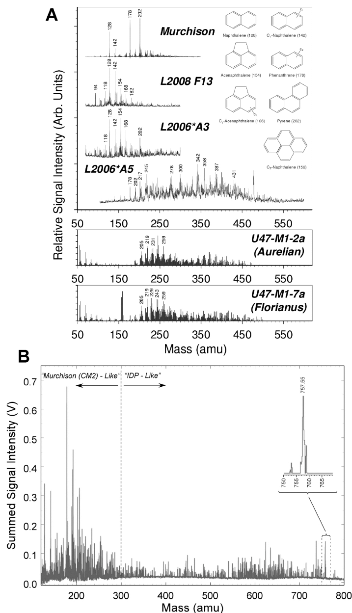
FIGURE 1 – (A) The L 2 MS spectra of the carbonaceous chondrite Murchison and 5 stratospheric IDPs. The meteorite and some IDPs show relatively simple populations dominated by small PAHs, but the spectra of some IDPs extend to higher masses, indicating a more complex distribution of PAHs. (B) The L 2 MS spectrum of Stardust sample Track 16, is similar to the lower IDP spectra in 1A. The higher mass envelope of peaks above 300 amu for the Stardust sample probably reflects increased polymerization during impact with the aerogel compared to the more benign atmospheric deceleration experienced by most stratospheric IDPs.
