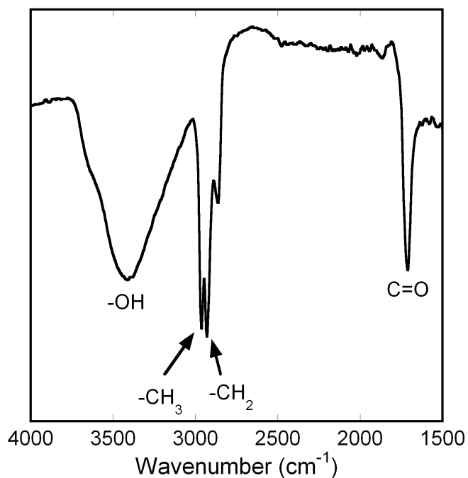
SUPPORTING FIGURE 4 – The 4000–1500 \text{cm}^{-1} infrared spectrum of a section of Track 59. Absorption features can be seen near 3322 \text{cm}^{-1} ( -\text{OH} ), 2968 \text{cm}^{-1} ( -\text{CH}_3 ), 2923 \text{cm}^{-1} ( -\text{CH}_2- ), 2855 \text{cm}^{-1} ( -\text{CH}_3 and -\text{CH}_2- ), and 1706 \text{cm}^{-1} ( \text{C}=\text{O} ). All these features except the 1706 \text{cm}^{-1} \text{C}=\text{O} band contain some contributions from aerogel.
