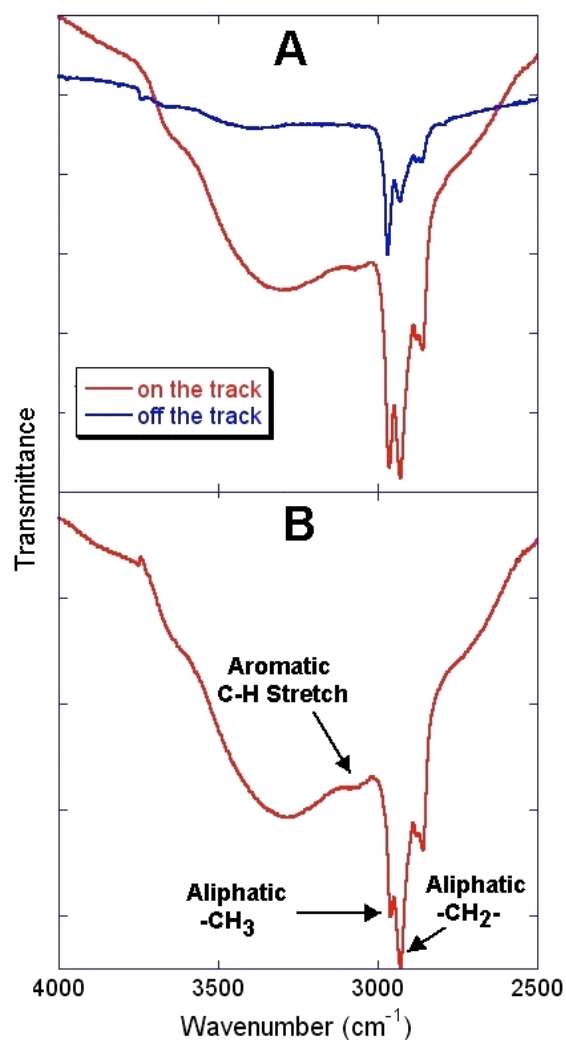
SUPPORTING FIGURE 5 – (A) The 4000-2500 cm -1 spectrum from an aerogel keystone (Track 58) on a track (red line) and far from the track (blue line). The aerogel spectrum can be scaled using an absorption feature due solely to aerogel and subtracted from the track spectrum. The residual absorption (B) is then dominated by new, non-aerogel material associated with the track dominated by a broad feature near 3300 cm -1 (-OH) and narrower features near 3065 cm -1 (aromatic CH stretch, weak), 2968 cm -1 (-CH 3 asymmetric stretch), 2923 cm -1 (-CH 2 - asymmetric stretch), and 2855 cm -1 (symmetric -CH 3 and -CH 2 - stretches).
