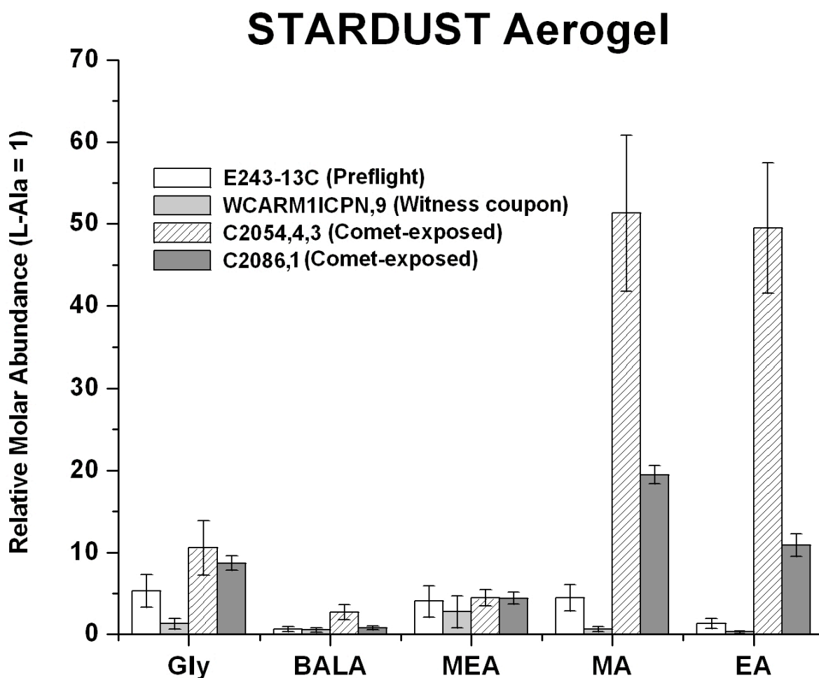
SUPPORTING FIGURE 8 - A comparison of the relative molar abundances (L-Ala = 1) of glycine (Gly), \beta -alanine (BALA), ethanolamine (MEA), methylamine (MA), and ethylamine (EA) in the acid-hydrolyzed hot-water extracts of Stardust aerogel. The high relative abundances of MA, EA, and glycine in comet-exposed aerogel samples C2054,4 (Piece 3) and C2086,1 compared to the preflight (E243-13C) and witness coupon (WCARM1ICPN,9) aerogel samples suggest a cometary origin for these amines.
