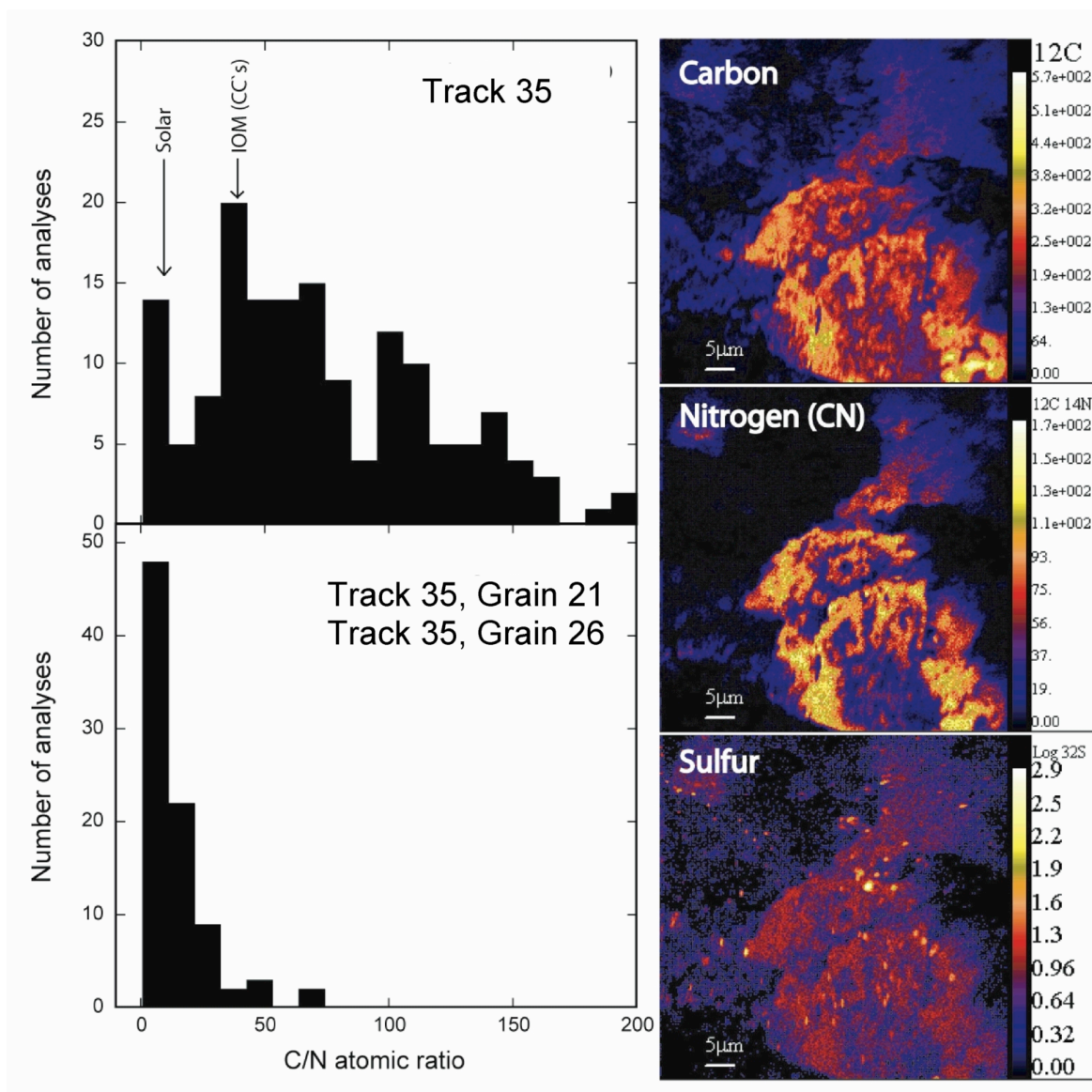
FIGURE 5 - Distribution of C and N. Left column : Histograms of C/N ratios in organics in three different Stardust samples. One sample (top) shows a large spread in C/N, whereas two samples (bottom) have organics characterized by low C/N ratios, consistent with the presence of volatile organic molecules such as HCN, or their polymer counterparts. Right column : NanoSIMS images of the distribution of C, N, and S in a region of an aerogel sample from along Track 35 containing cometary materials. The intensity of the signal increases from blue, to red, to bright yellow. C, N, and S distributions are clearly correlated, although significant variations in their relative abundances are observed. S is also present in a population of ‘hotspots’ that likely indicate the presence of sulfides. The color scale in the S map is logarithmic, in order to show the large difference in S count rates between the organics and the sulfides. The distribution of C and N is qualitatively similar in particles both with and without ^{15}\text{N} excesses. The location labelled IOM (CCs) in the upper left panel denotes the C/N ratio of the insoluble organic matter found in carbonaceous chondrites.
