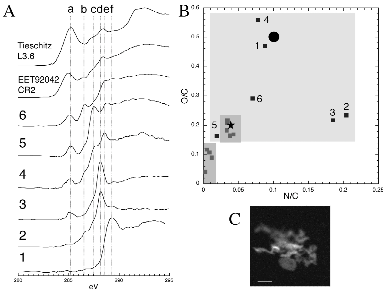
FIGURE 4 - A ) C-XANES spectra of six thin section samples (1-6) compared to spectra of primitive (EET92042, CR2) and moderately processed (Tieschitz, L3.6) chondritic organic matter. Samples are 1 , Track 16, Grain 1, Mount 10; 2 , Track 35, Grain 16, Mount 4 ; 3 , Track 22, Grain 1, Mount 5; 4 , Track 35, Grain 32, Mount 10; 5 , Track 35, Grain 32, Mount 8 ; and 6 , (Track 13, Grain, Mount 5) (samples 4 and 5 are different thin sections of the same grain). Specific organic functional groups are highlighted (dashed lines a-f); a) (C=C at \sim 285.2 eV), b) (C=C-O at \sim 286.5 eV), c) (C=O at \sim 287.5 eV), d) (N-C=O at 288.2 eV), e) (O-C=O at 288.6 eV), and f) (C-O at 289.5 eV). Sample chemistry ranges enormously, with sp^2 bonded carbon varying from non-existent in 1 to modest in samples 5 and 6 (relative to chondritic organic matter). B ) Atomic O/C and N/C for samples 1-6 derived from C,N,O-XANES analysis (black squares) are compared to chondritic organic matter (grey squares, where the higher values corresponds to petrologic type 1 and 2 and the lower values are type 3). Average values for Comet Halley particles and stratospheric IDPs (17) are marked by a black star and a large solid circle, respectively. C ) An example of a sample thin section from Track 35, Grain 32, Mount 8 (spectrum 5 ) revealed as a high resolution (40 nm pixel size) STXM optical density image (scale bar = 1 \mu\text{m} ) on the carbon 1s absorption edge.
