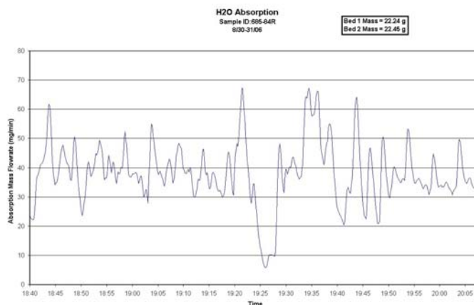
Figure 11. Water adsorption.
