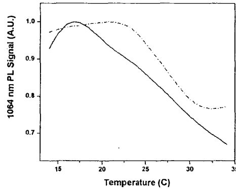
Fig. 3. 1064 nm PL vs. diode temperature in 2-passed (solid) and 4-passed (dashed) pump mode. The 2-pass pumped configuration produces a peak inversion around 17°C while the 4-pass method is broader in \Delta T and peaks around 21°C.
