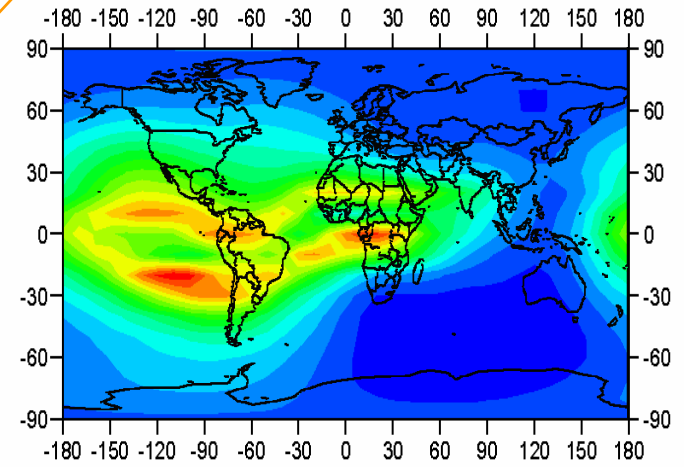
Plasma Density (#/m^3)
