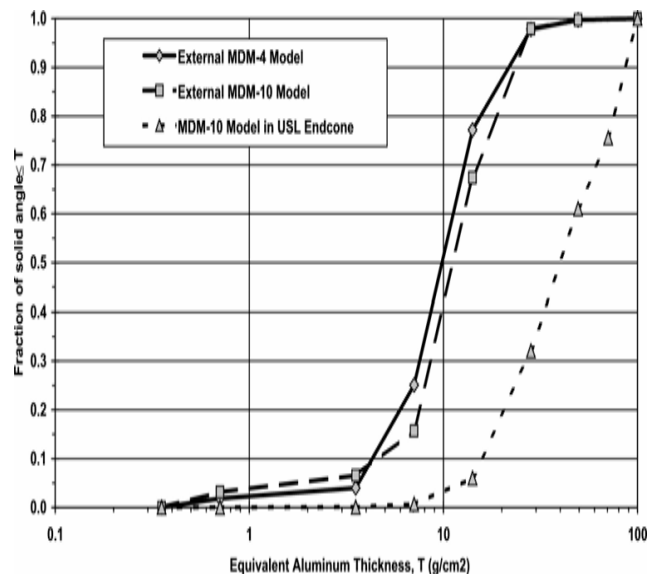
MDM 1Mx4 DRAM Structural Shielding Distributions.
