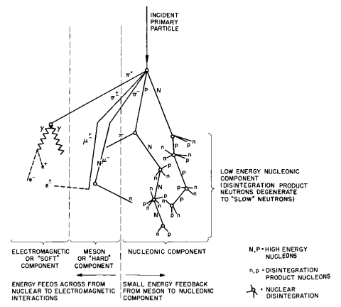
Schematic Diagram of Cosmic Ray Shower
