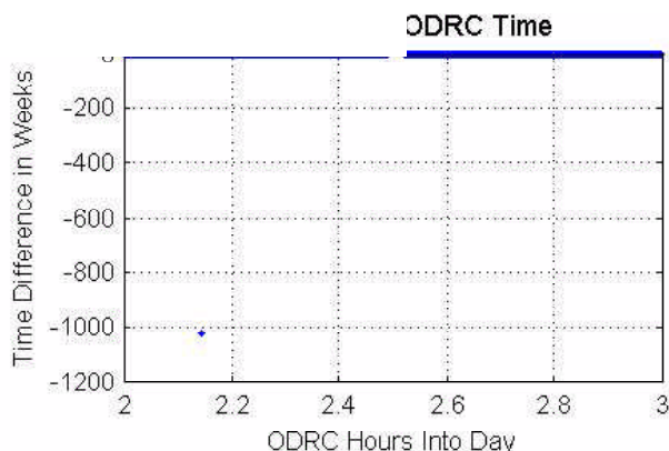
Fig. 5 GPS/INS time compared to ODRC time.
