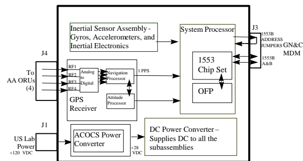
Fig. 1 Block diagram of ISS GPS/INS.
