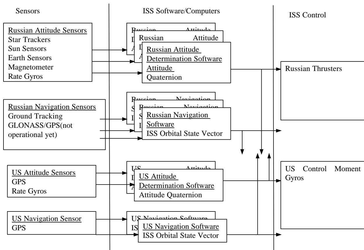
Fig. 3 ISS GNC overview.
