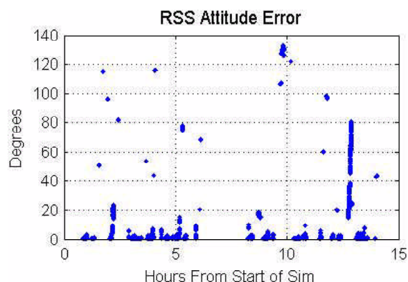
Fig. 8 Attitude error in degrees for orbit simulation with ISS multipath environment – original GPS attitude firmware.
