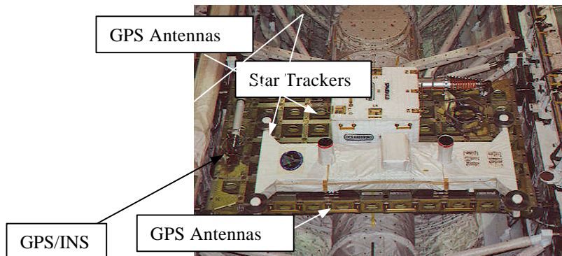
Fig. 4 Space Shuttle payload bay arrangement for STS-101 and STS-106.
