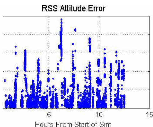
Fig. 9 Attitude error in degrees for orbit simulation with ISS multipath environment – new GPS attitude firmware.
