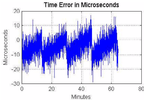
Fig. 6 Time error in microseconds when tracking at least 4 satellites.
