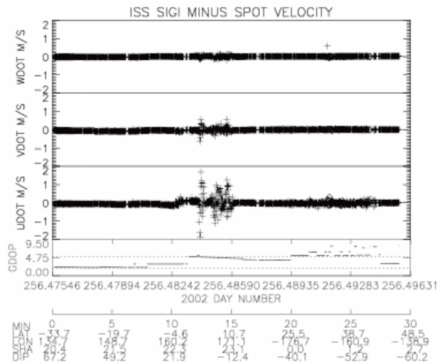
Fig. 11 GPS/INS velocity noise as compared to ground filter.
