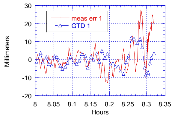
Fig. 13 Measured differential carrier phase errors compared to GTD predicted differential carrier phase errors for SV24 and antennas 1 and 2 from STS-77 data.
