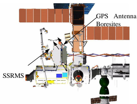
Fig. 14 SSRMS Parked over GPS antenna array.
