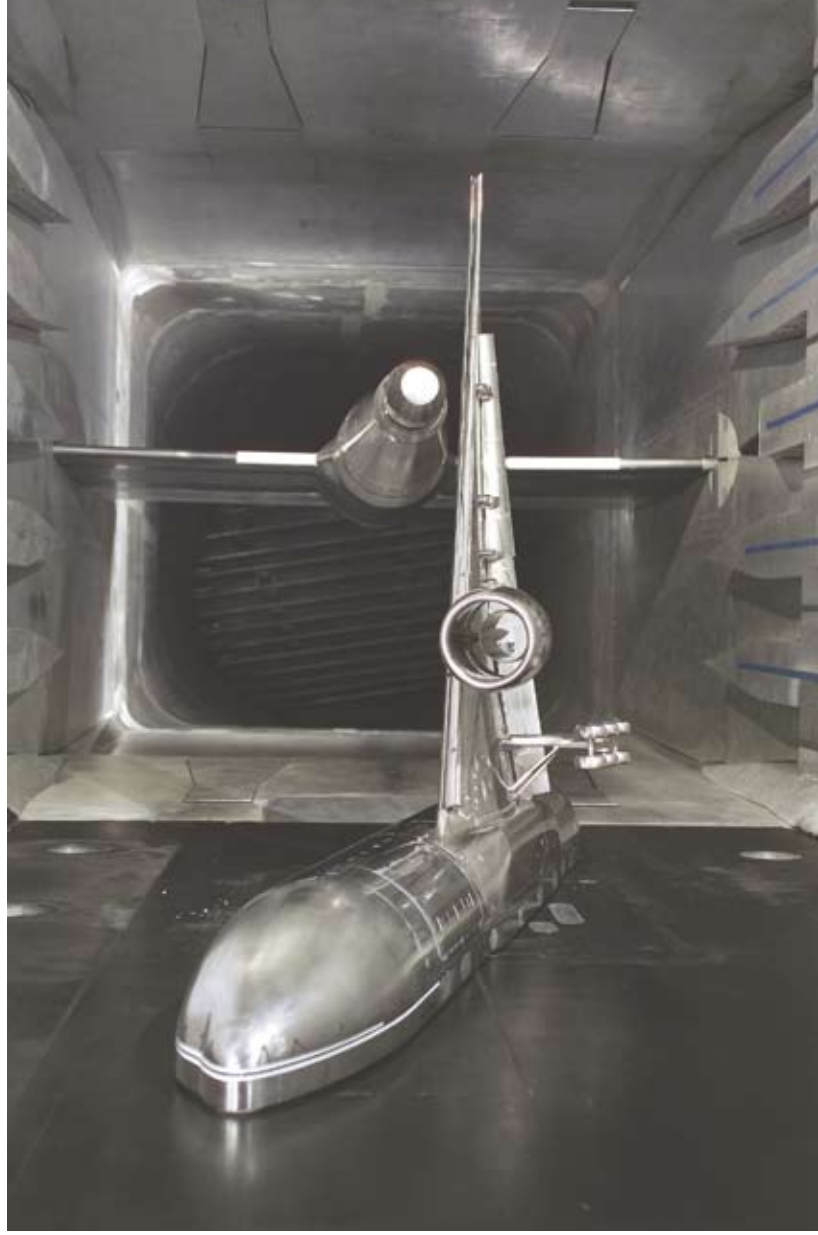
Wing trailing edge design concepts for Boeing's new 787 aircraft are being tested on a 5.2-percent scale 777 semi-span model inside Langley Research Center's National Transonic Facility.
