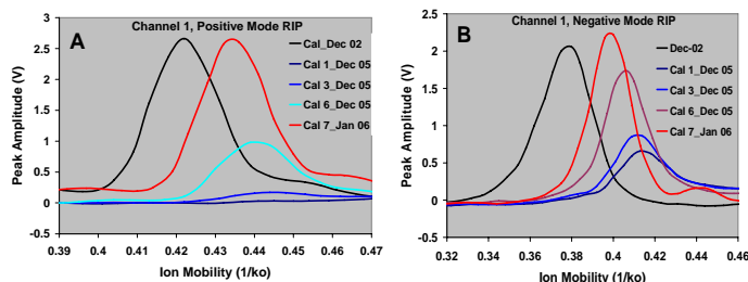
Figure 3 Channel 1 runs for December 2005 and the first run in January 2006 A) Positive RIP and B) Negative RIP
