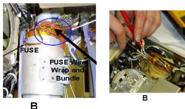
Figure 1 Fuse position and testing A) IMS cell B) preconcentrator
