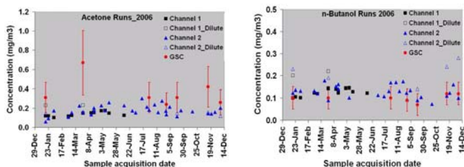
Figure 5 Plots of 2006 VOA data for acetone and n-butanol
