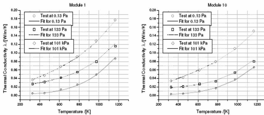
Figure 2. Local Thermal Conductivity of Modules 1 and 10 – Comparison between Model and Test Results
