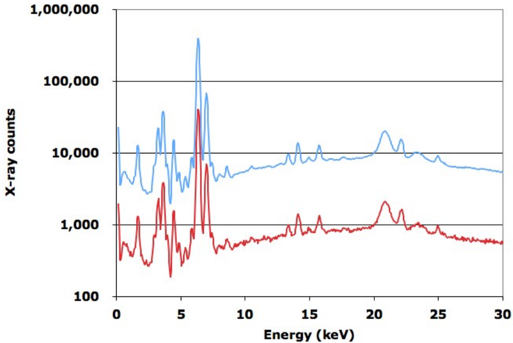
Figure 2. Spectra from borehole instrument. Upper curve is 1000 seconds data collection time. and lower curve is 100 seconds.
