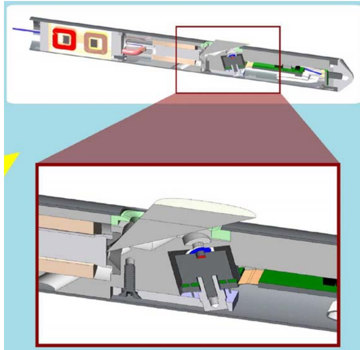
Figure 1. Engineering drawing of the final design of the downhole assembly. The enlarged area shows the X-ray tube and the detector. See text for details.
