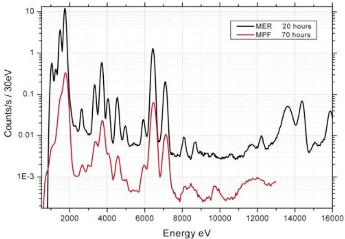
Figure 3. Spectra from the APXS instrument. Reproduced from reference 3.
