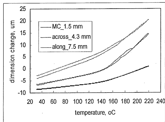
Figure 10. Thermo-mechanical characteristics of a chip tantalum 15 \mu\text{F}/50\text{ V} capacitor.
