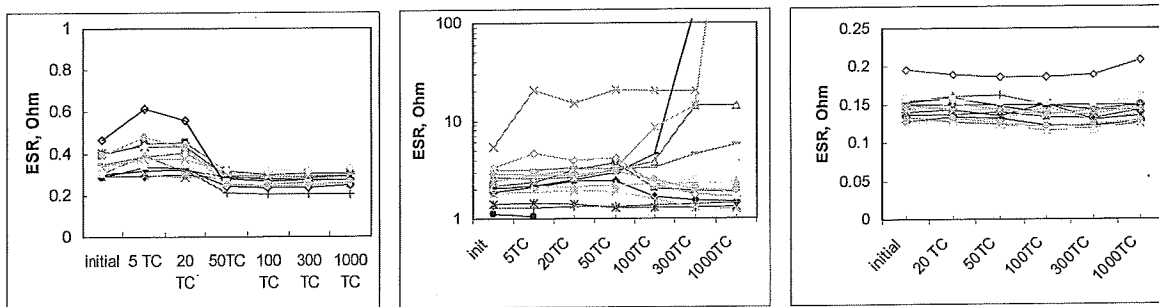
a) 10\ \mu\text{F}/25\ \text{V} , \text{ESR}_{\text{max}} = 1.4 b) 2.2\ \mu\text{F}/10\ \text{V} , \text{ESR}_{\text{max}} = 8 c) 22\ \mu\text{F}/20\ \text{V} , \text{ESR}_{\text{max}} = 0.9 Figure 3. Variation of ESR in military-grade parts during temperature cycling in the range from -65^{\circ}\text{C} to +125^{\circ}\text{C} .
