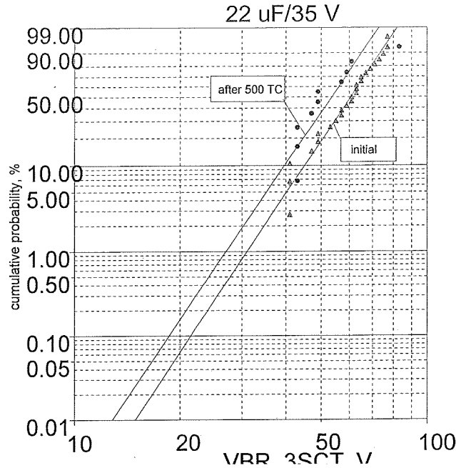
Figure 9. Effect of temperature cycling on distributions of breakdown failures during step stress surge current testing of 22 \mu\text{F}/35\text{ V} parts.
