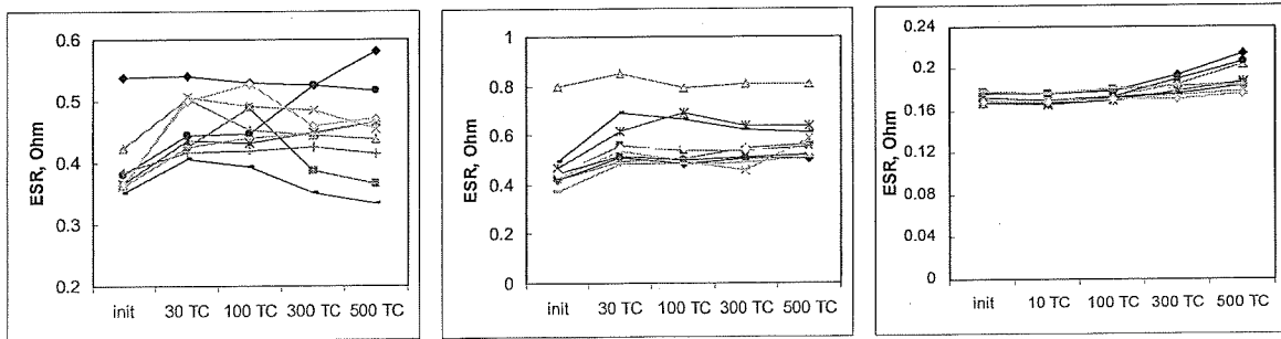
d) 10\ \mu\text{F}/25\ \text{V} , \text{ESR}_{\text{max}} = 2.5 e) 10\ \mu\text{F}/50\ \text{V} , \text{ESR}_{\text{max}} = 1.6 f) 15\ \mu\text{F}/50\ \text{V} , gr. II, \text{ESR}_{\text{max}} = 0.3 Figure 4. Variation of ESR in commercial parts during temperature cycling in the range from -65^{\circ}\text{C} to +150^{\circ}\text{C} .
