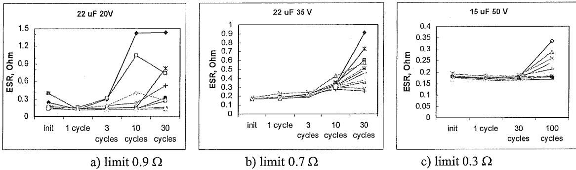
Figure 14. Effect of high-temperature cycles on ESR. Captions indicate specified ESR limits for the parts.
