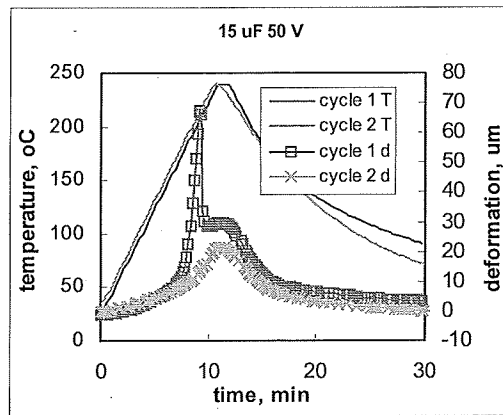
Figure 11. A deformation spike during the first heating cycle on a 15\text{ }\mu\text{F}/50\text{ V} capacitor. Unmarked lines show temperature variations, and marked lines show deformation of the part.
