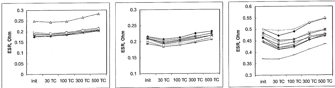
a) 15\ \mu\text{F}/50\ \text{V} , gr. I, \text{ESR}_{\text{max}} = 0.3 b) 22\ \mu\text{F}/35\ \text{V} , \text{ESR}_{\text{max}} = 0.7 c) 2.2\ \mu\text{F}/35\ \text{V} , \text{ESR}_{\text{max}} = 4
