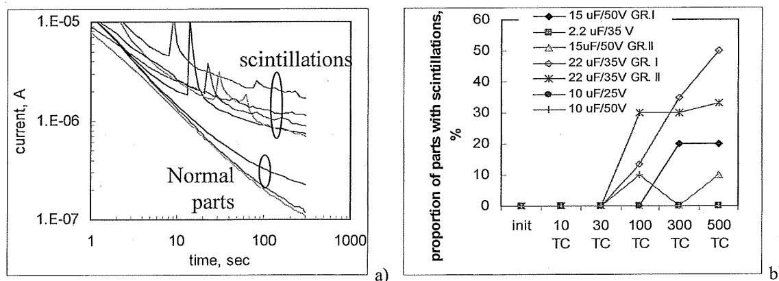
Figure 7. I-t characteristics for the 22 \mu F/35 V capacitors showing normal parts and parts with scintillations (a) and variation of the proportion of devices with scintillations with the number of TC (b).
