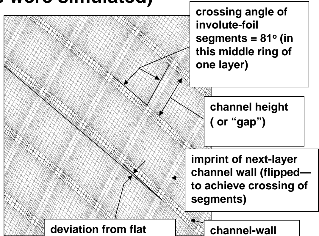
Enlarged area from middle of periodic sector—two layers of involute foils with grids—basis of simplifications for straight-channel-layer approx.
