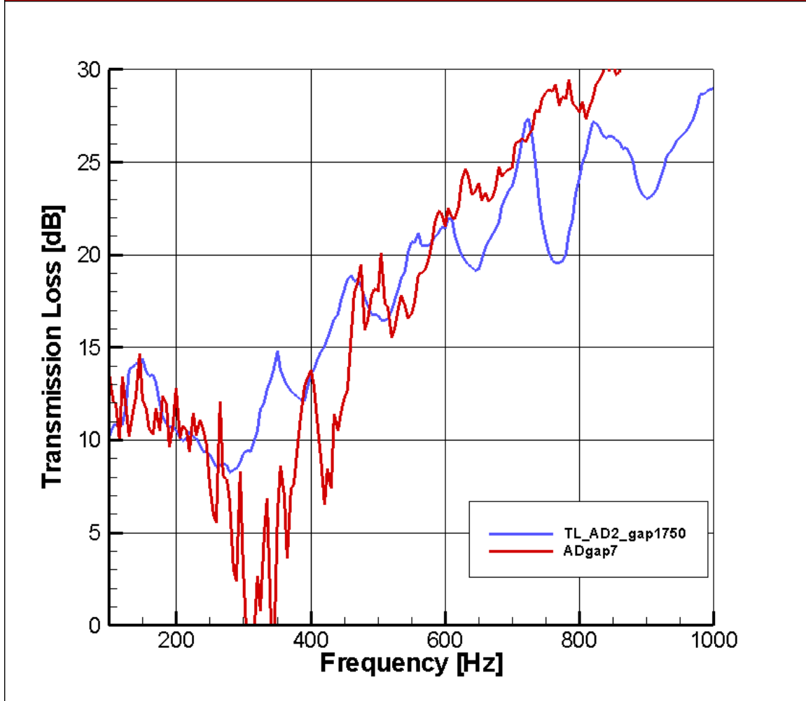
Figure 19. Experimental (TL_AD2_gap1750) and predicted (ADgap7) transmission loss of a double wall configuration of 0.020 and 0.032 inch thick aluminum panels separated by a distance of 1.75 inches.
