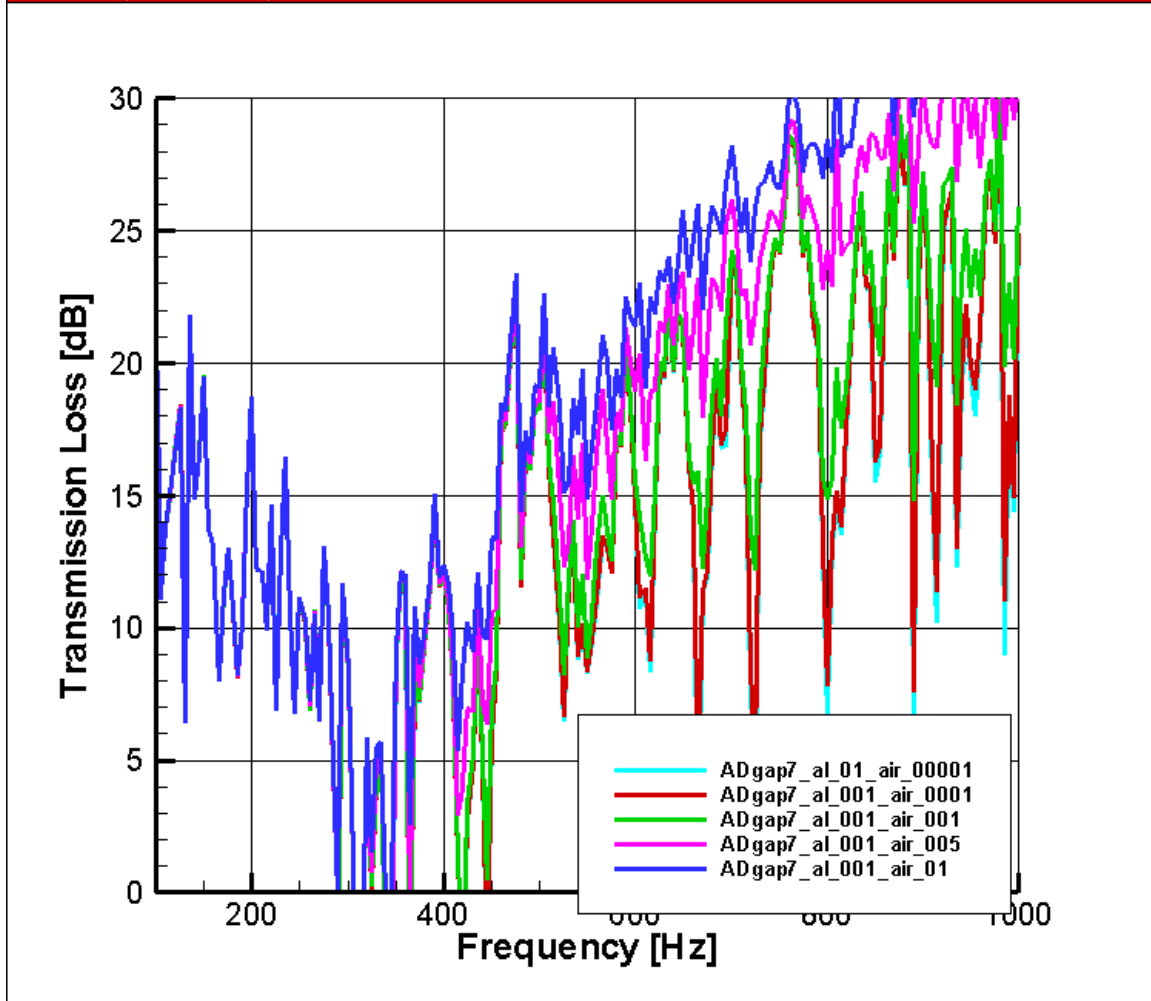
Figure 48. Transmission loss of a double wall configuration with 0.020 inch and 0.032 inch thick aluminum panels separated by an air gap of 1.75 inches having air damping coefficients of 0.0001, 0.001, 0.01, 0.05 and 0.1. The damping factor of the aluminum panels was 0.01 except for the air damping coefficient of 0.0001 for which case the aluminum panel damping coefficient equaled 0.1 Each transmission loss curve was predicted for one set of random sound incident input parameters.
