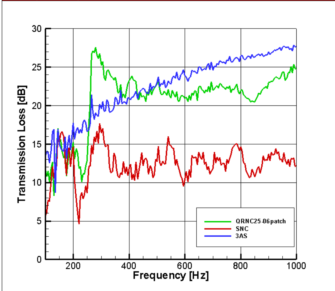
Figure 38. Predicted transmission loss of the honeycomb panel with twenty-five, 6 by 6 inch, quarter inch thick recessed cores with a 0.016 inch thick aluminum patch applied to the recessed cores (QRNC25-06) the transmission loss of the base nomex core honeycomb panel (SNC) and a single, 0.05871 inch thick aluminum panel (3AS) with the same total mass as the base honeycomb panel. The mass of the QRNC25-06patch panel is 5.1% more than the SNC or 3AS panels.
