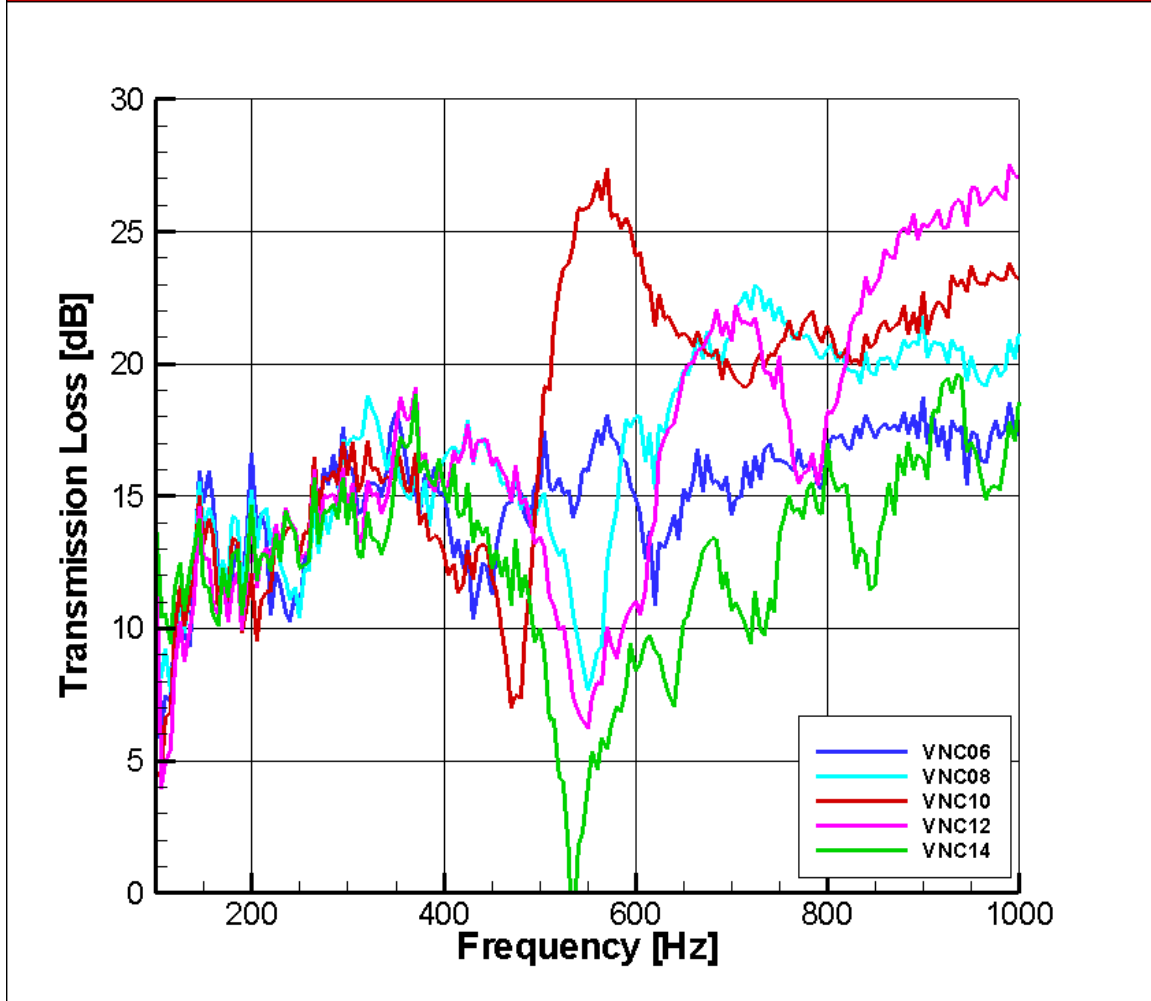
Figure 27. Predicted transmission loss of nomex core honeycomb panels having nine 6 by 6 (VNC06), 8 by 8 (VNC08), 10 by 10 (VNC10), 12 by 12 (VNC12), and 14 by 14 (VNC14) inch voids.
