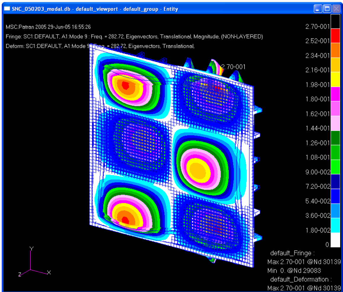
Figure A49. Modal analysis of a nomex core honeycomb panel, Mode 9.
