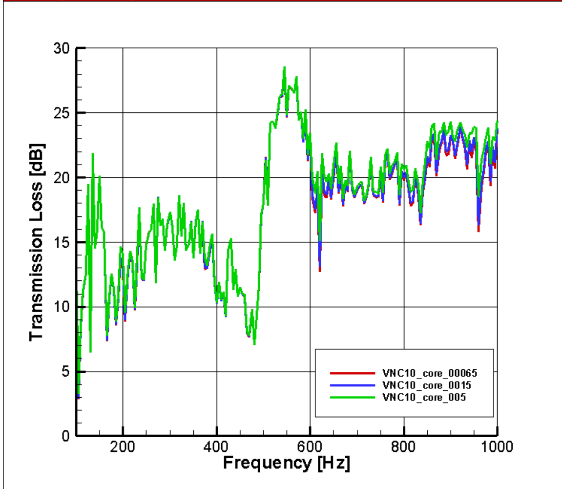
Figure 50. Transmission loss of honeycomb panels with nine 10 by 10 inch voids predicted for nomex cores with damping coefficients of 0.0065, 0.015 and 0.05. The core material properties are listed in Table 1. Each transmission loss curve was predicted for one set of random sound incident input parameters.
