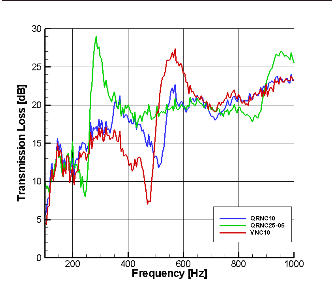
Figure 30. Predicted transmission loss of the honeycomb panels with nine 10 by 10 inch voids (VNC10), nine 10 by 10, quarter-inch recessed cores (QRNC10), and twenty-five 6 by 6, quarter-inch recessed cores (QRNC25-06).
