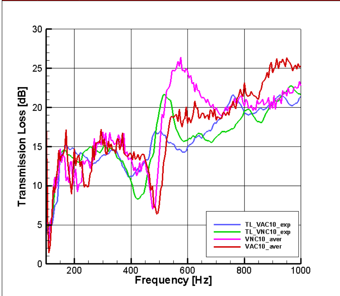
Figure 40. Experimental transmission loss of aluminum (TL_VAC10_exp) and nomex core honeycomb (TL_VNC10_exp) panels with nine 10 by 10 inch voids compared with predicted transmission loss for of aluminum (VAC10_aver) and nomex core honeycomb (VNC10_aver) panels with nine 10 by 10 inch voids.
