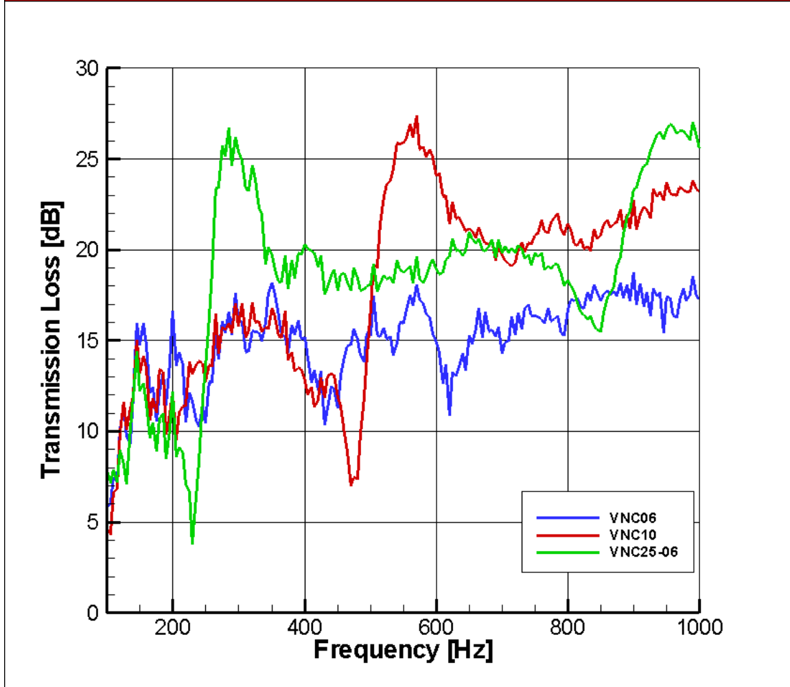
Figure 29. Predicted transmission loss of nomex core honeycomb panels having nine 6 by 6 (VNC06), nine 10 by 10 (VNC10), and twenty-five 6 by 6 (VNC25-06) inch voids.
