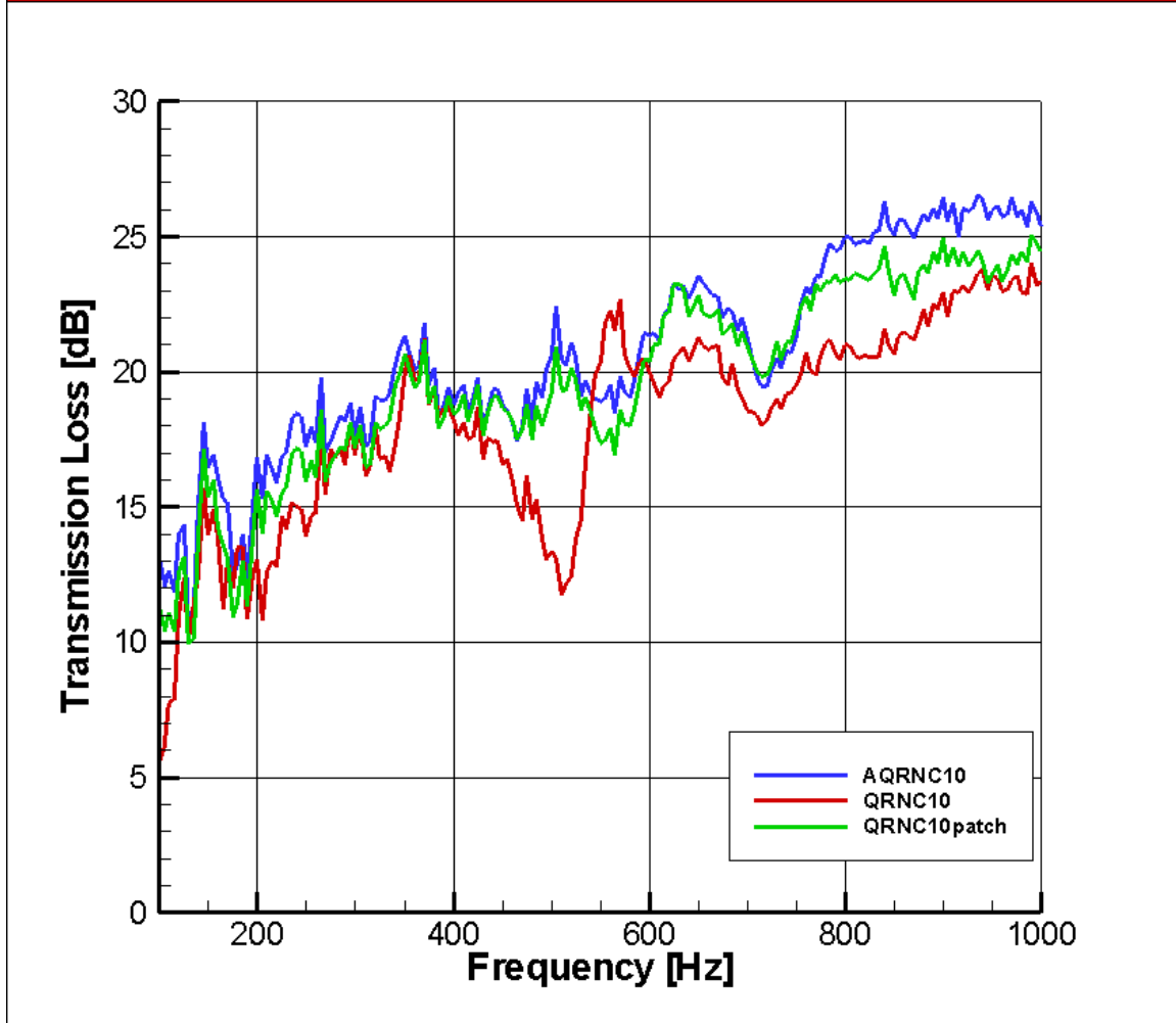
Figure 25. Predicted transmission loss of the honeycomb panels with quarter inch thick recessed cores without material covering the recessed core (QRNC10), with a 0.016 inch thick, 45 by 45 inch aluminum panel covering the recessed cores (AQRNC10) and with a 0.016 inch thick aluminum patch applied to the recessed cores (QRNC10patch).
