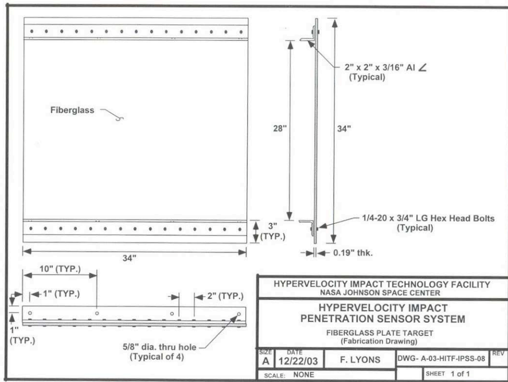
Figure 23: Fiberglass Article Target C-2 Drawing
