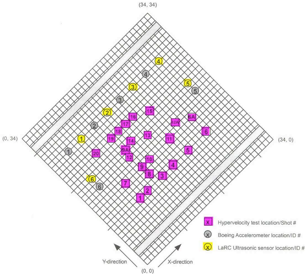
Figure 5: C-2 Diagram of Sensor and Impact Locations. Front View.
