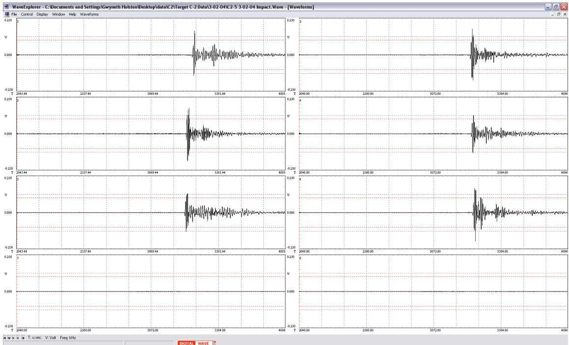
Figure 28: C-2 Shot #5 Impact Waveform
