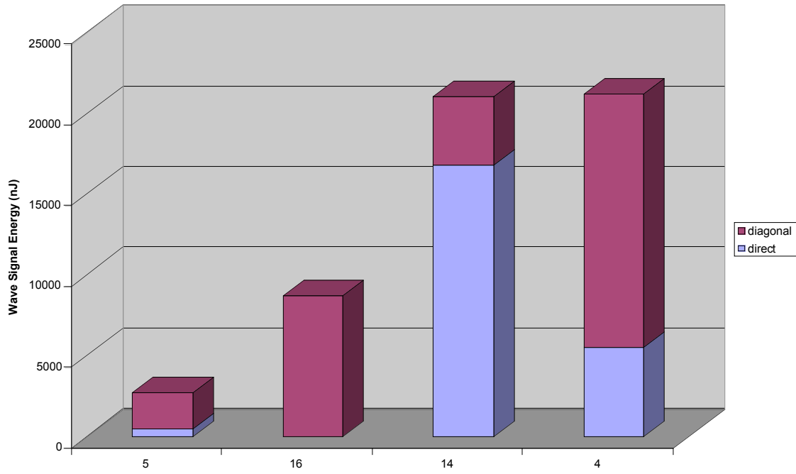
Figure 22: C-2 Diagonal and Direct W.S.E. for shots #5, 16, 14, and 4
