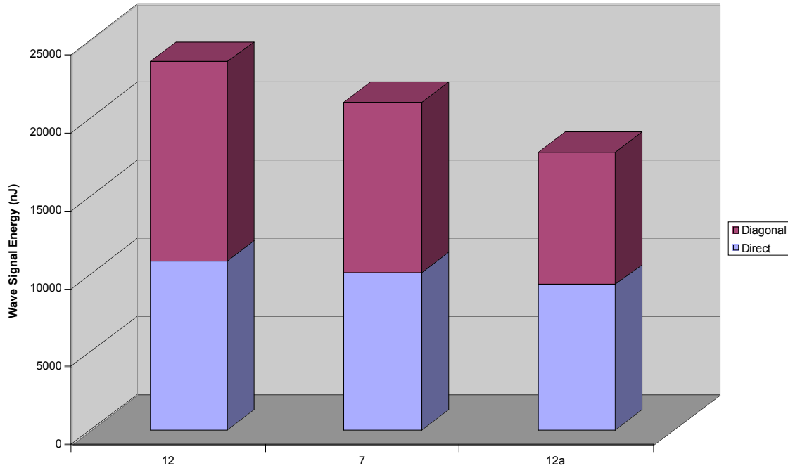
Figure 21: C-2 Diagonal and Direct W.S.E. for Shots #12, 7, and 12a
