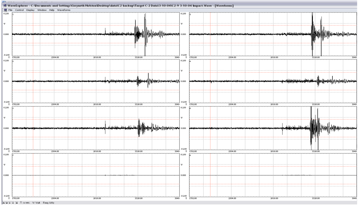
Figure 33: C-2 Shot #9 Impact Waveform
