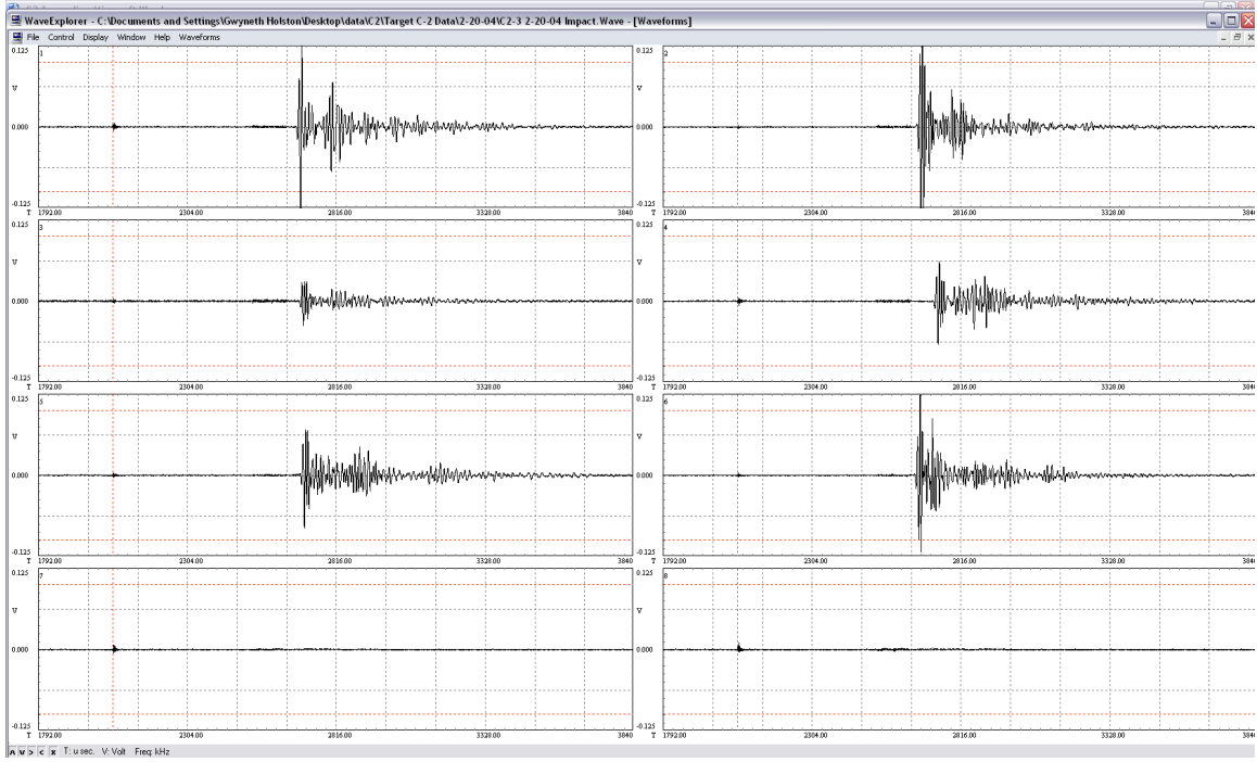
Figure 26: C-2 Shot #3 Impact Waveform
