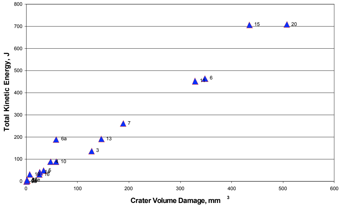
Figure 14: C-2 Total Kinetic Energy vs. Crater Volume Damage
