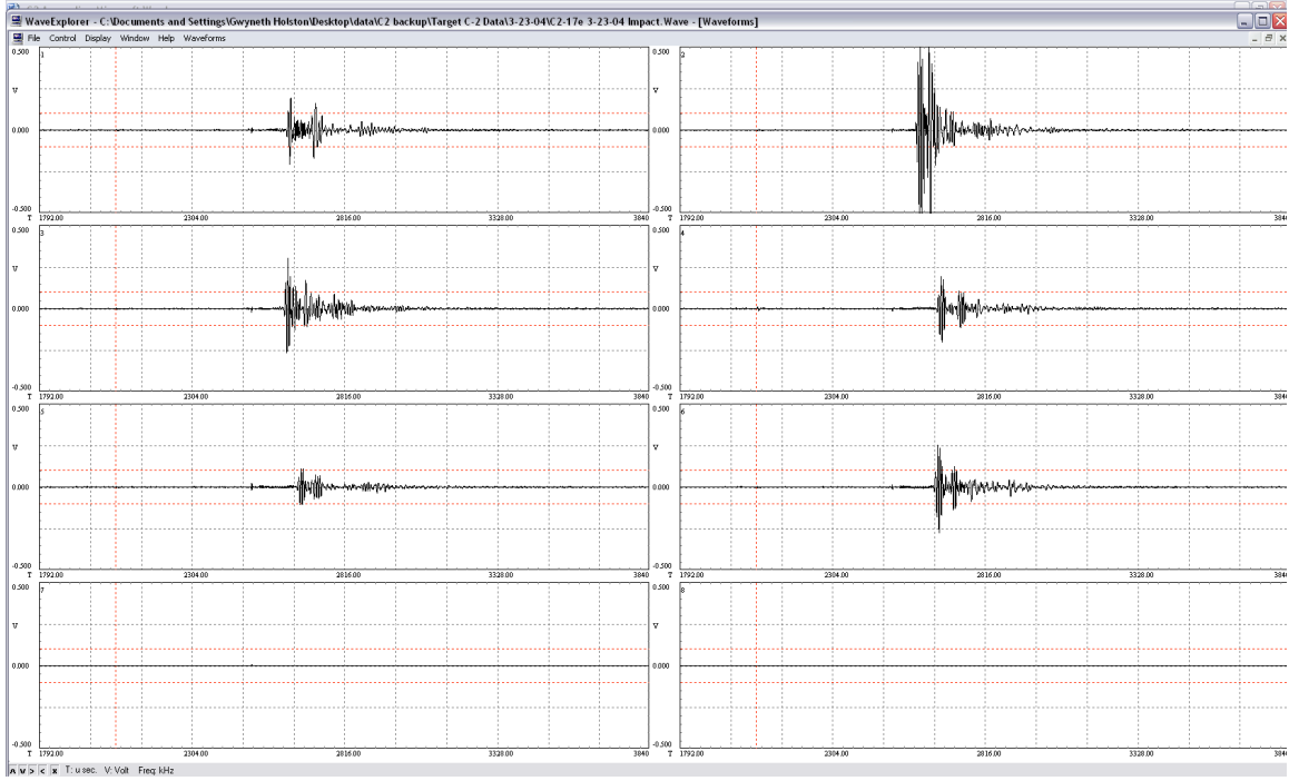
Figure 43: C-2 Shot #17e Impact Waveform
