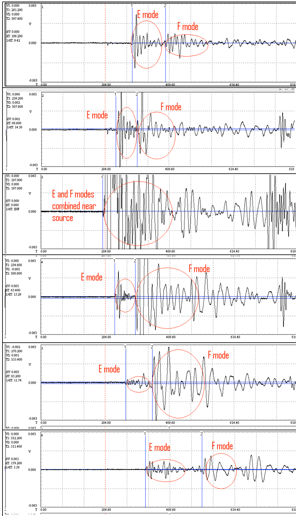
Figure 18: C-2 Lead Break at Sensor 3 for Shot #2 Pretest
