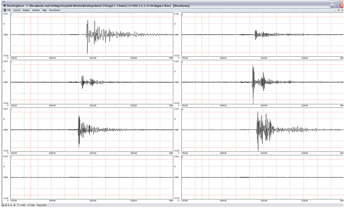
Figure 29: C-2 Shot #6 Impact Waveform
