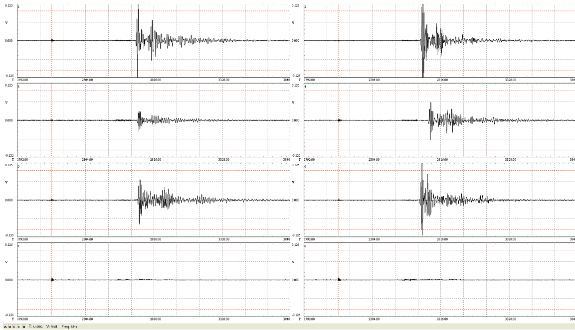
Figure 7: C-2 Impact Signal for Shot #3
