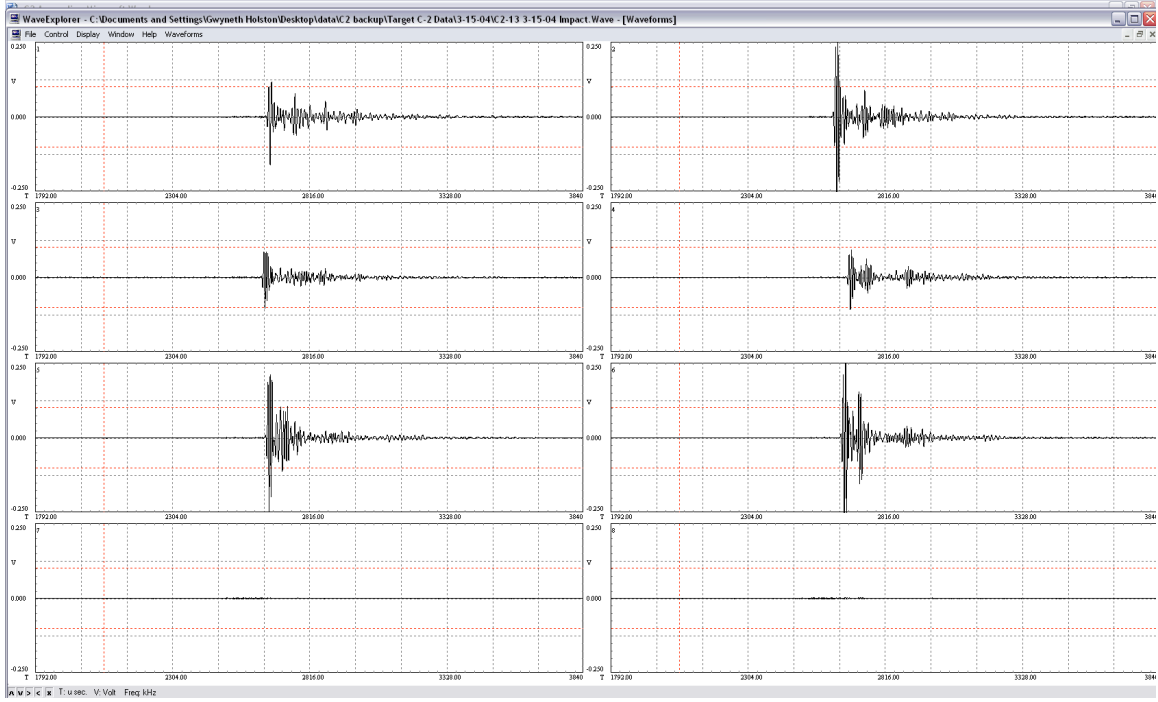
Figure 39: C-2 Shot #13 Impact Waveform
