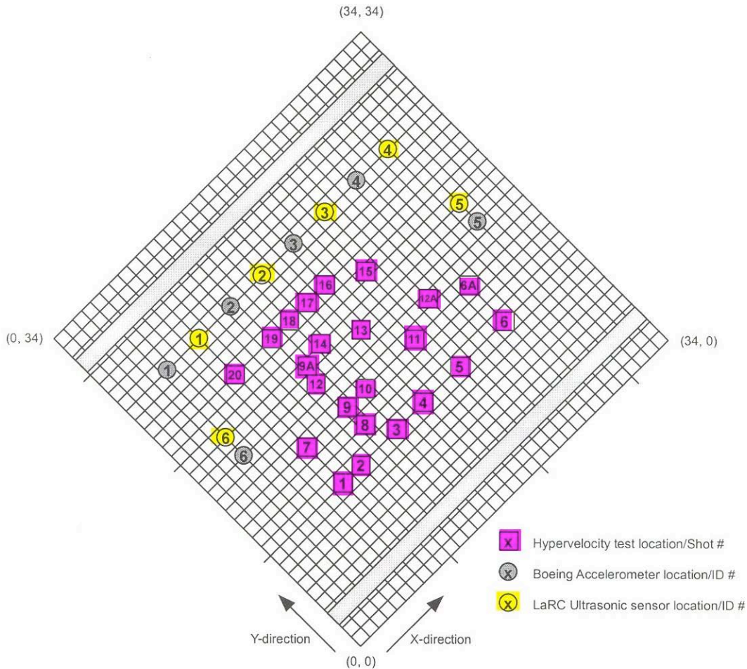
Figure 19: C-2 Diagram of Sensor and Impact Locations. Front View. (Repeat of Figure 5) Acoustic emission sensors are highlighted in yellow with the following coordinates: #1 (8, 26), #2 (15, 26), #3 (22, 26), #4 (29, 26), #5 (30, 19), #6 (4, 19).
