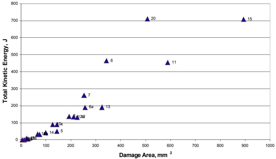
Figure 12: C-2 Total Kinetic Energy vs. Fiber Damage Area
