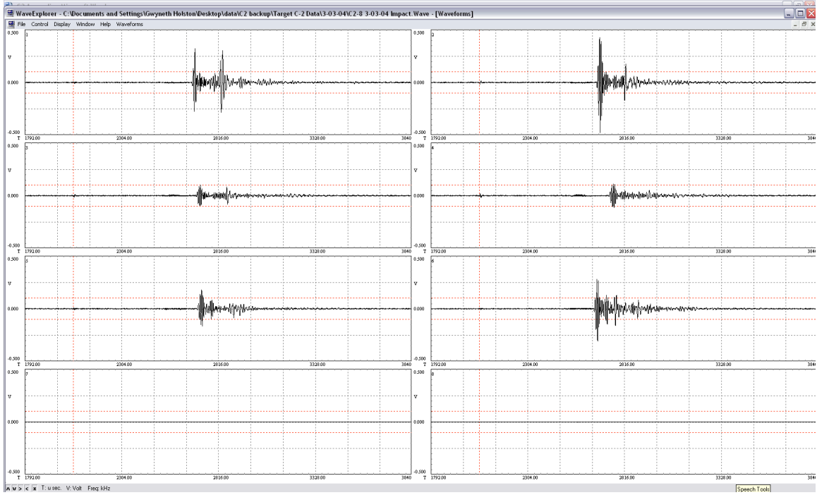
Figure 32: C-2 Shot #8 Impact Waveform
