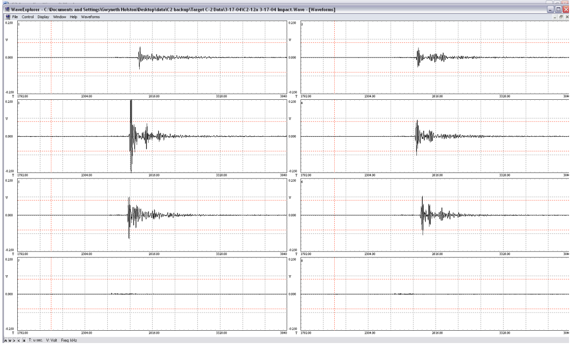
Figure 38: C-2 Shot #12a Impact Waveform
