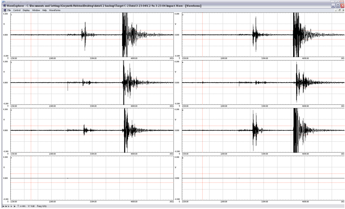
Figure 34: C-2 Shot #9a Impact Waveform
