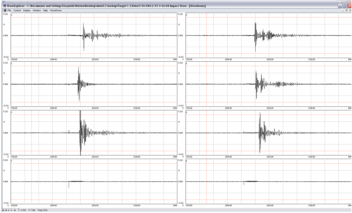
Figure 41: C-2 Shot #15 Impact Waveform
