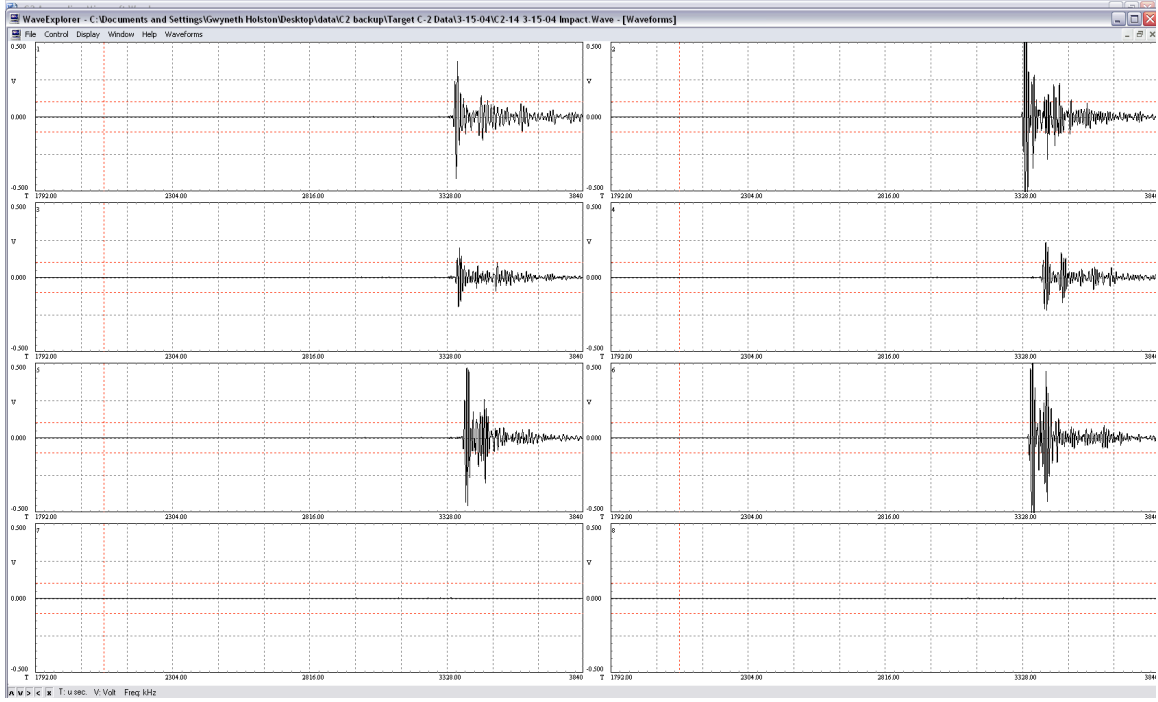
Figure 40: C-2 Shot #14 Impact Waveform
