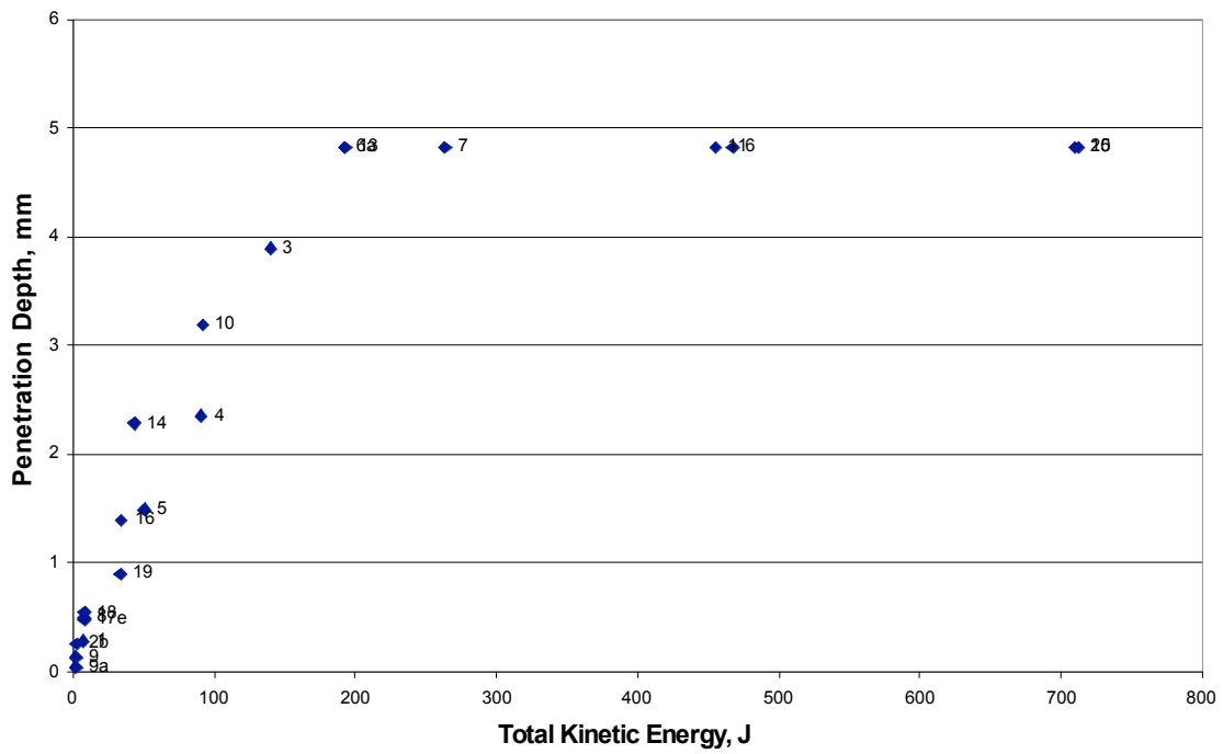
Figure 11: Penetration Depth vs. Total Kinetic Energy
