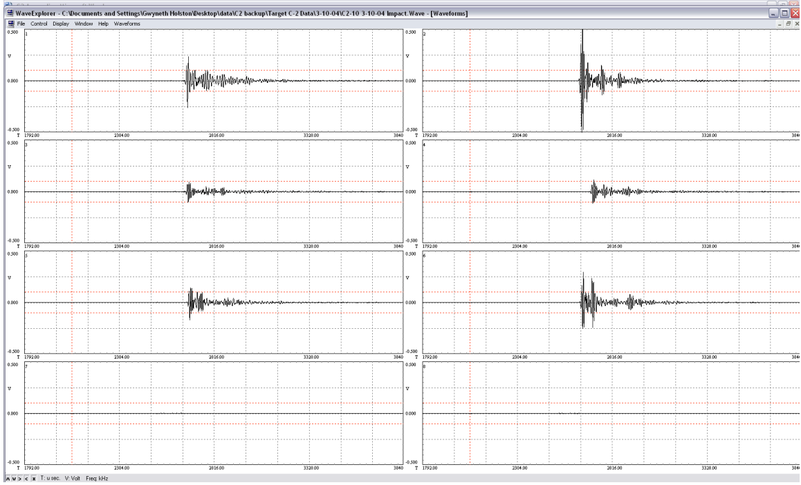
Figure 35: C-2 Shot #10 Impact Waveform
