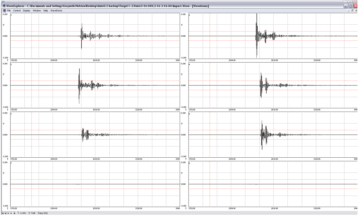
Figure 42: C-2 Shot #16 Impact Waveform
