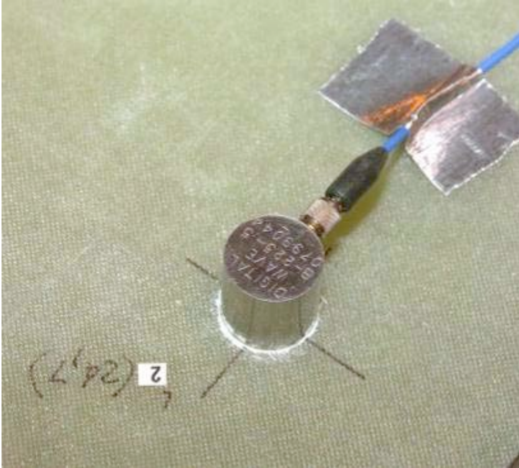
Figure 4: C-1 Detail of Sensor 2 No photo was available for sensors on C-2.
