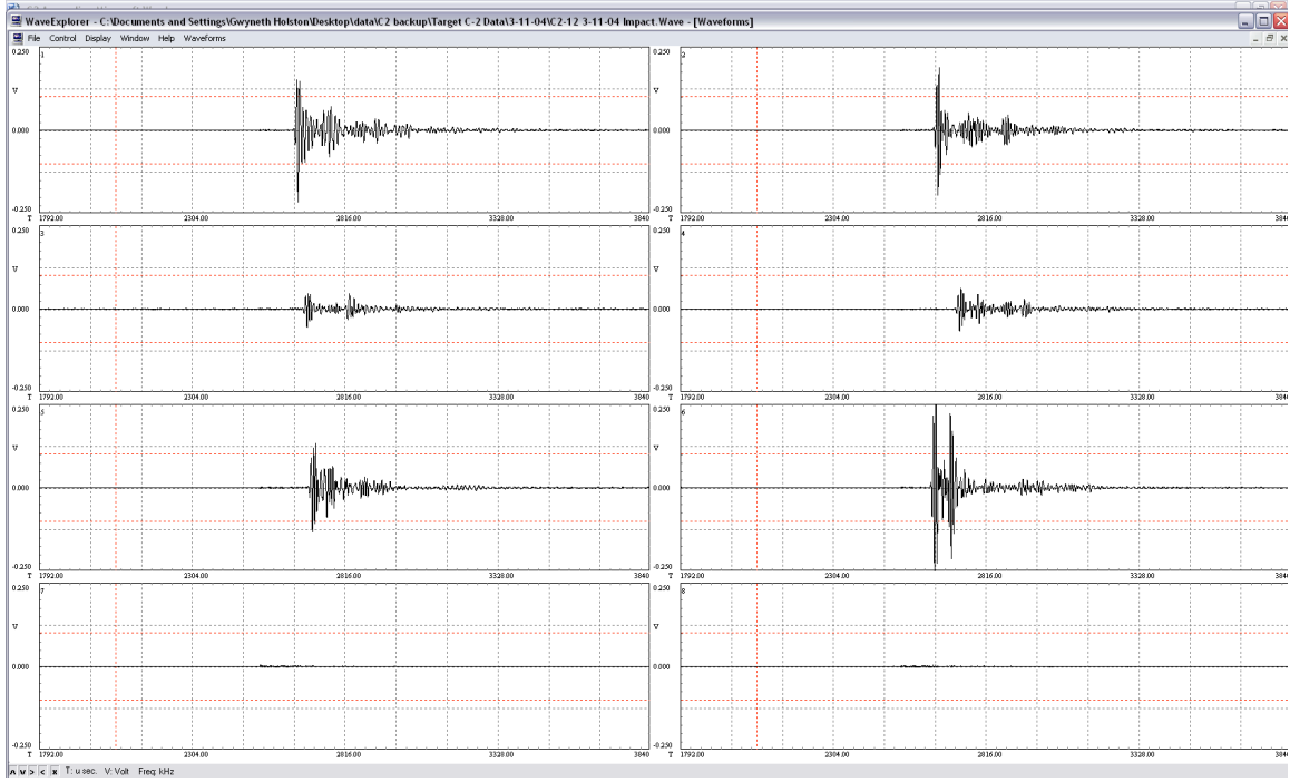
Figure 37: C-2 Shot #12 Impact Waveform
