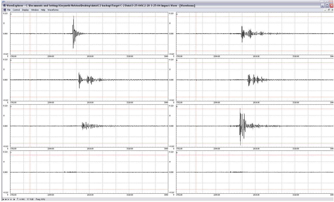
Figure 46: C-2 Shot #20 Impact Waveform
