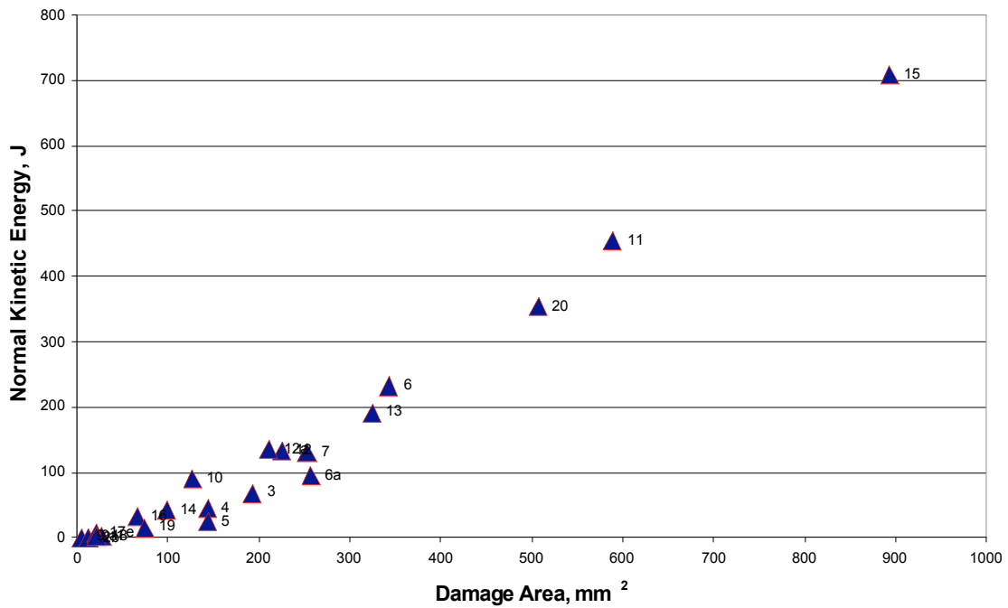
Figure 13: C-2 Normal Kinetic Energy vs. Fiber Damage Area
