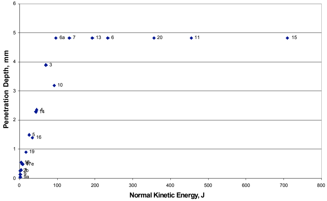
Figure 10: Penetration Depth vs. Normal Kinetic Energy
