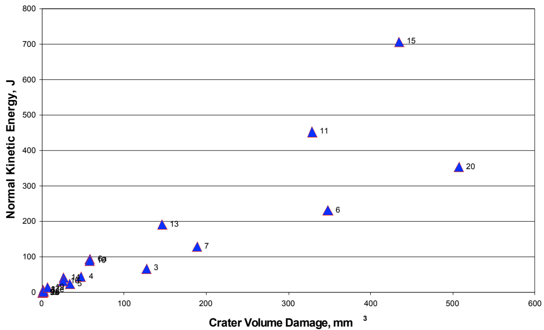
Figure 15: C-2 Normal Kinetic Energy vs. Crater Volume Damage
