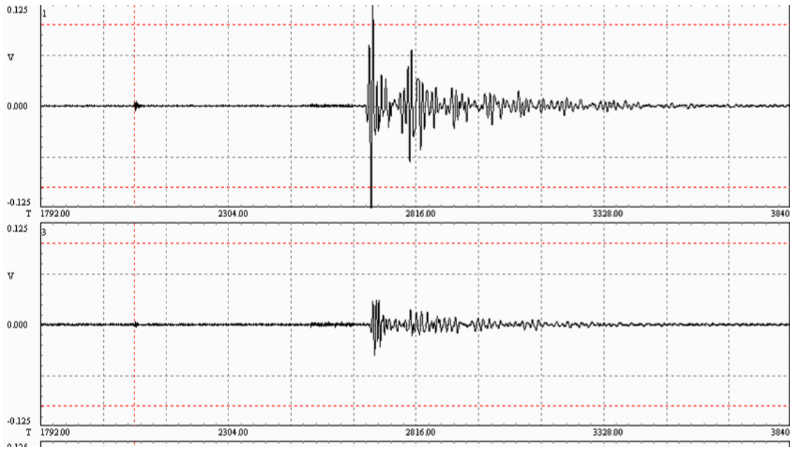
Figure 8: Detail of C-2 Impact Signal for Shot #3, Sensors 1 and 2
