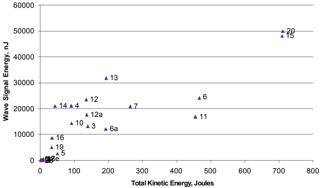
Figure 16: C-2 Wave Signal Energy vs. Total Kinetic Energy
