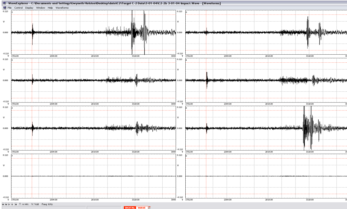
Figure 25: C-2 Shot #2b Impact Waveform
