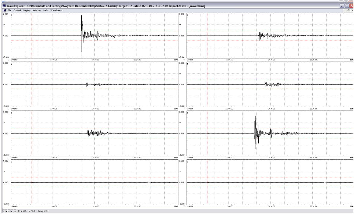
Figure 31: C-2 Shot #7 Impact Waveform
