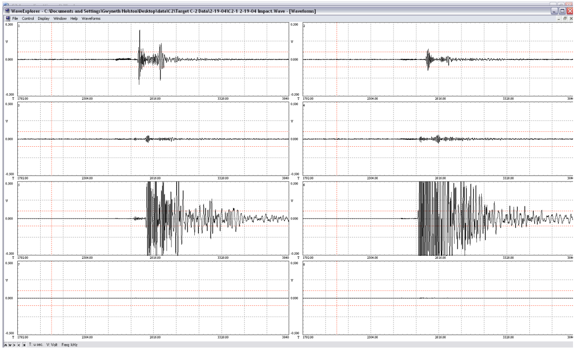
Figure 24: C-2 Shot #1 Impact Waveform
