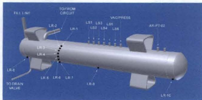
Figure 8. Lower reservoir
