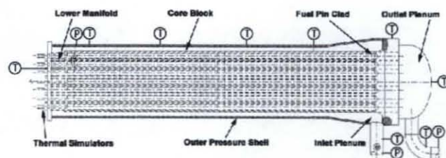
Figure 3. Core assembly
