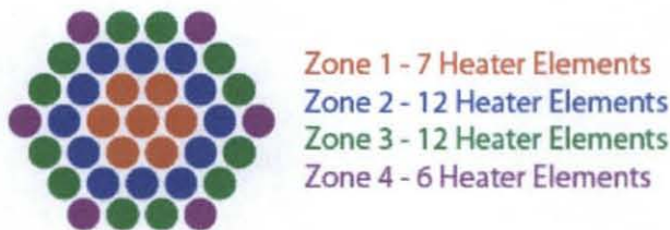
Figure 5. Power zones
