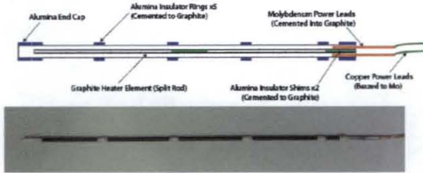
Figure 4. Thermal simulator
