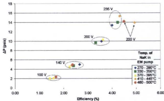
Figure 13. Pump efficiency
