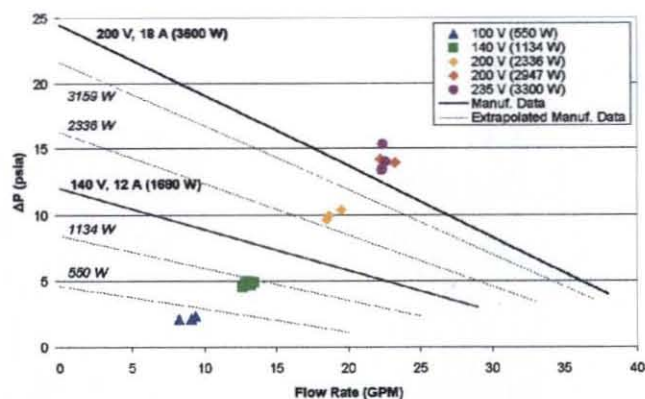
Figure 12. Pump performance data
