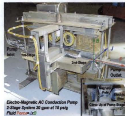
Figure 7. Electromagnetic pump
