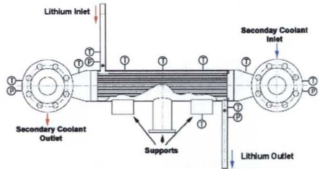
Figure 6. NaK/GN 2 heat exchanger
