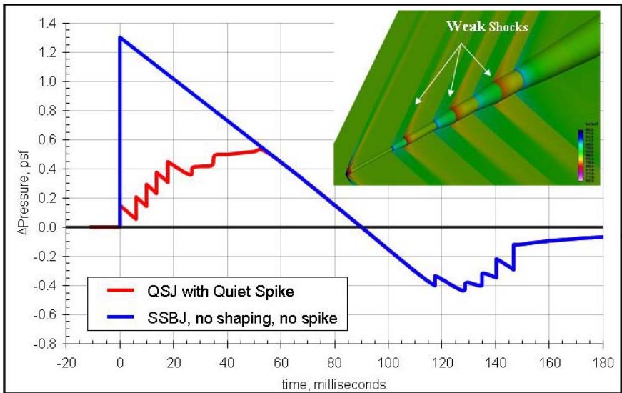
Figure 1. Quiet Spike shock wave “shaping” in near-field and ground signatures. (Note: QJSJ – Quiet Supersonic Jet, SSBJ – Supersonic Business Jet)
