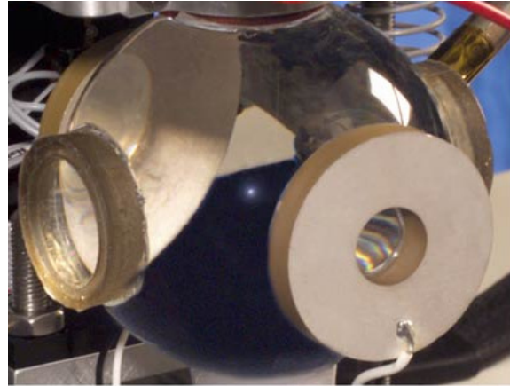
Figure 2.—Sonoluminescence flight hardware testing in 2003.
