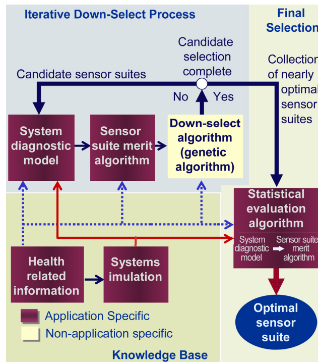
Fig. 3 Proposed diagnostic sensor selection architecture.
