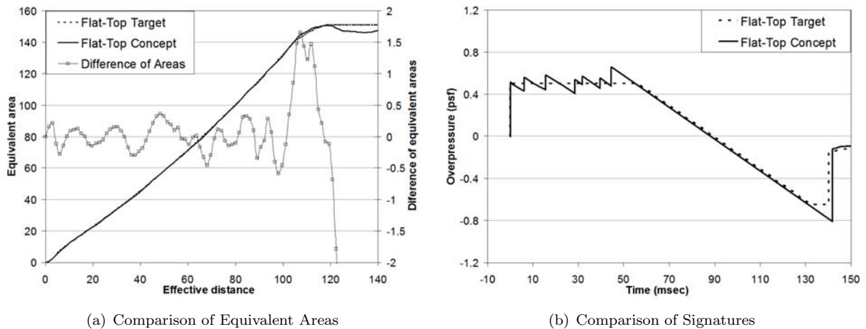
Figure 16. Ground signature and area distribution of a flattop supersonic concept.
