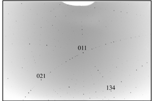
Fig. 2. A partially indexed Laue pattern of sample C2067,1,111,4 obtained by a 120 min. Laue exposure with a ring operation of 2.5 GeV at PF, KEK.
