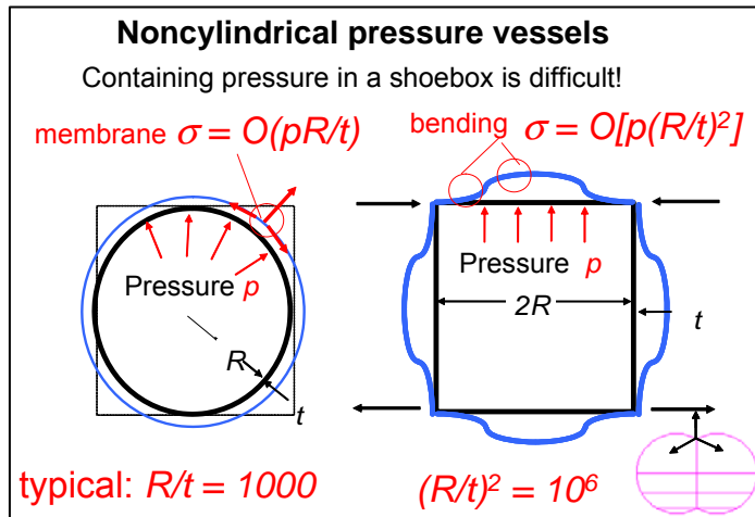
Figure 4. High bending stress associated with a noncylindrical pressure vessel.
