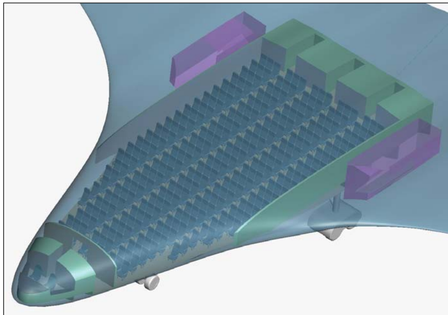
Figure 5. Sample 335-passenger layout for volumetric sanity check.
