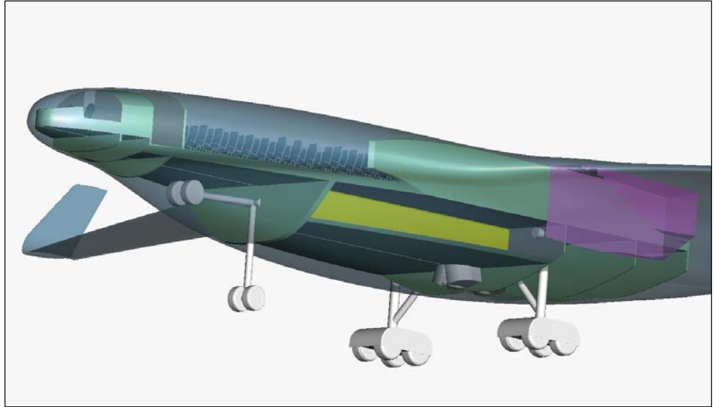
Figure 6. Landing gear retraction geometry.
