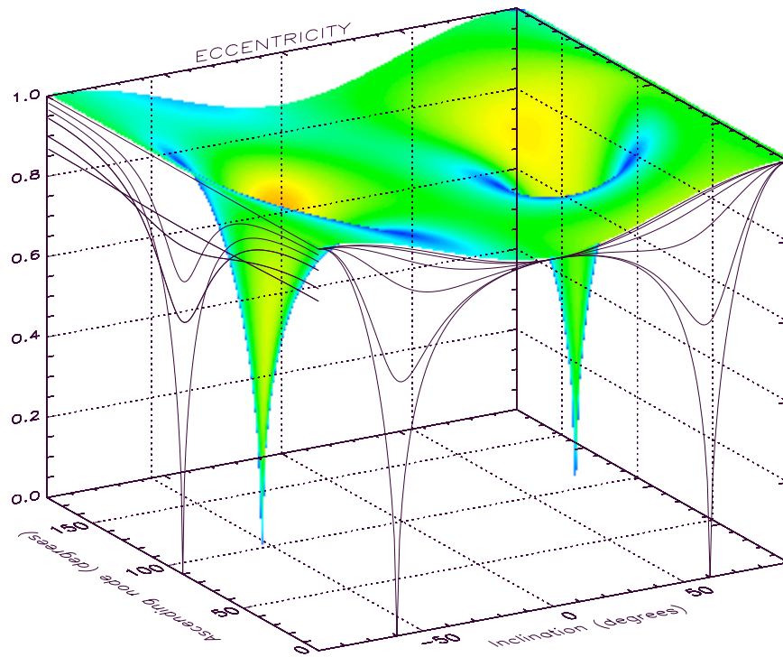
Figure 2: Eccentricity as function of the inclination and the longitude of the ascending node
