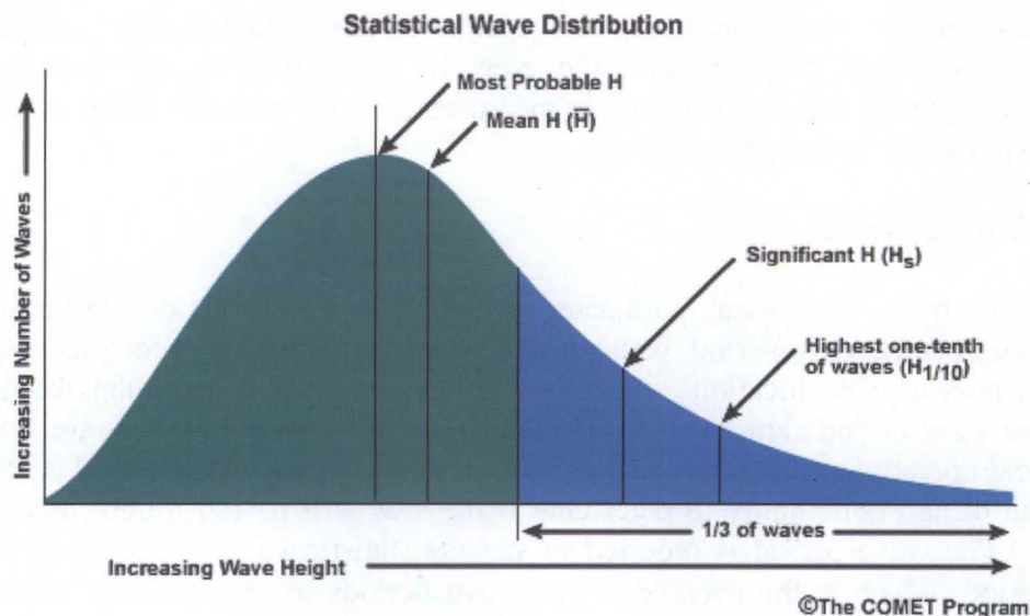
Figure 1: Rayleigh distribution of wave heights annotated with the relationships of H_{mean} , H_s , and H_{1/10} ( http://www.meted.ucar.edu/marine/mod1_wv_type_char/frame.htm )
