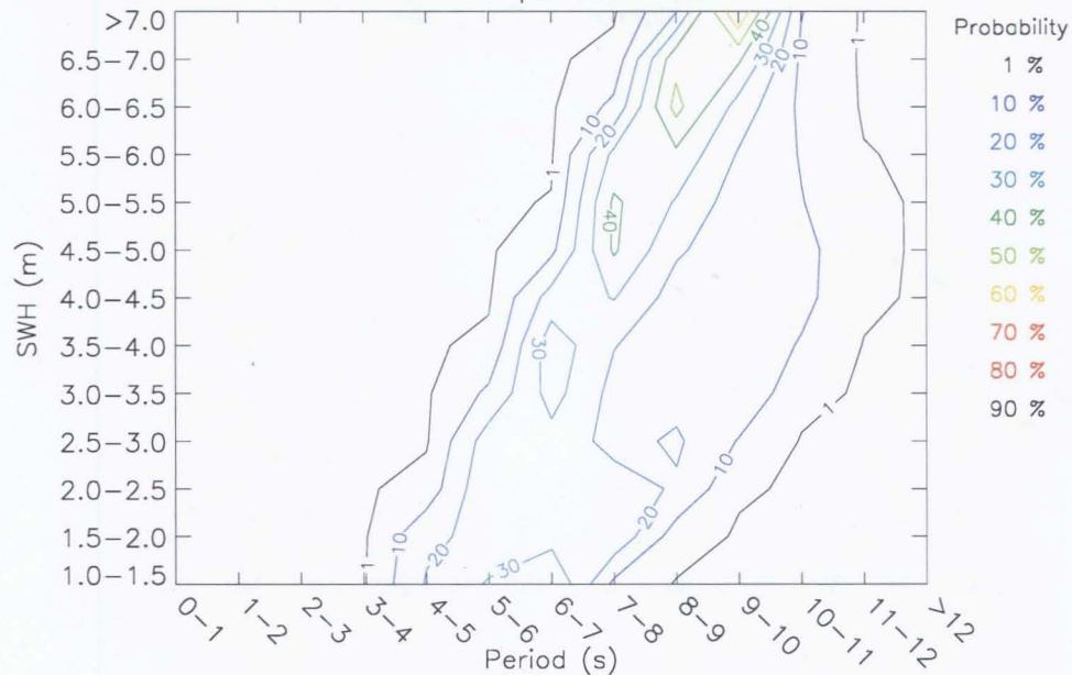
1971–2001 Conditional Probability of Specified Wave Period With a Given SWH Ship_Three
