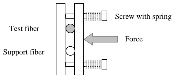
Figure 4: Schematic representation of a pressurized fiber Bragg grating. A copper plate with four screws holds the test fiber and the support fiber onto the cold plate of the cryogenic chamber. Four springs apply a diametric load to the test fiber to form a PFBG.
