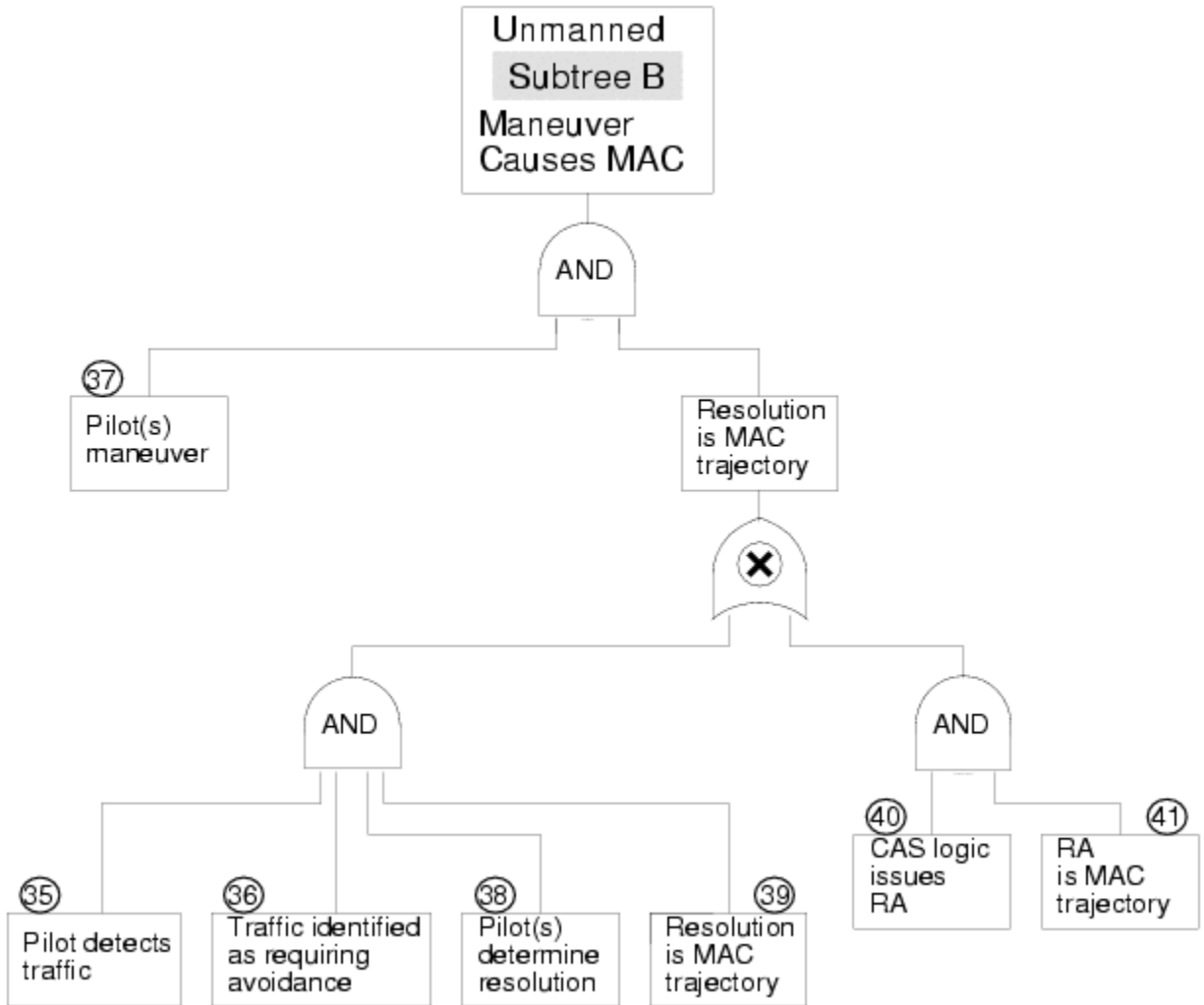
Figure 2.7. Subtree B for Unmanned Aircraft.
